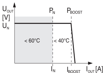
Figure 13 Output characteristic curve
