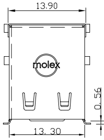
PANEL CUT-OUT DIMENSIONS
