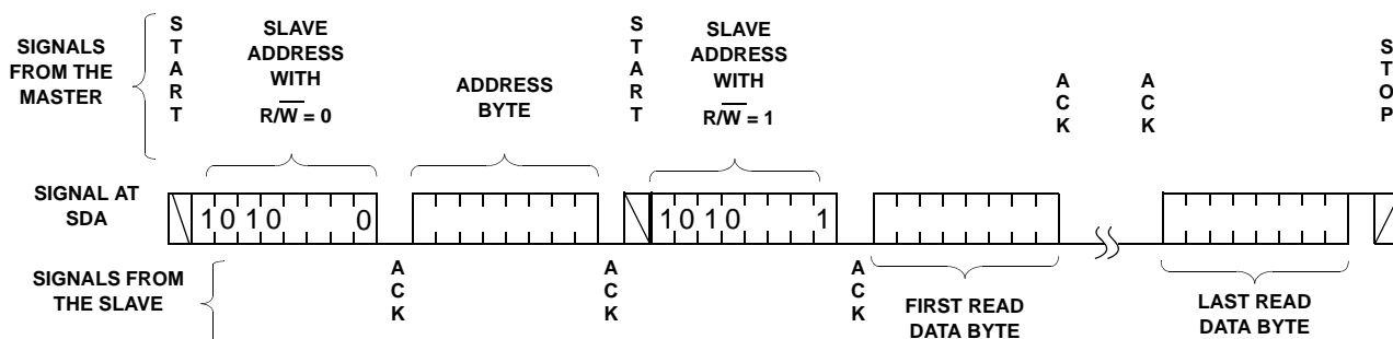
FIGURE 18. READ SEQUENCE
