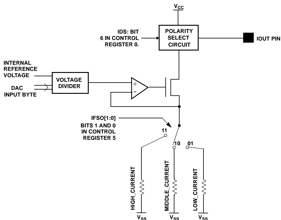
FIGURE 5. D/A CONVERTER BLOCK DIAGRAM
