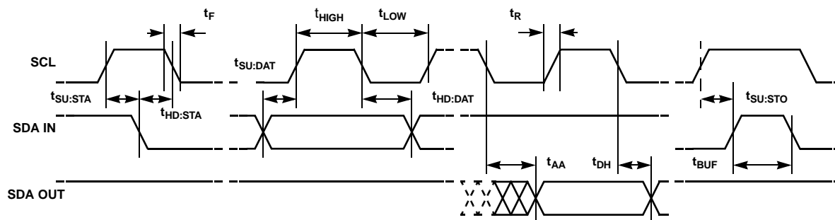
FIGURE 1. BUS TIMING
