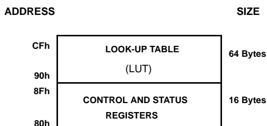
FIGURE 12. X96011 MEMORY MAP
