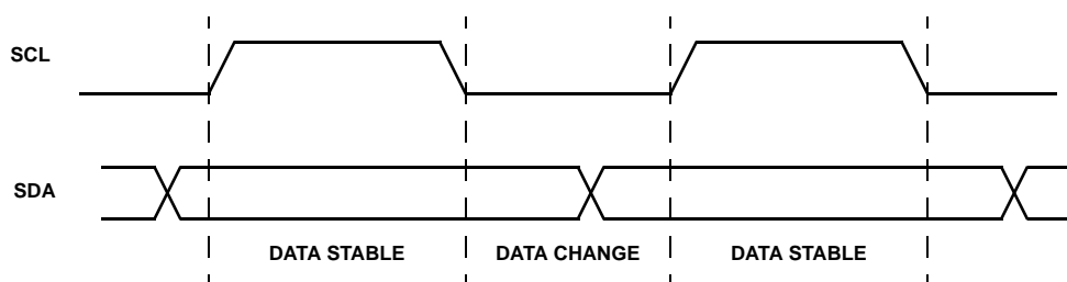
FIGURE 10. VALID DATA CHANGES ON THE BUS
