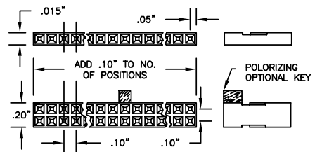
FIG. 3 HOUSING SIZES: WHEN ORDERING LEAD ASSEMBLY, SPECIFY NO. OF POSITIONS. IF SINGLE ROW, 2 THRU 36; DOUBLE ROW, 2 X 2 THRU 2 X 36 (Polarizing Key Available on Request).
