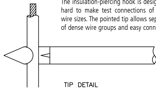
TIP DETAIL
