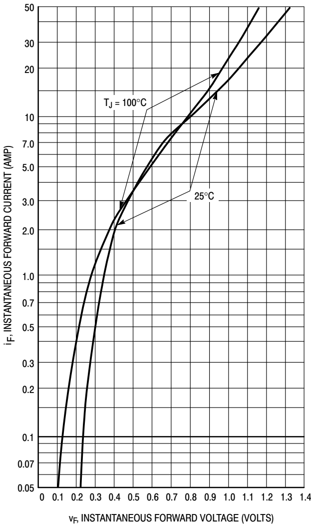
Figure 7. Typical Forward Voltage
