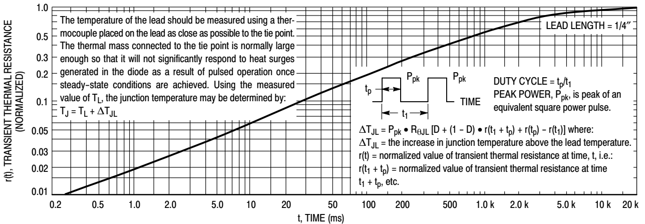
Figure 5. Thermal Response
