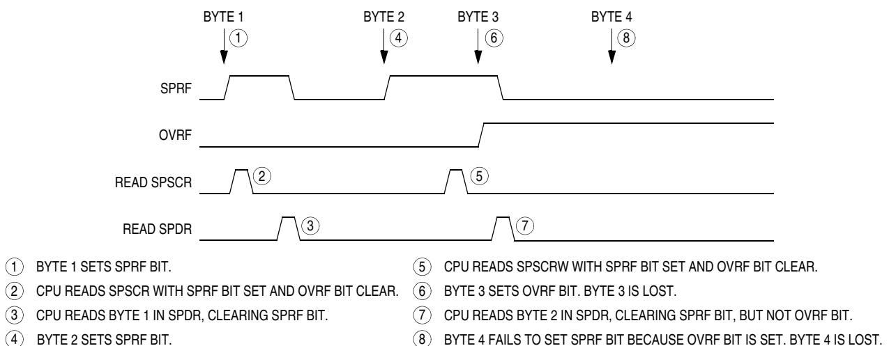
Figure 15-7. Missed Read of Overflow Condition
