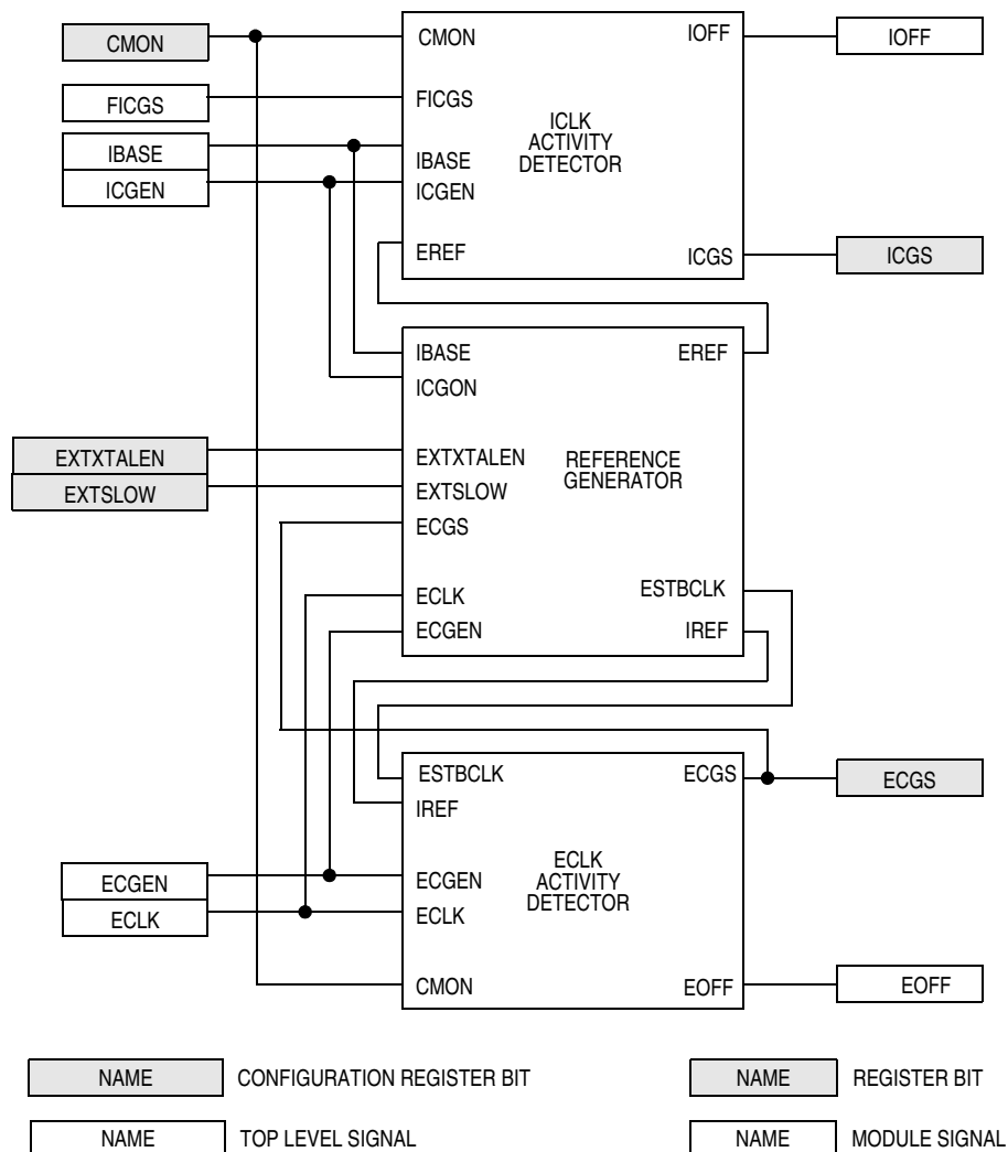
Figure 8-5. Clock Monitor Block Diagram
