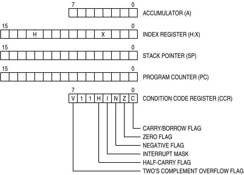
Figure 7-1. CPU Registers
