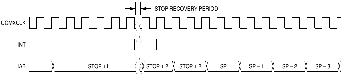
Figure 14-15. Stop Mode Recovery from Interrupt
