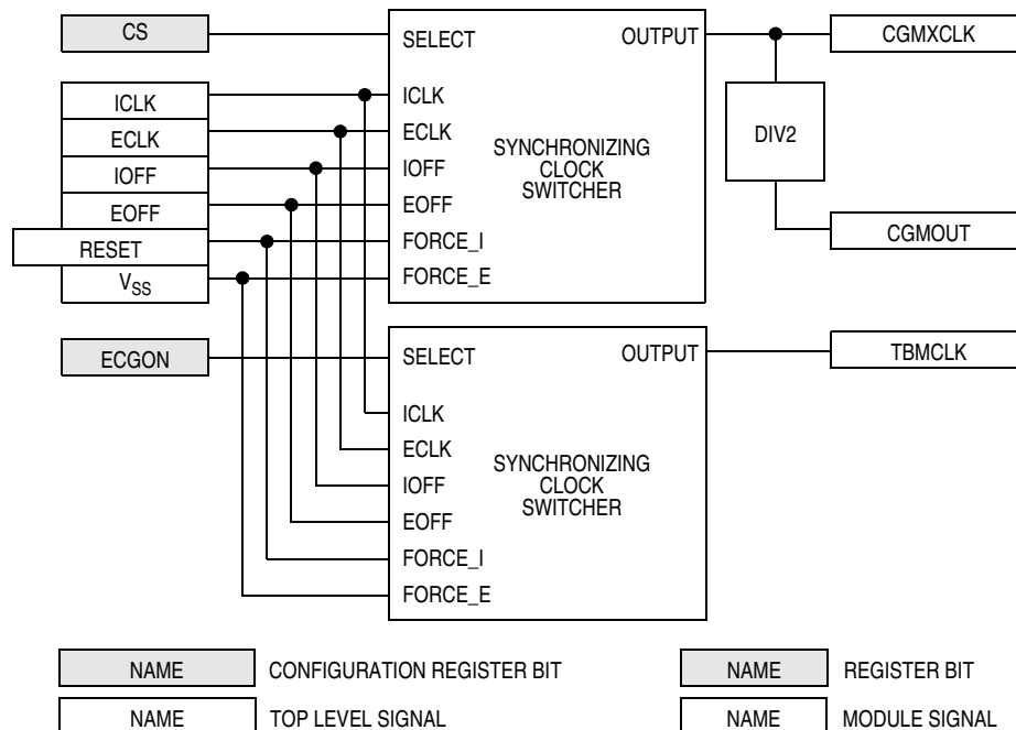
Figure 8-8. Clock Selection Circuit Block Diagram
