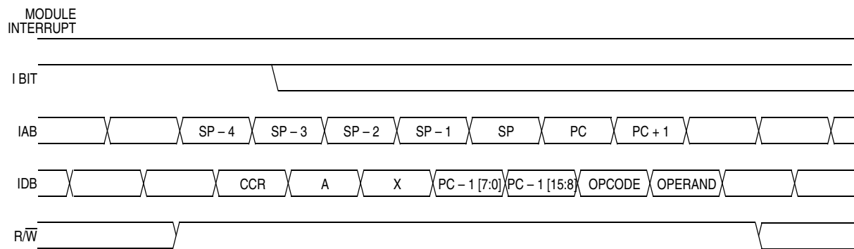
Figure 14-8. Interrupt Recovery
