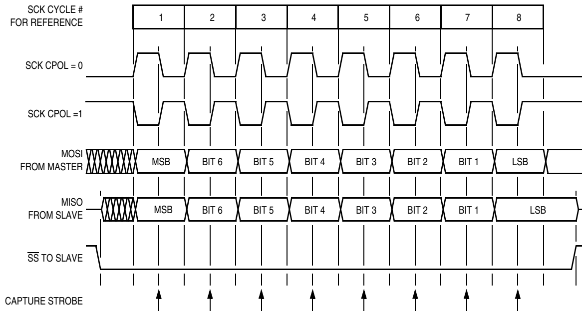
Figure 15-5. Transmission Format (CPHA = 1)
