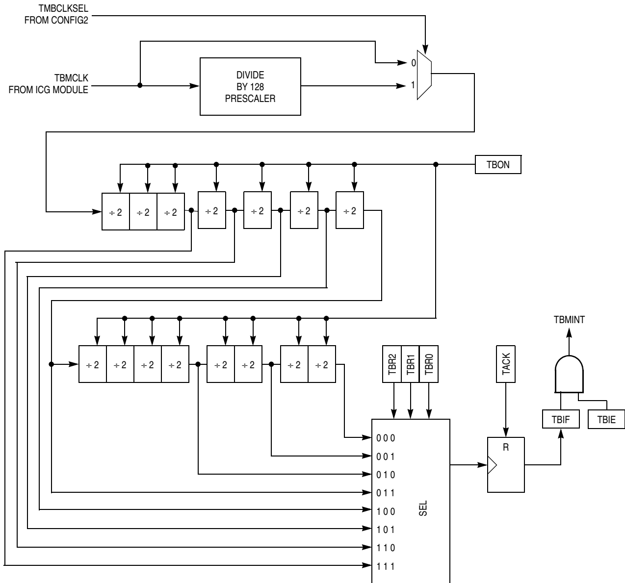
Figure 16-1. Timebase Block Diagram
