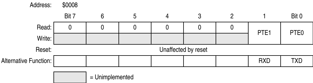
Figure 12-13. Port E Data Register (PTE)
