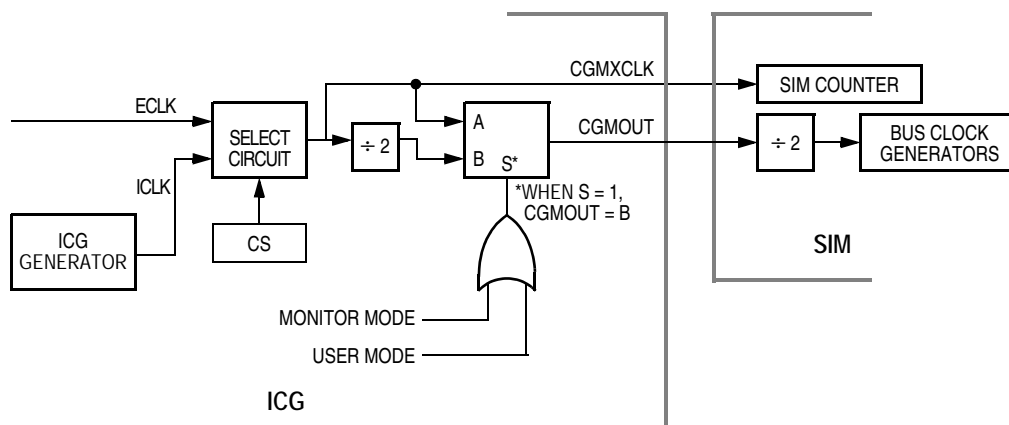
Figure 14-2. System Clock Signals
