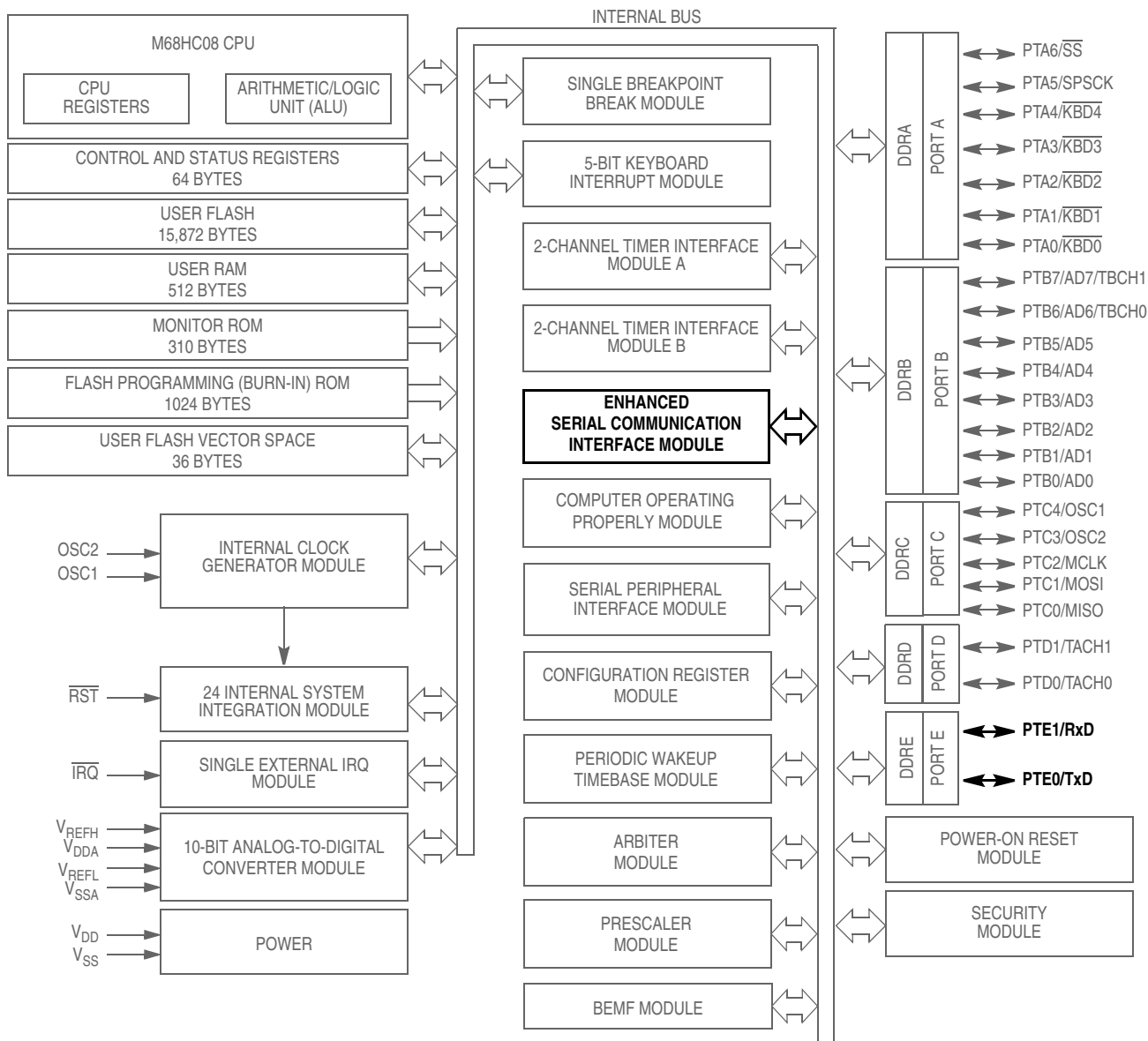
Figure 13-1. Block Diagram Highlighting ESCI Block and Pins
