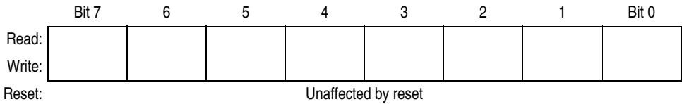
Figure 7-2. Accumulator (A)
