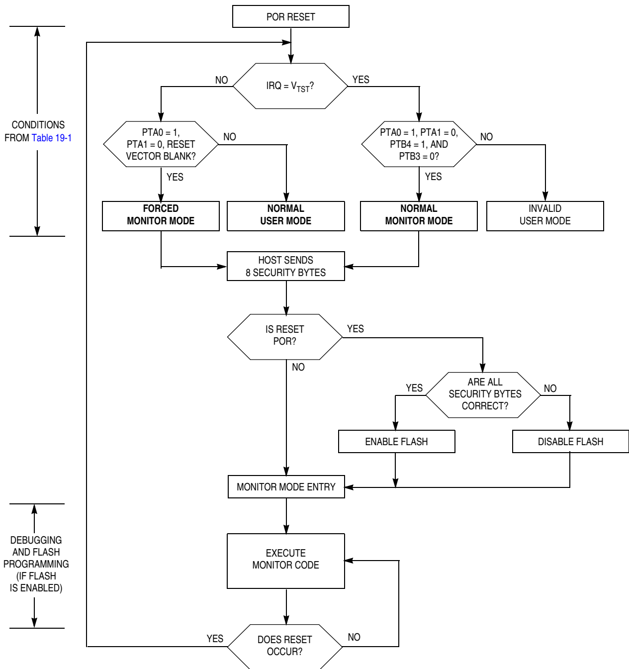
Figure 19-8. Simplified Monitor Mode Entry Flowchart
