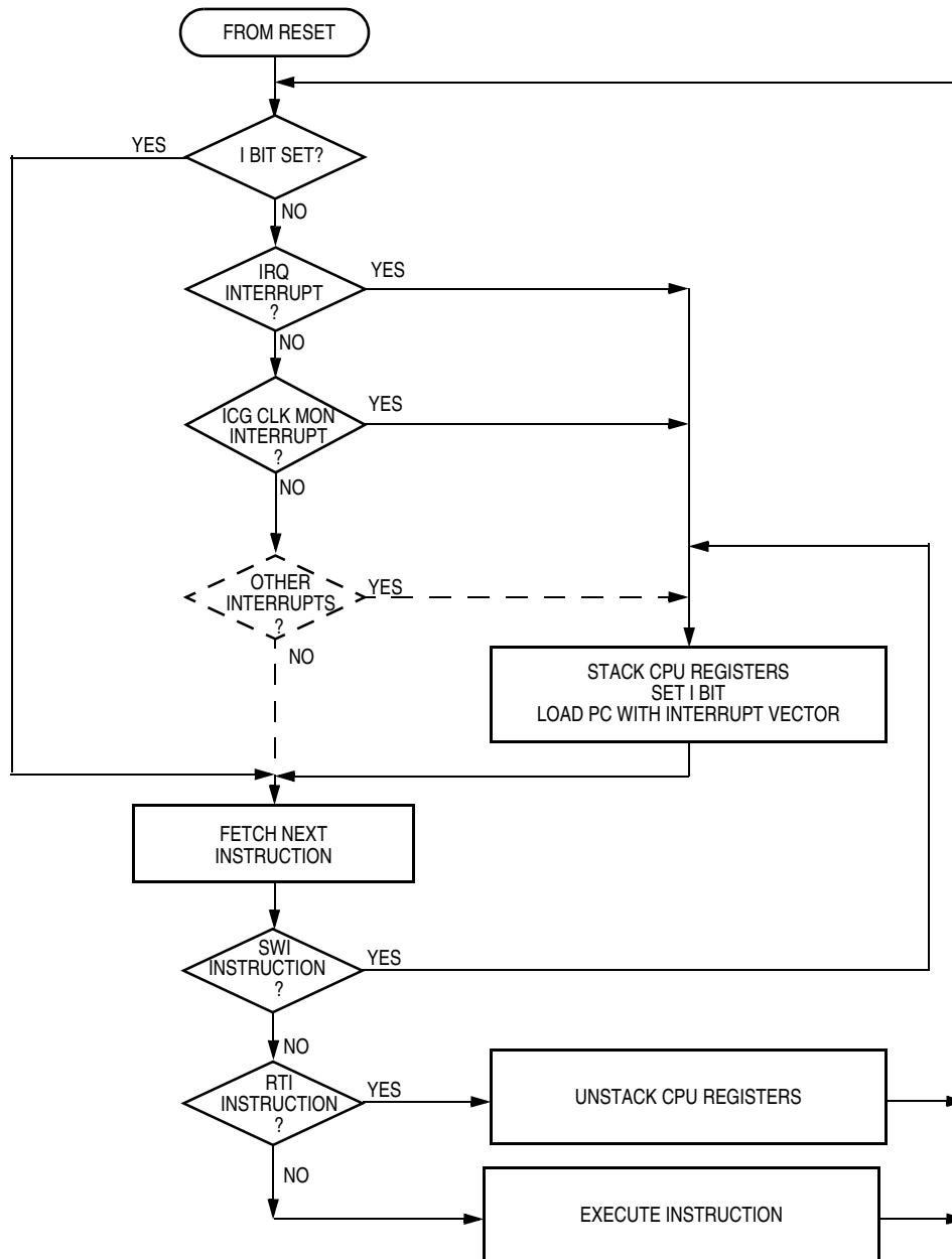
Figure 14-9. Interrupt Processing
