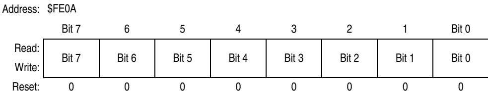
Figure 19-5. Break Address Register Low (BRKL)
