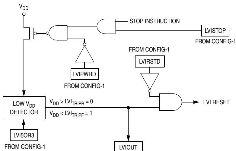
Figure 11-1. LVI Module Block Diagram
