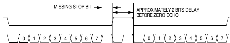
Figure 19-13. Break Transaction
