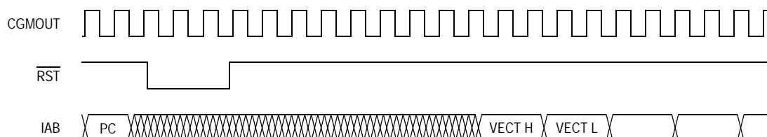
Figure 14-3. External Reset Timing
