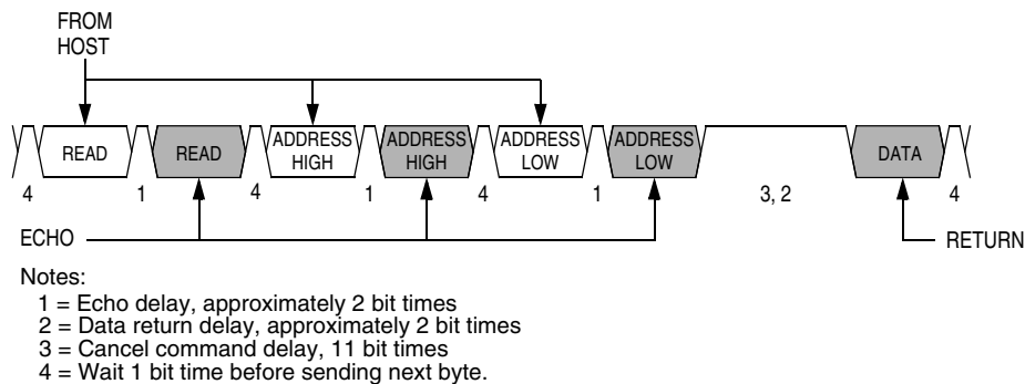
Figure 19-14. Read Transaction
