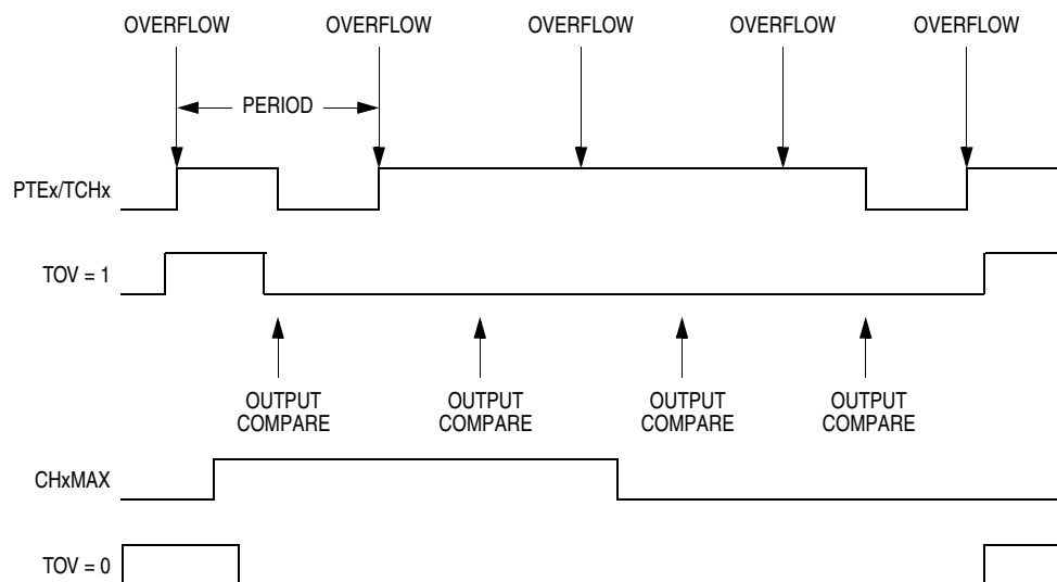
Figure 18-8. CHxMAX Latency
