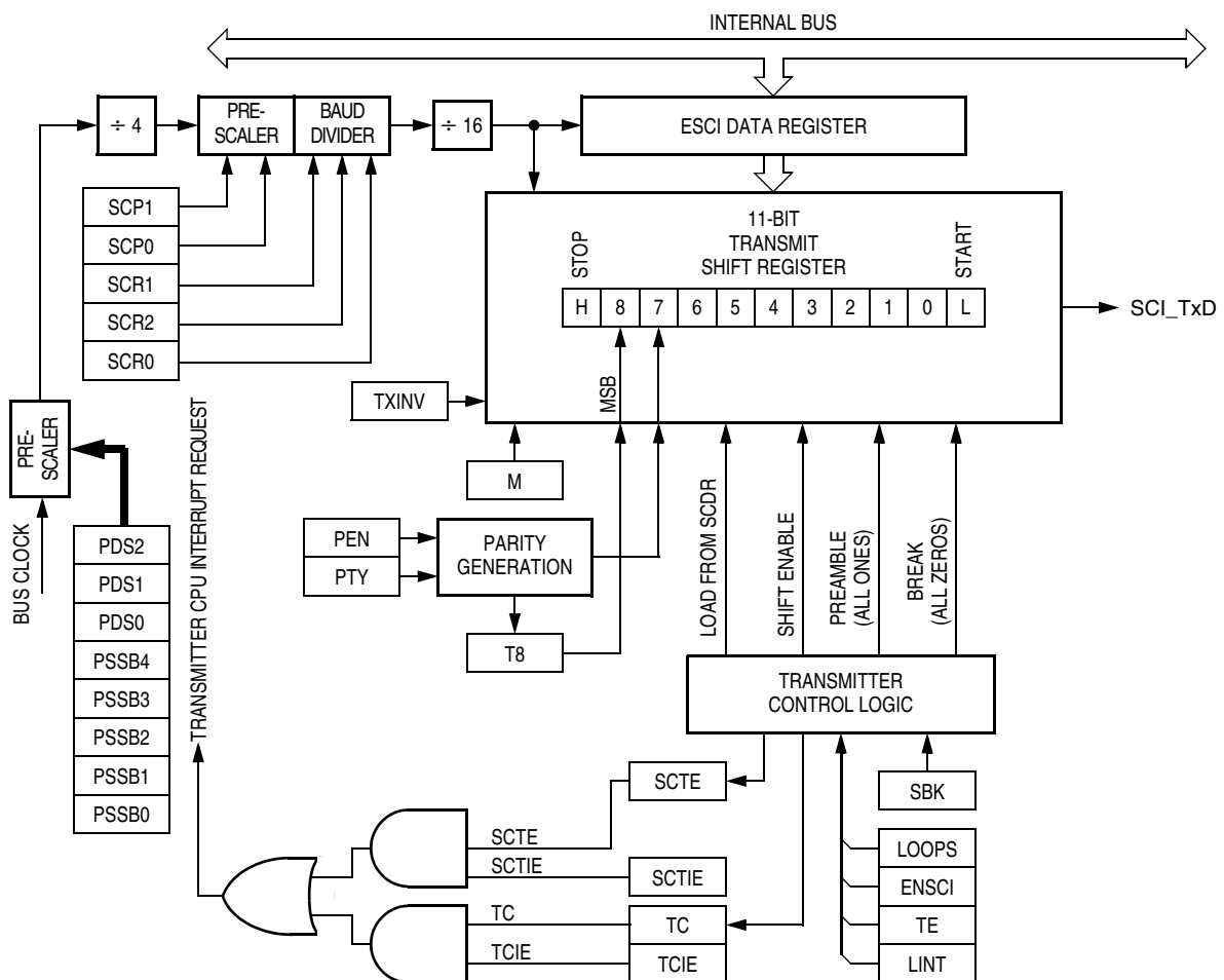
Figure 13-4. ESCI Transmitter
