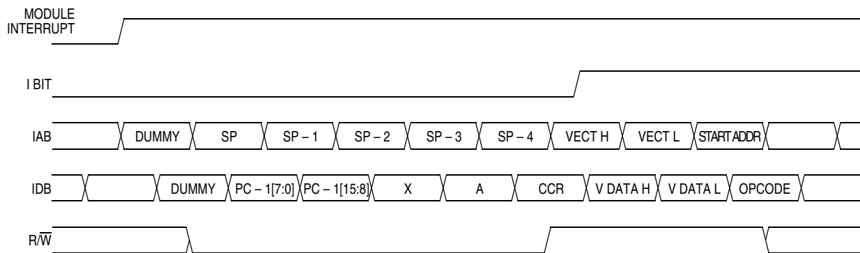
Figure 14-7. Interrupt Entry
