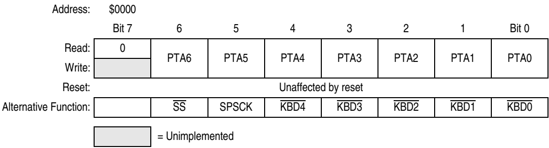
Figure 12-1. Port A Data Register (PTA)
