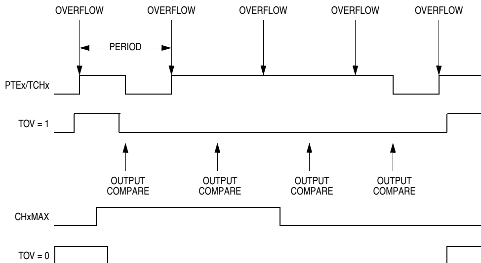
Figure 17-8. CHxMAX Latency
