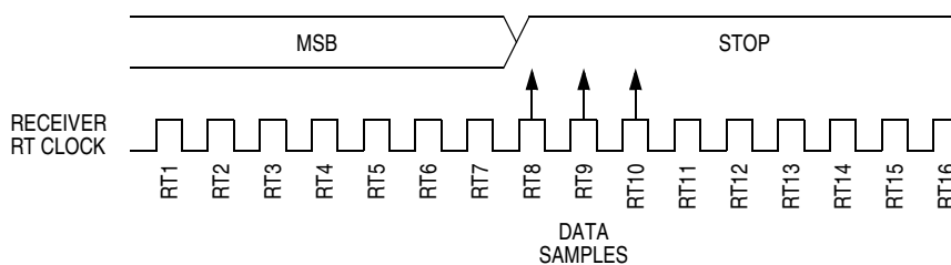
Figure 13-7. Slow Data
