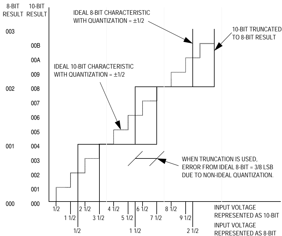
Figure 3-3. 8-Bit Truncation Mode Error
