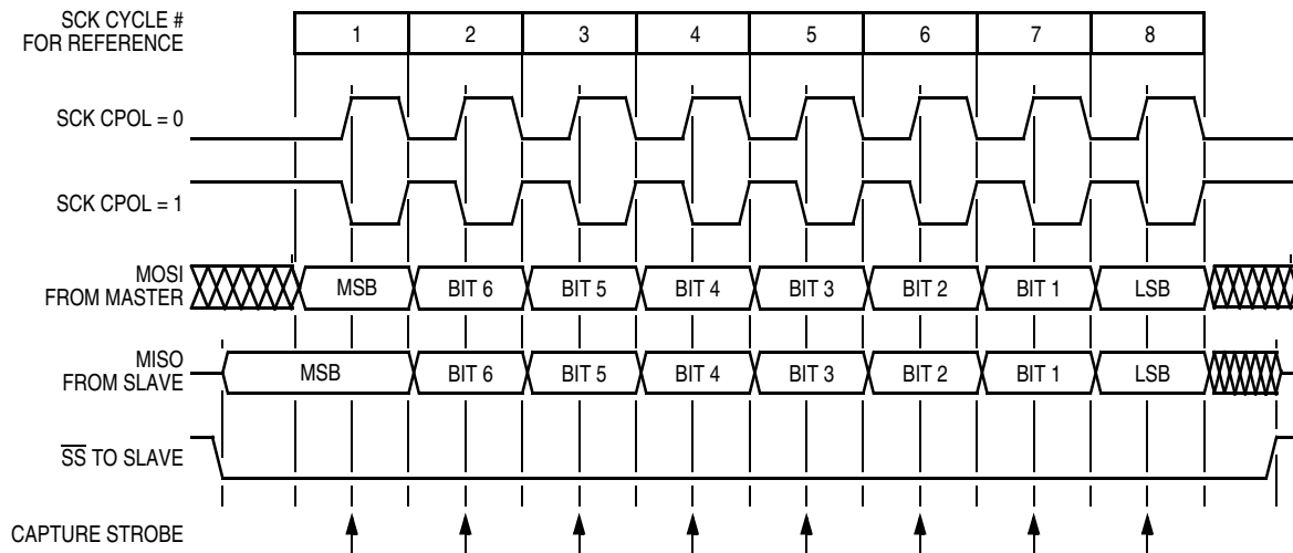
Figure 15-4. Transmission Format (CPHA = 0)
