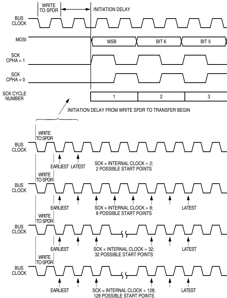
Figure 15-6. Transmission Start Delay (Master)
