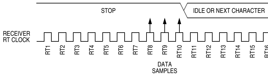
Figure 13-8. Fast Data
