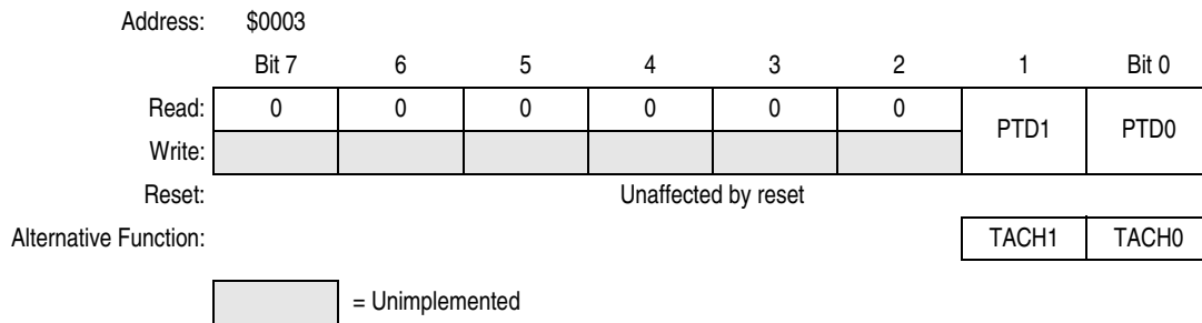
Figure 12-10. Port D Data Register (PTD)
