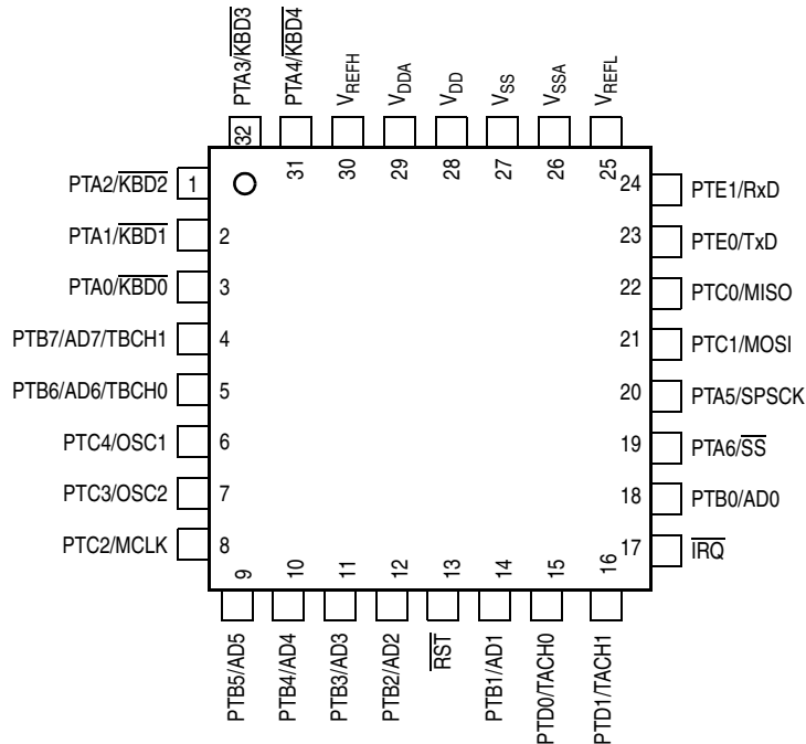
Figure 1-2. Pin Assignments
