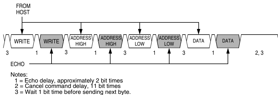
Figure 19-15. Write Transaction
