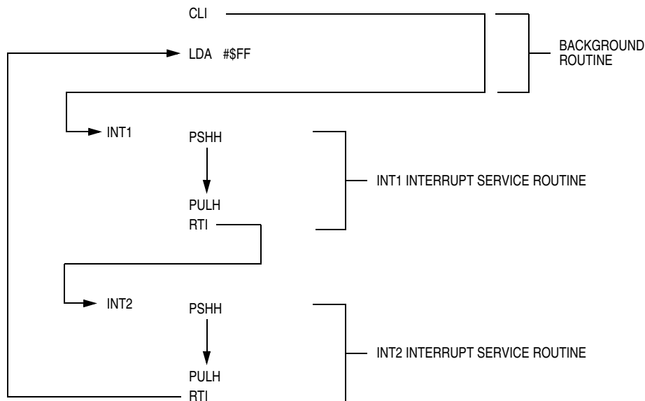
Figure 14-10. Interrupt Recognition Example
