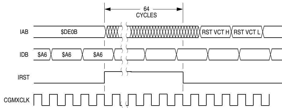
Figure 14-13. Wait Recovery from Internal Reset
