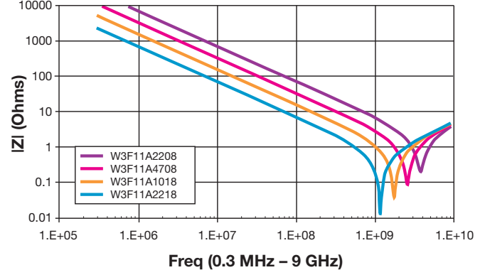
IMPEDANCE 1206 – 100V
