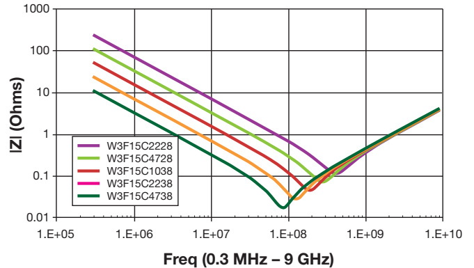
IMPEDANCE 1206 – 50V
