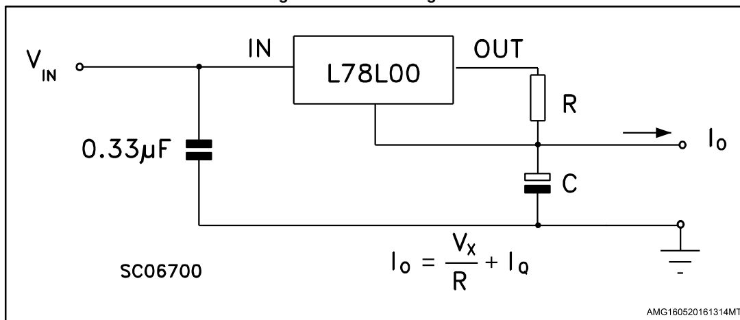
Figure 15: Current regulator
