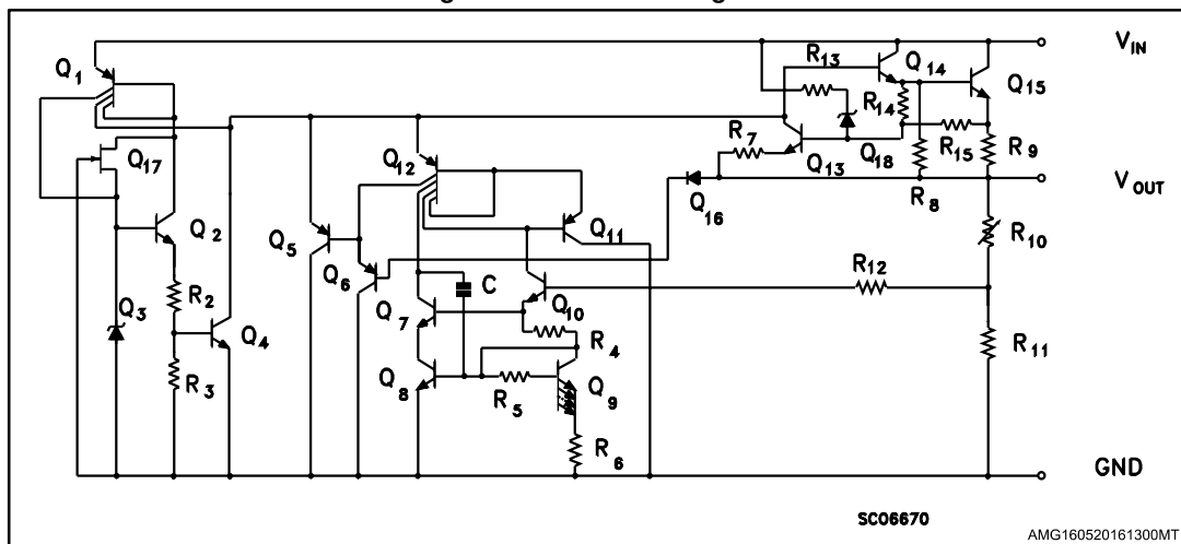
Figure 1: Schematic diagram
