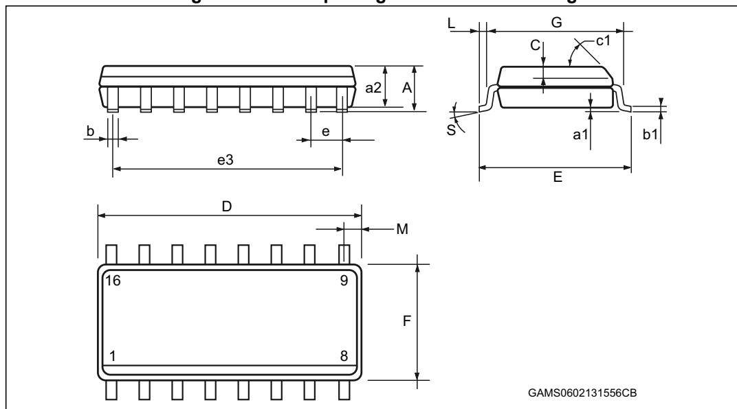
Figure 11. SO-16 package mechanical drawing
