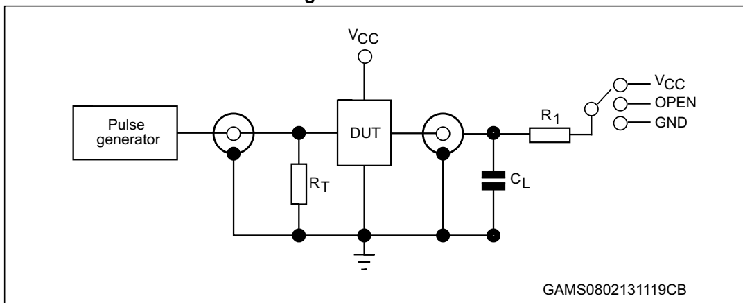
Figure 7. Test circuit
