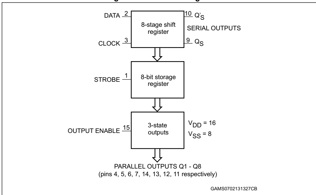
Figure 3. Functional diagram
