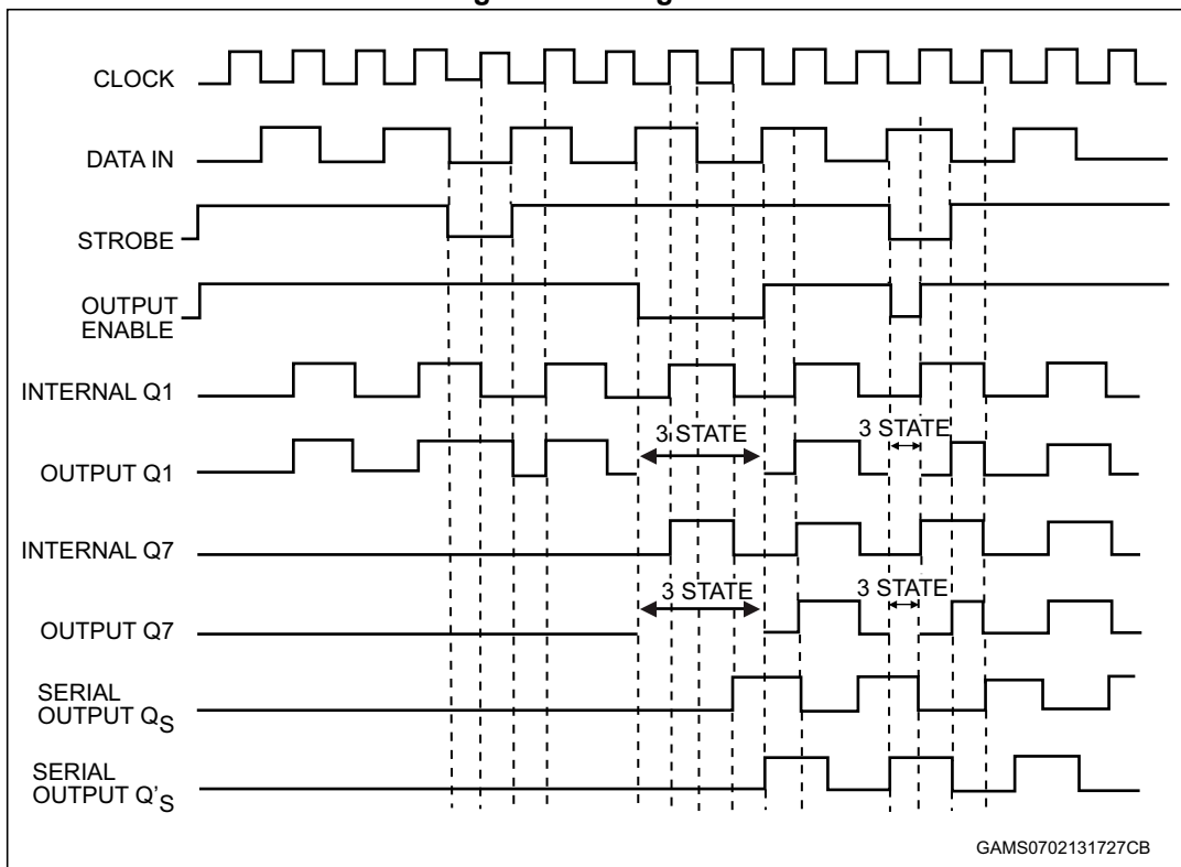
Figure 5. Timing chart
