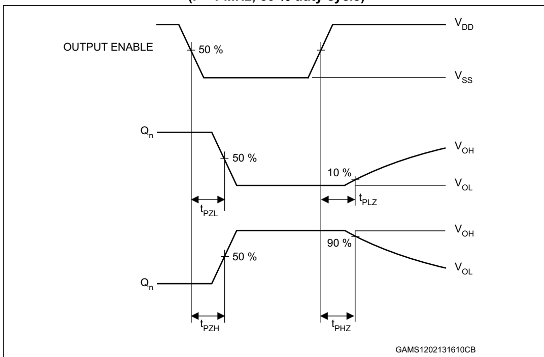
Figure 10. Waveform 3: Setup and hold time (PI to P/S) (f = 1 MHz; 50 % duty cycle)
