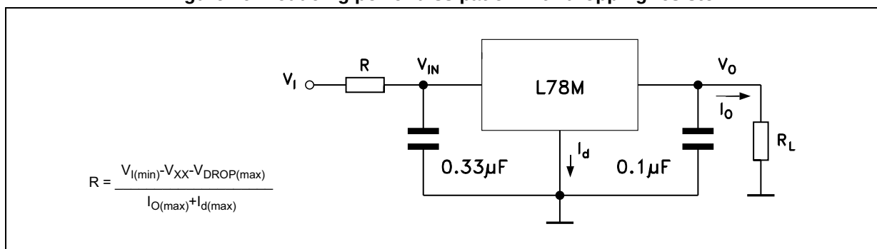
Figure 26. Reducing power dissipation with dropping resistor
