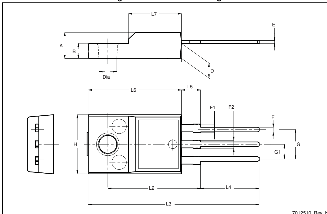
Figure 31. TO-220FP drawing
