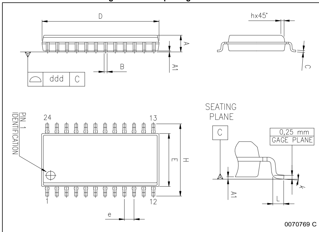
Figure 42. SO24 package outline
