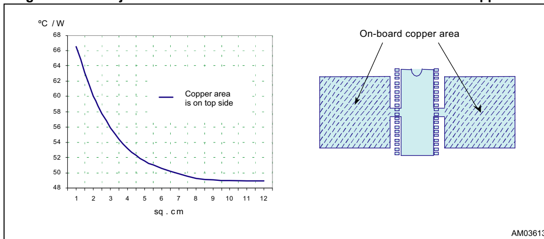
Figure 32. SO24 junction ambient thermal resistance versus on-board copper area
