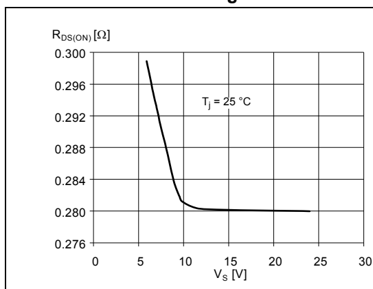
Figure 38. Typical low-side R_{DS(ON)} vs. supply voltage
