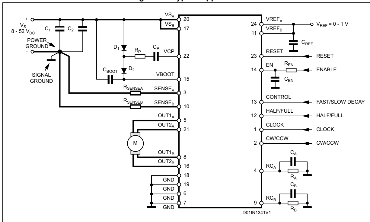
Figure 25. Typical application
