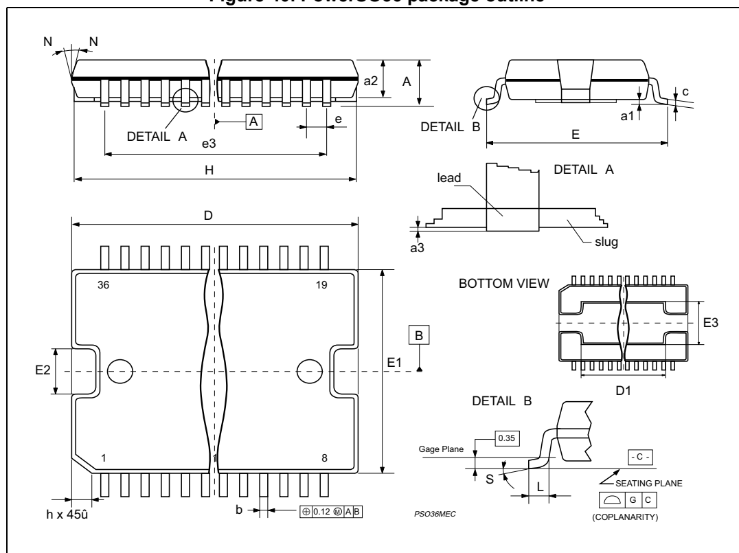
Figure 40. PowerSO36 package outline
