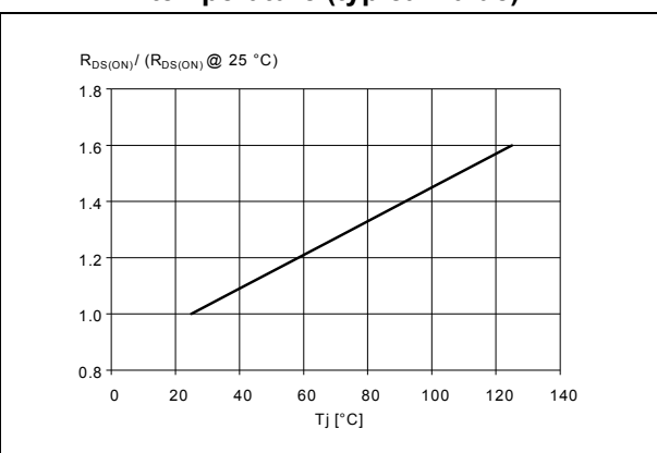
Figure 37. Normalized R_{DS(ON)} vs. junction temperature (typical value)
