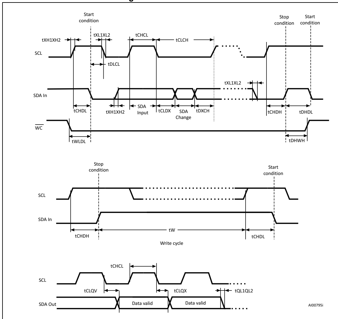
Figure 11. AC waveforms
