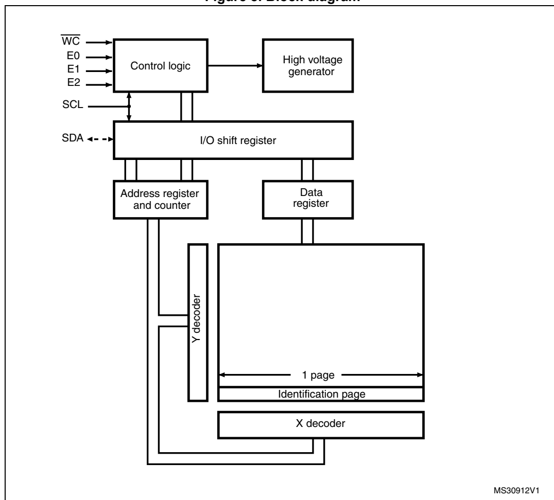
Figure 8. Block diagram
