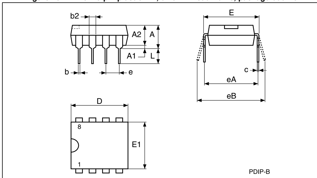
Figure 23. PDIP8 – 8-pin plastic DIP, 0.25 mm lead frame, package outline
