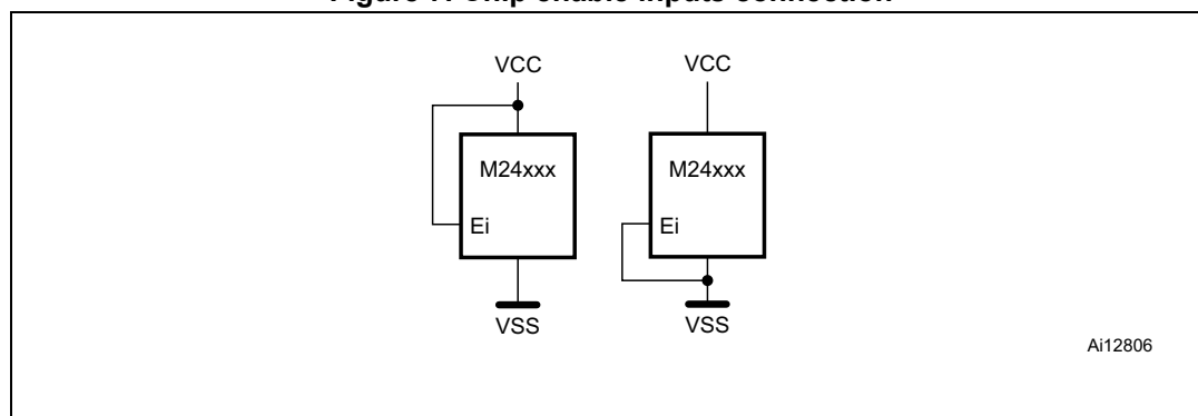
Figure 7. Chip enable inputs connection
