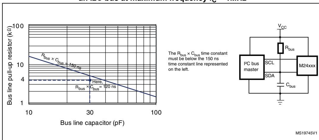
Figure 16. Maximum R_{bus} value versus bus parasitic capacitance ( C_{bus} ) for an I2C bus at maximum frequency f_C = 1 MHz
