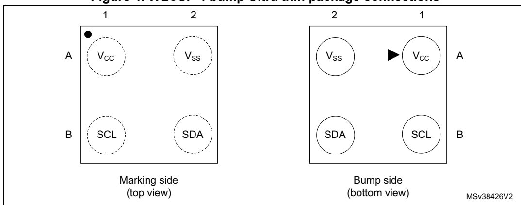
Figure 4. WLCSP 4 bump Ultra thin package connections
