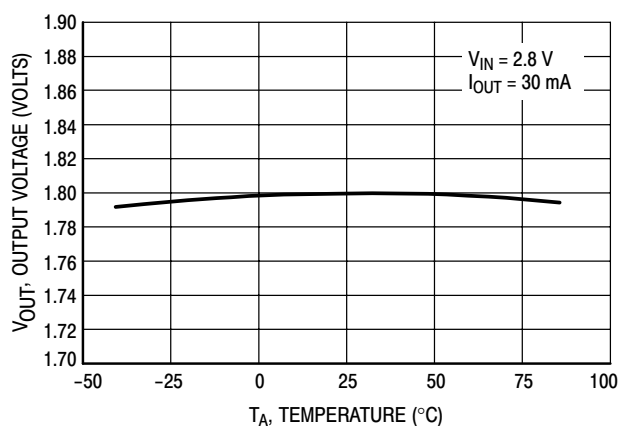
Figure 17. MPC78PC18 Output Voltage versus Temperature
