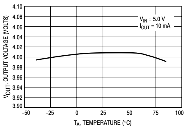
Figure 19. MC78PC40 (4.0 V) Output Voltage versus Temperature
