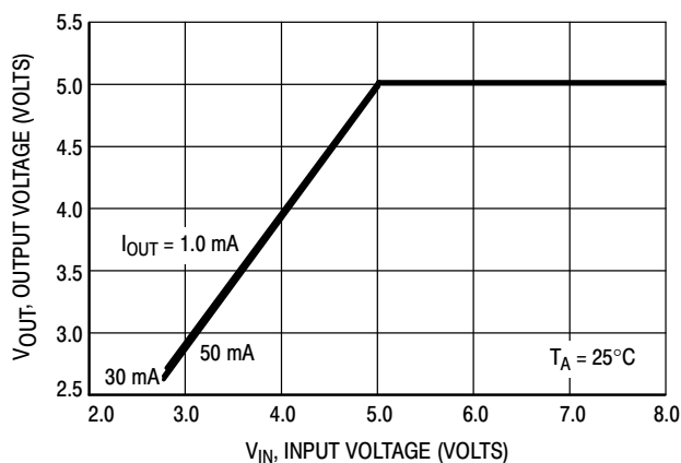
Figure 12. MC78PC50 Output Voltage versus Input Voltage
