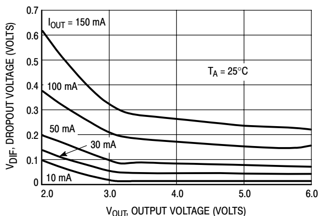
Figure 28. Dropout Voltage versus Output Voltage
