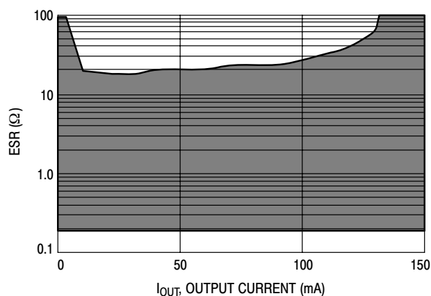
Figure 49. Ceramic Capacitor 6.8 \mu F
