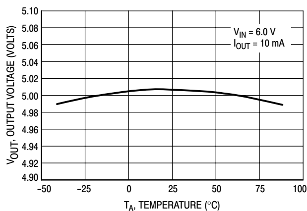
Figure 20. MC78PC50 Output Voltage versus Temperature
