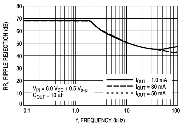
Figure 36. MC78PC50 Ripple Rejection versus Frequency
