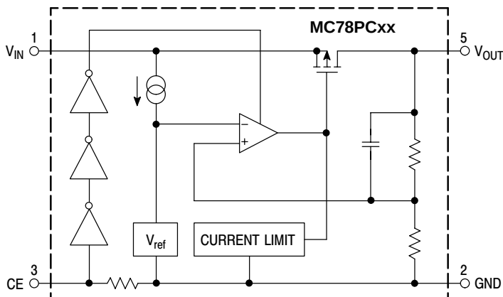
Block Diagram
