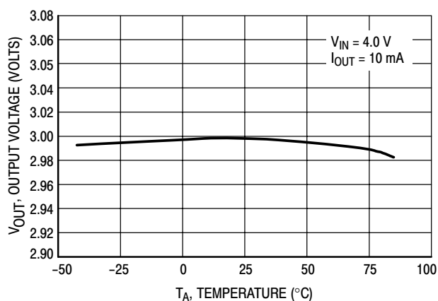
Figure 18. MC78PC30 Output Voltage versus Temperature
