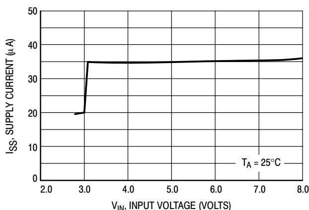
Figure 22. MC78PC30 Supply Current versus Input Voltage
