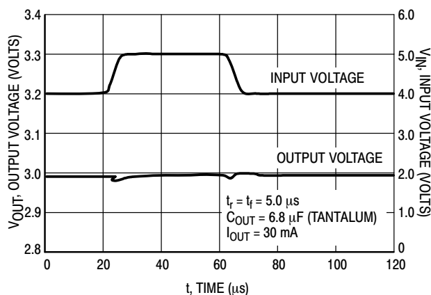
Figure 41. MC78PC30 Line Transient Response
