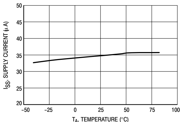
Figure 25. MC78PC30 Supply Current versus Temperature
