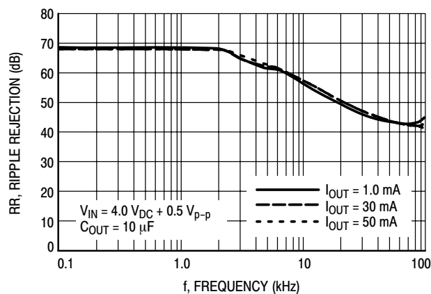
Figure 32. MC78PC30 Ripple Rejection versus Frequency
