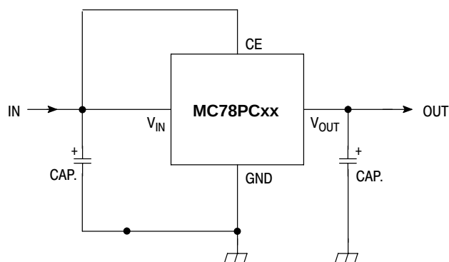
Figure 47. Typical Application
