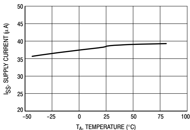
Figure 27. MC78PC50 Supply Current versus Temperature
