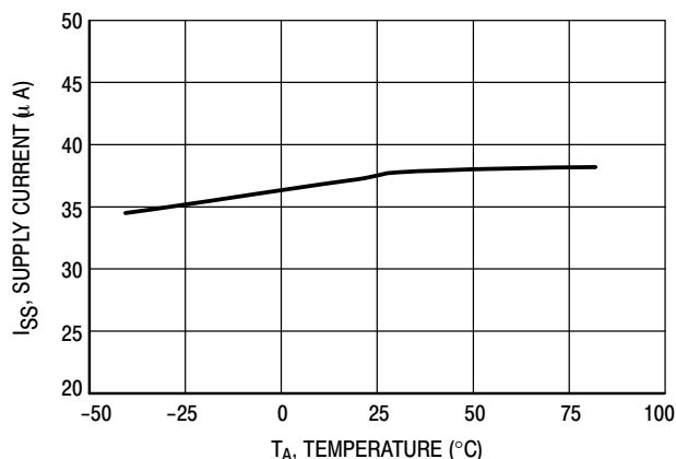
Figure 26. MC78PC40 (4.0 V) Supply Current versus Temperature
