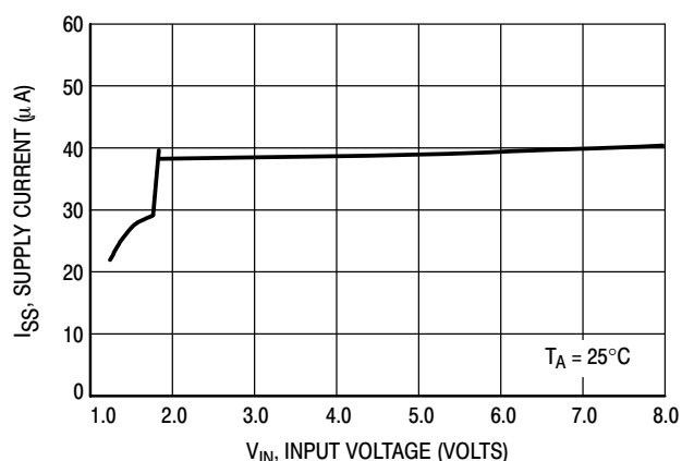
Figure 21. MC78PC18 Supply Current versus Input Voltage
