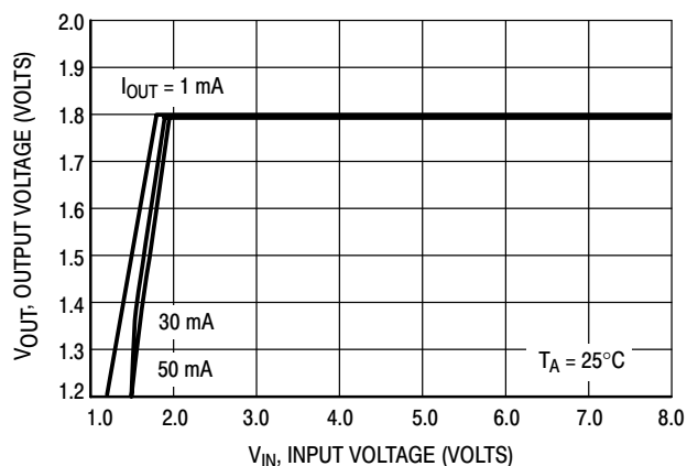
Figure 9. MC78PC18 Output Voltage versus Input Voltage
