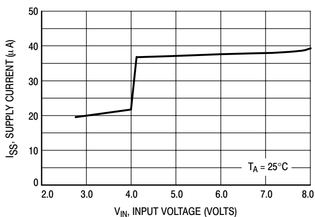
Figure 23. MC78PC40 (4.0 V) Supply Current versus Input Voltage
