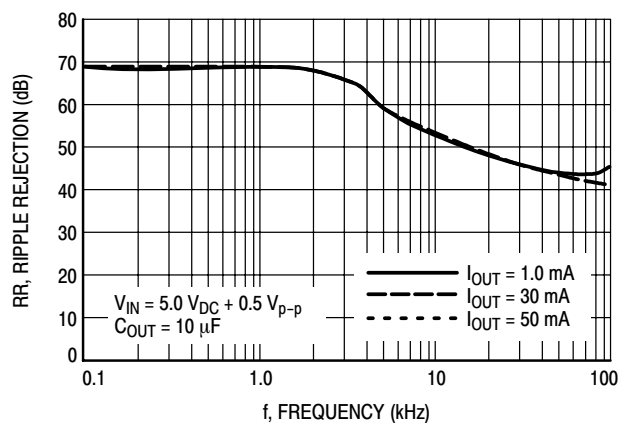
Figure 34. MC78PC40 (4.0 V) Ripple Rejection versus Frequency
