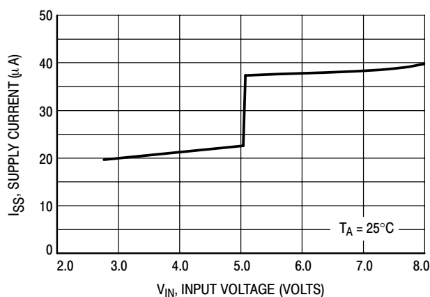
Figure 24. MC78PC50 Supply Current versus Input Voltage
