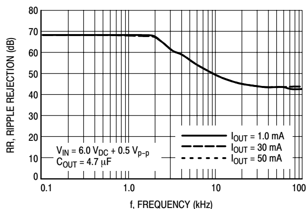
Figure 35. MC78PC50 Ripple Rejection versus Frequency
