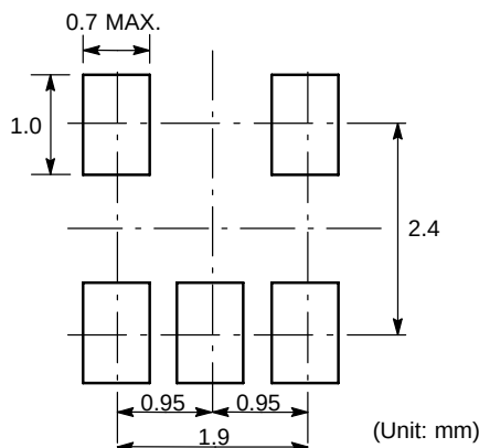
Figure 51. SOT-23-5
