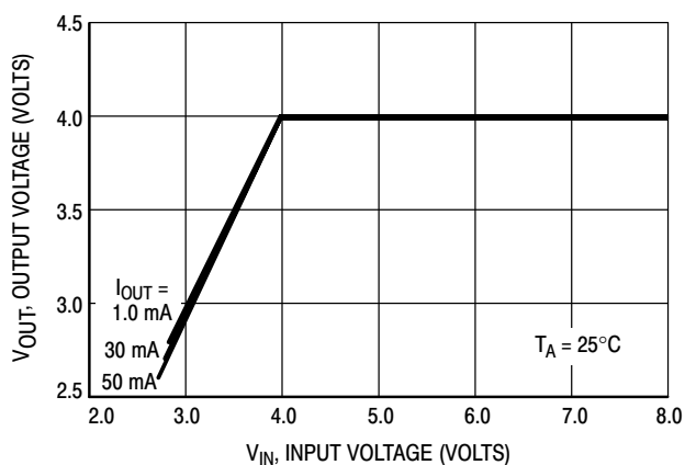
Figure 11. MC78PC40 (4.0 V) Output Voltage versus Input Voltage
