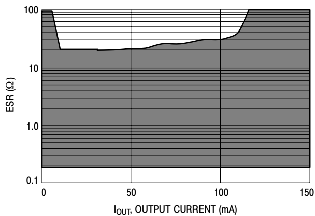
Figure 50. Ceramic Capacitor 10 \mu F
