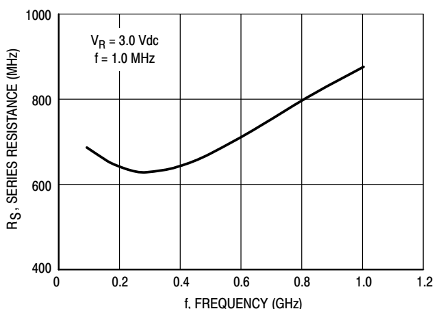
Figure 3. Series Resistance
