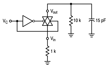
Figure 8. Crosstalk Test Circuit
