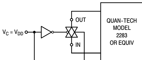
Figure 9. Noise Voltage Test Circuit
