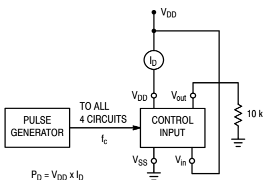
Figure 2. Quiescent Power Dissipation Test Circuit
