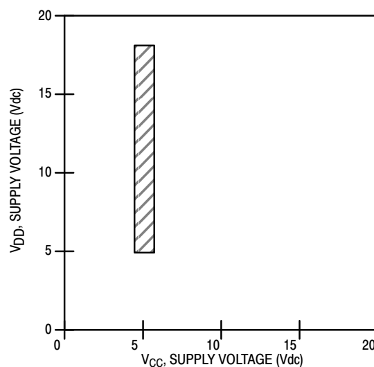
Figure 4. Operating Boundary TTL to CMOS Mode
