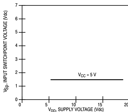
Figure 2. Input Switchpoint TTL to CMOS Mode
