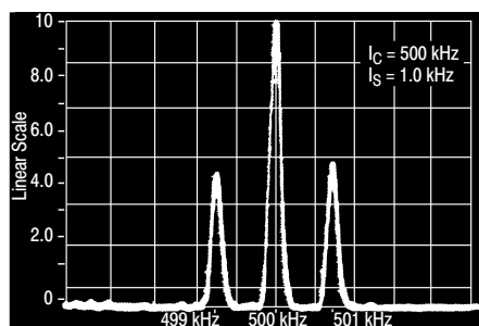
Figure 4. Amplitude-Modulation Spectrum
