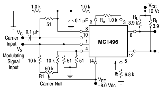
Figure 26. Balanced Modulator-Demodulator
