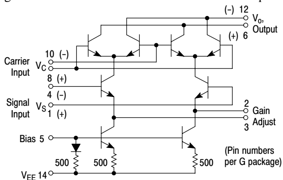
Figure 23. Circuit Schematic
