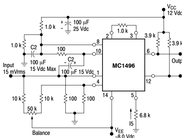
Figure 30. Low-Frequency Doubler
