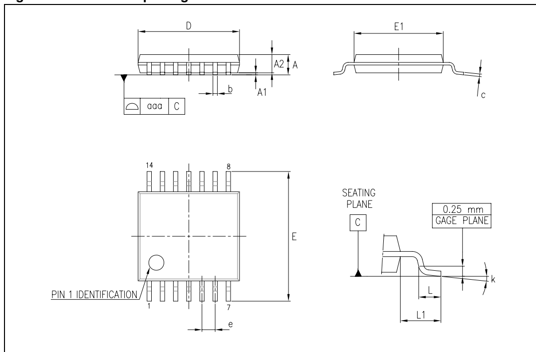
Figure 53. TSSOP14 package outline
