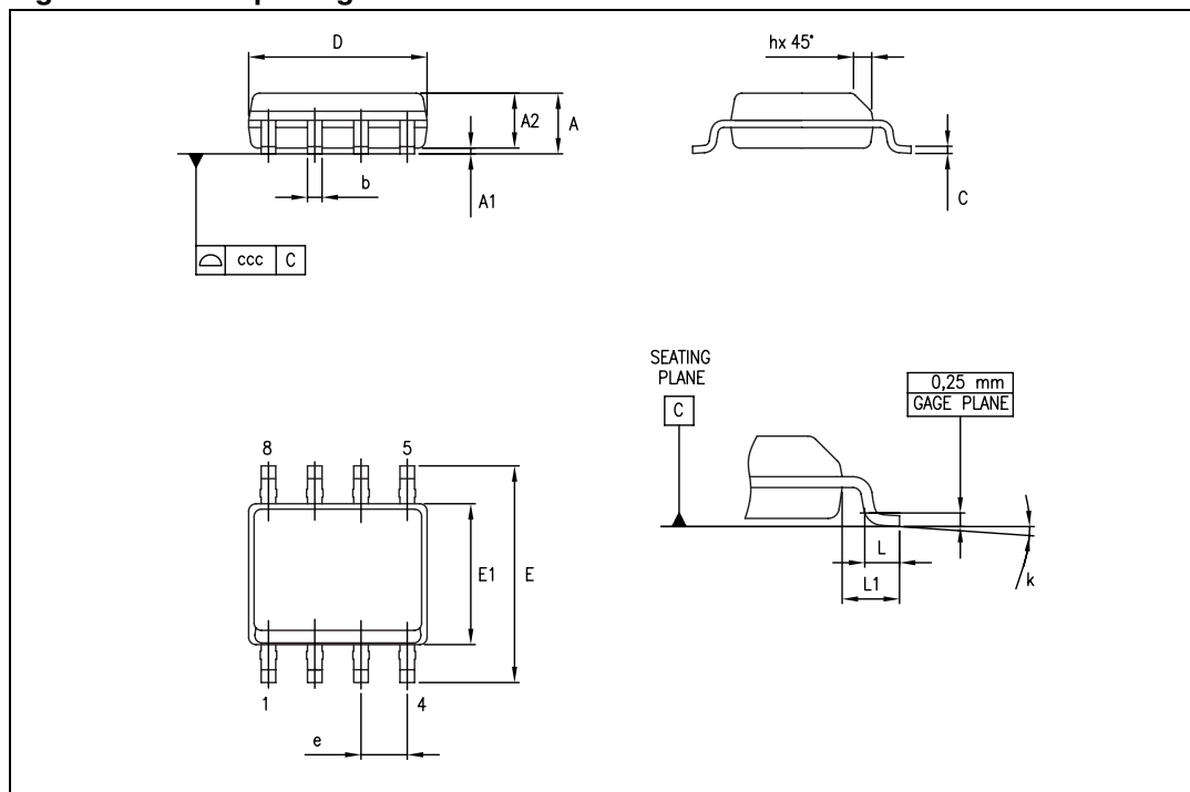
Figure 49. SO-8 package outline
