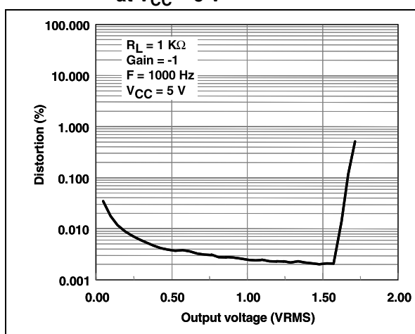
Figure 39. Distortion vs. output voltage at V_{CC} = 5\text{ V}
