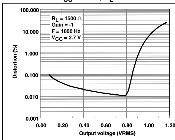
Figure 41. Distortion vs. output voltage at V_{CC} = 2.7\text{ V} , R_L = 1500\ \Omega
