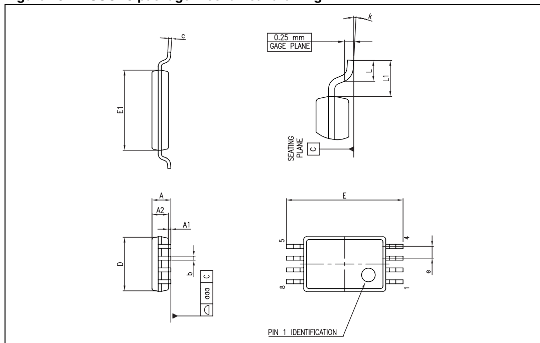
Figure 16. TSSOP8 package mechanical drawing
