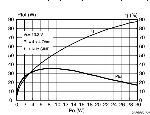
Figure 16. Power dissipation and efficiency vs. output power (sine-wave operation)
