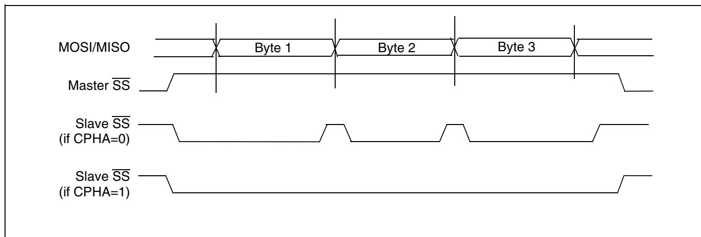
Figure 49. Hardware/Software Slave Select Management
