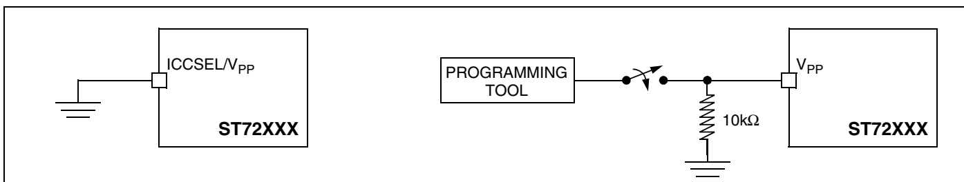
Figure 79. Two typical Applications with ICCSEL/V PP Pin 2)
