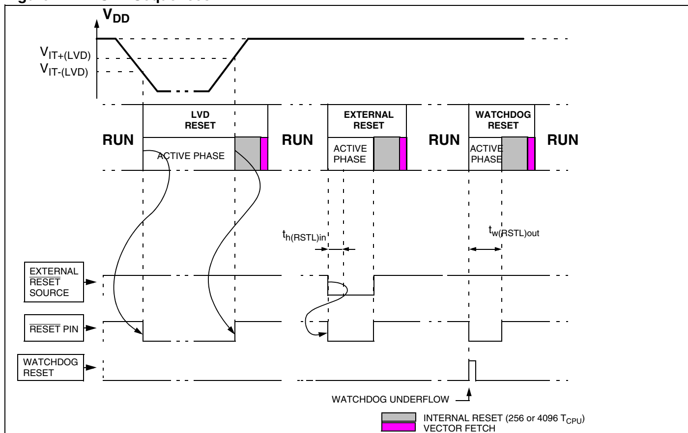
Figure 14. RESET Sequences
