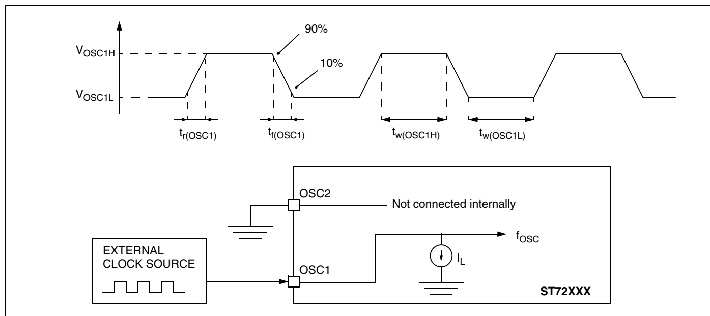
Figure 65. Typical Application with an External Clock Source
