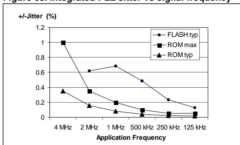
Figure 68. Integrated PLL Jitter vs signal frequency 1
