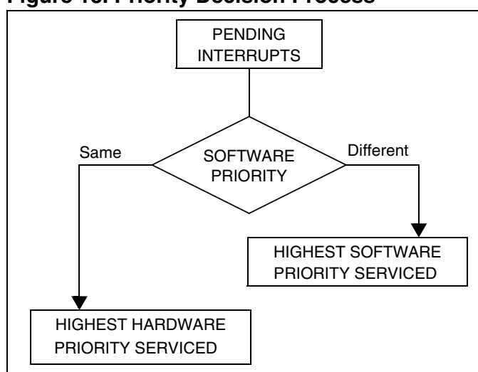
Figure 18. Priority Decision Process
