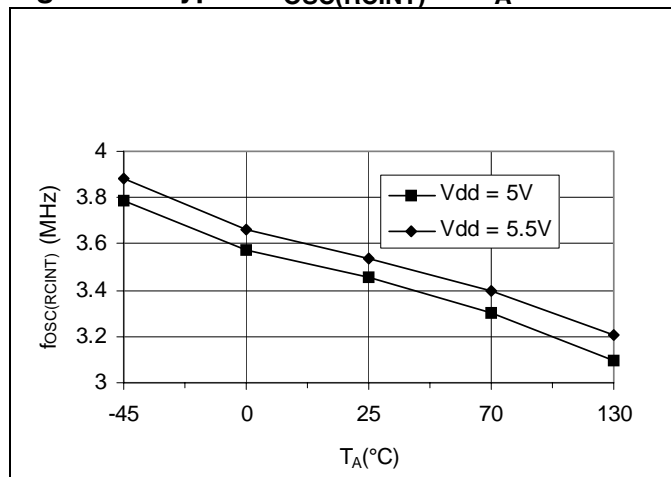
Figure 67. Typical f_{OSC(RCINT)} vs T_A
