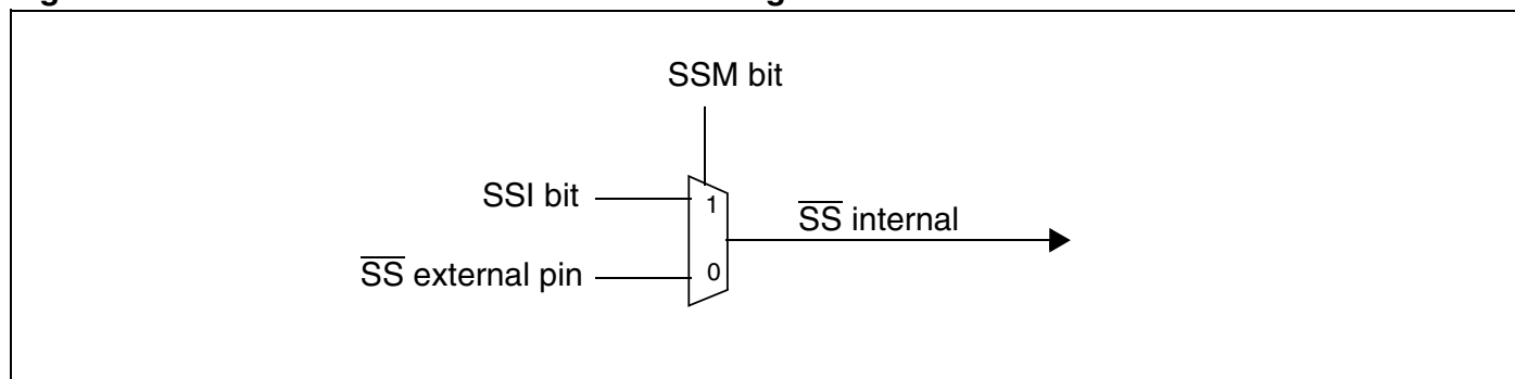
Figure 49. Hardware/Software Slave Select Management
