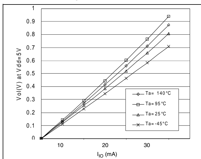
Figure 72. Typ. V_{OL} at V_{DD}=5V (high-sink ports)
