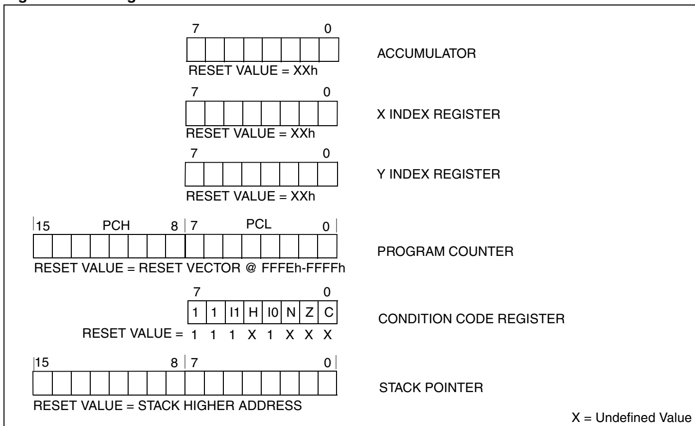
Figure 8. CPU Registers
