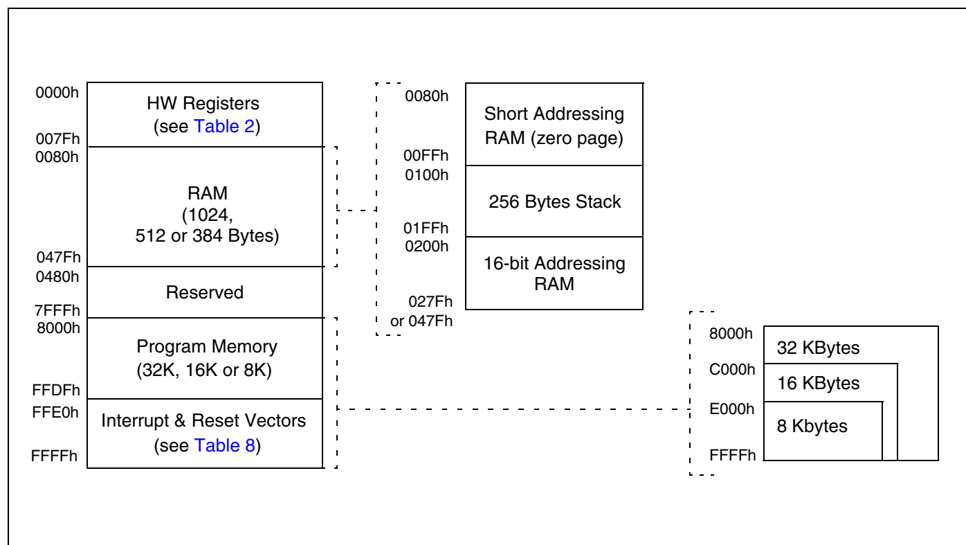
Figure 5. Memory Map
