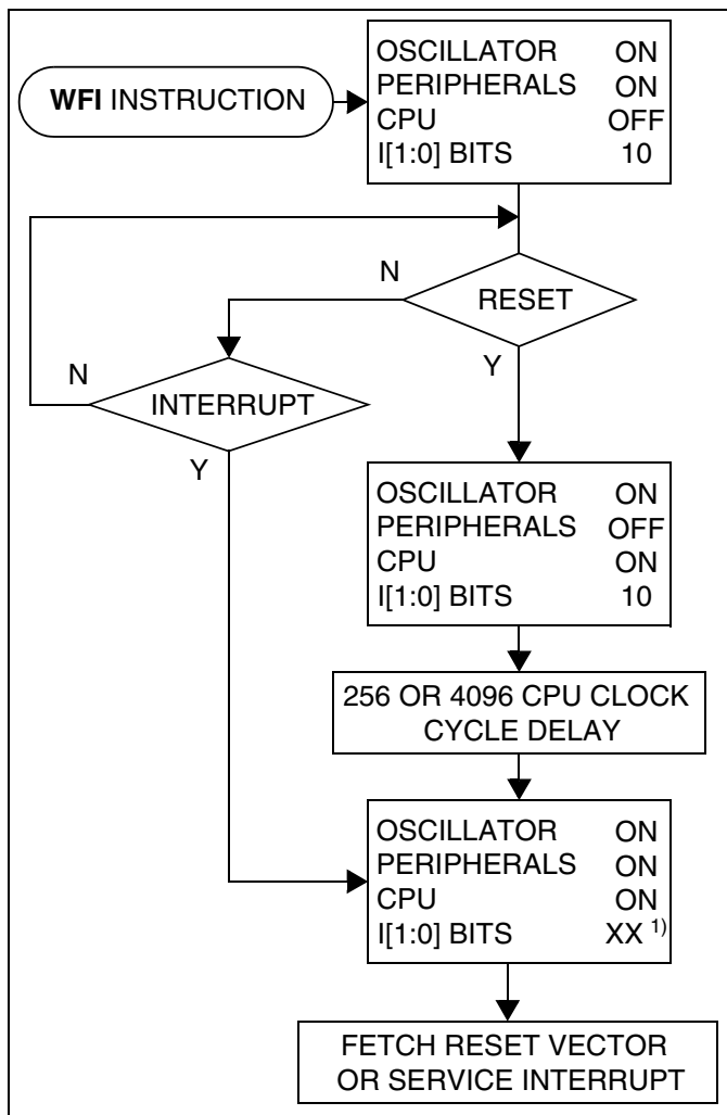
Figure 24. WAIT Mode Flow-chart
