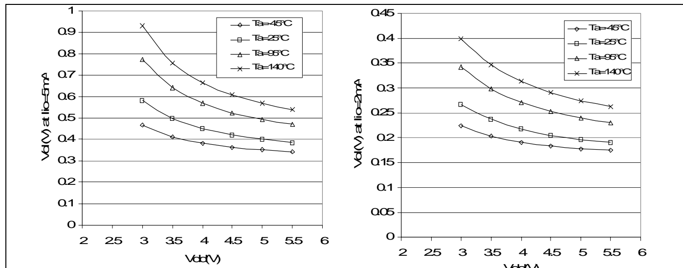
Figure 75. Typical V_{OL} vs. V_{DD} (high-sink ports)
