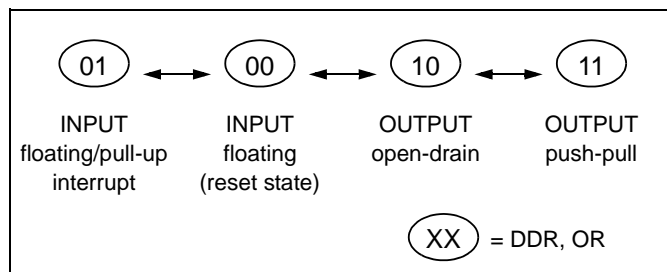
Figure 30. Interrupt I/O Port State Transitions
