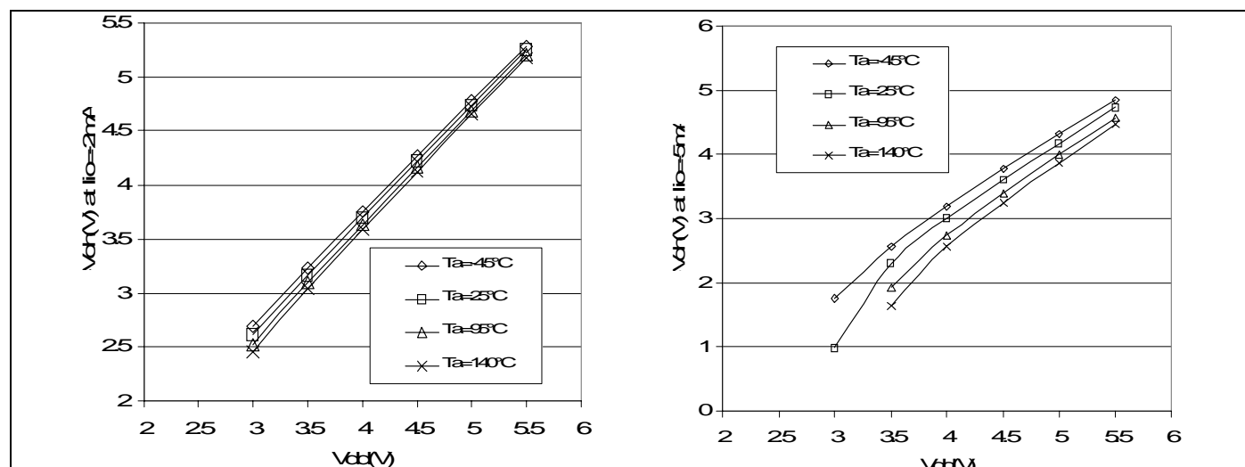
Figure 76. Typical V_{OH} vs. V_{DD}
