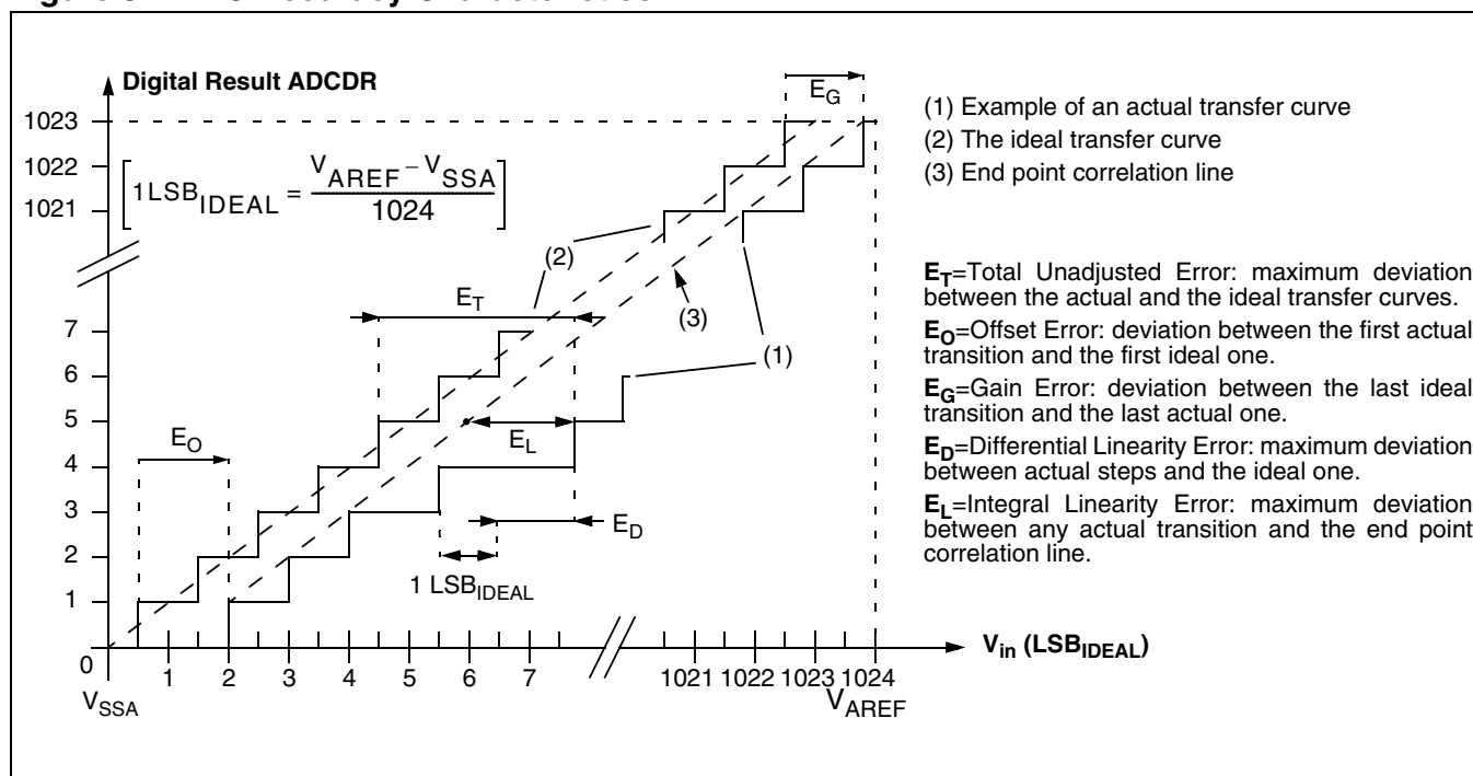
Figure 87. ADC Accuracy Characteristics
