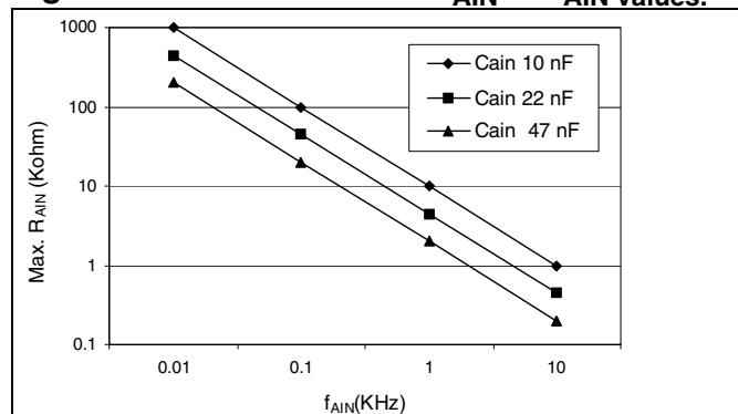
Figure 84. Recommended C_{AIN} & R_{AIN} values. 2)
