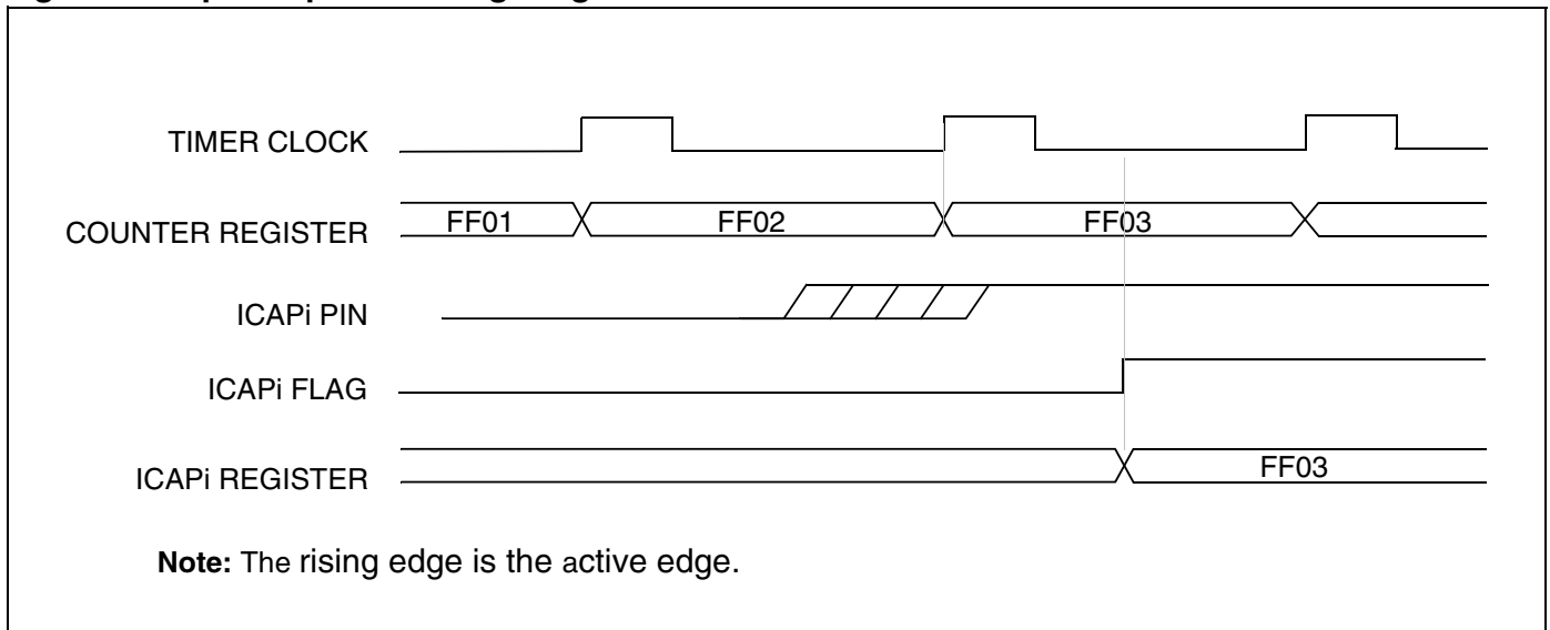
Figure 40. Input Capture Timing Diagram
