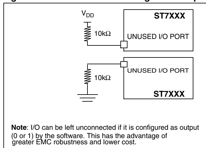
Figure 69. Unused I/O Pins configured as input
