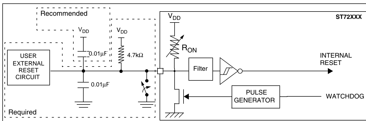
Figure 78. RESET pin protection when LVD is disabled. 1)2)3)4)
