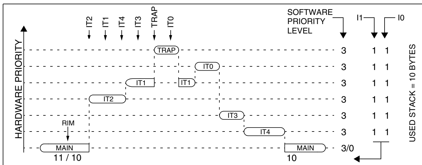
Figure 19. Concurrent Interrupt Management
