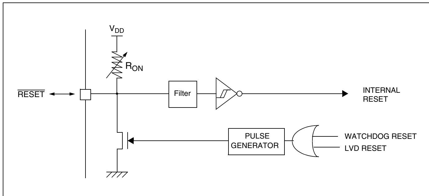
Figure 13. Reset Block Diagram
