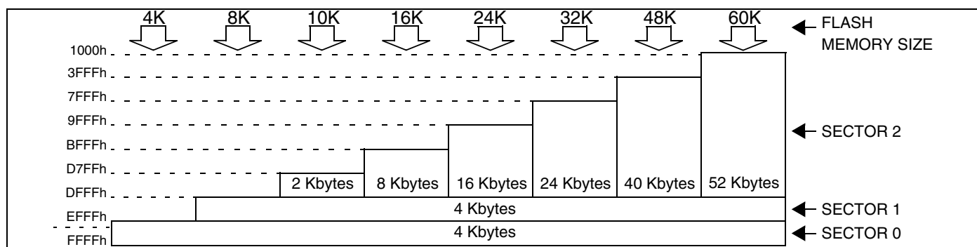
Figure 6. Memory Map and Sector Address
