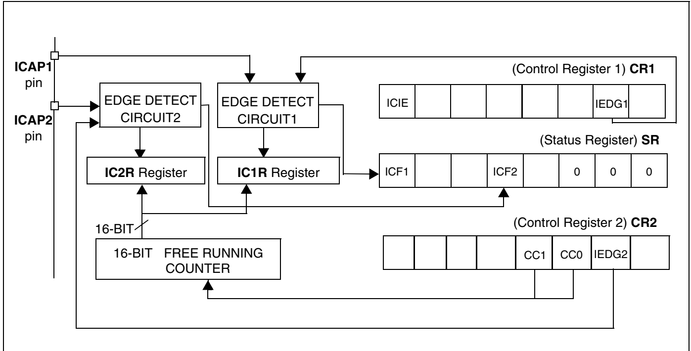
Figure 39. Input Capture Block Diagram
