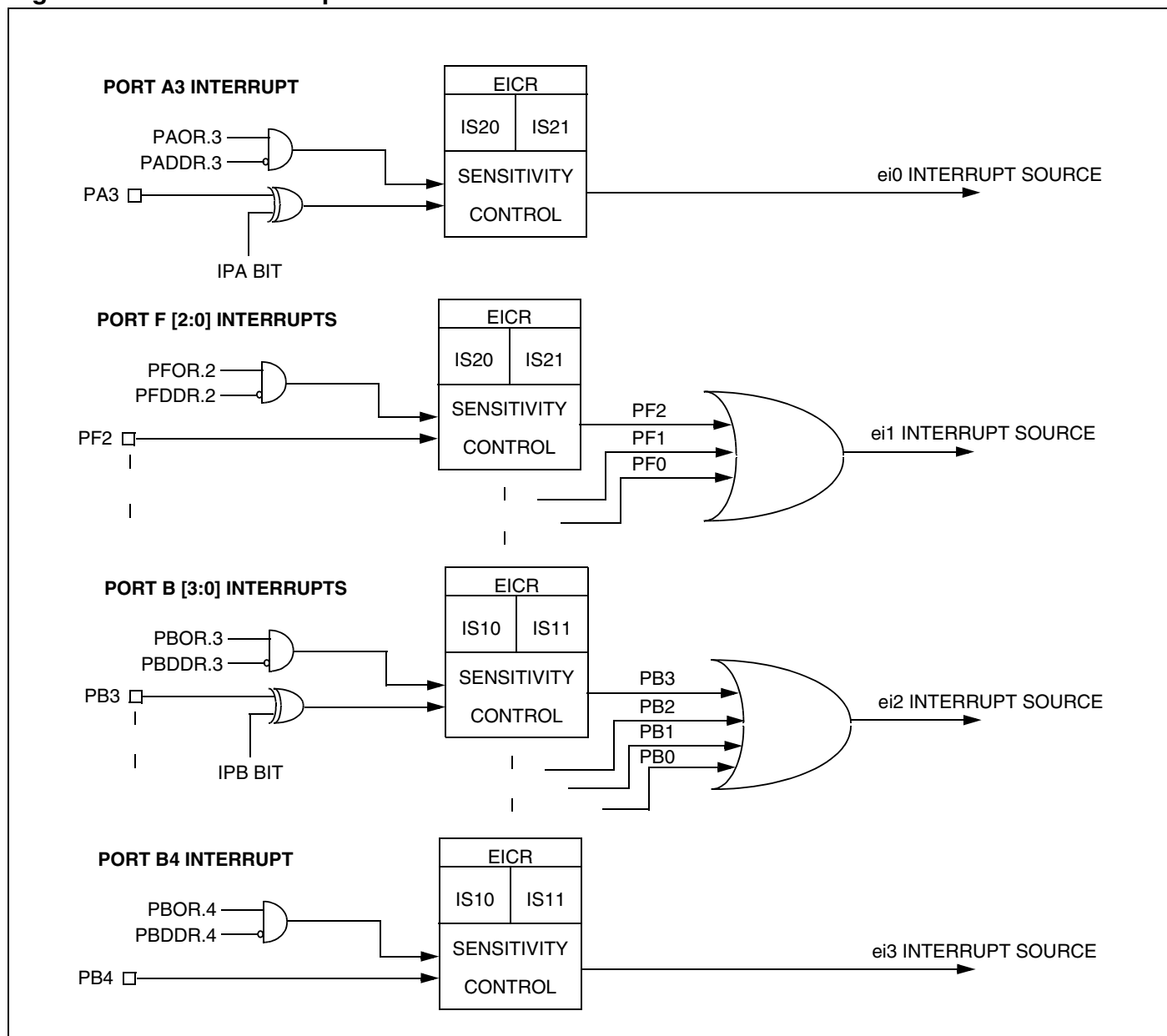
Figure 21. External Interrupt Control bits
