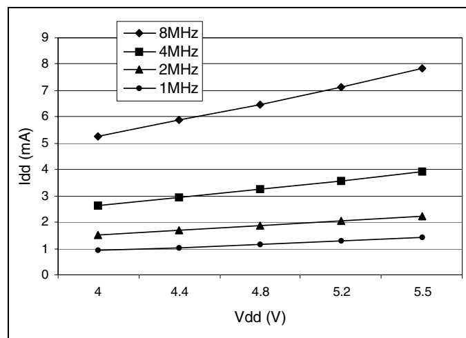
Figure 62. Typical I_{DD} in SLOW mode
