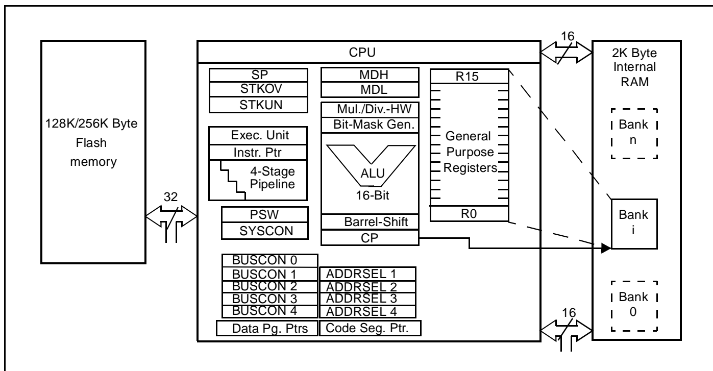
Figure 9 : CPU Block Diagram (MAC Unit not included)
