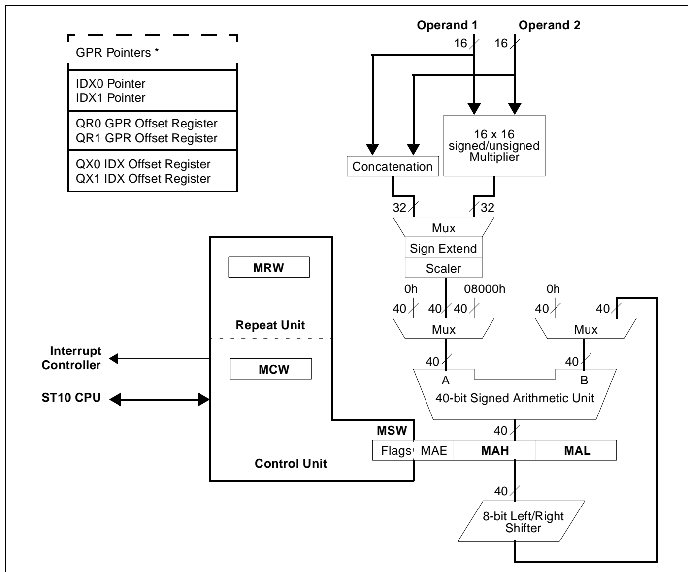
Figure 10 : MAC Unit Architecture
