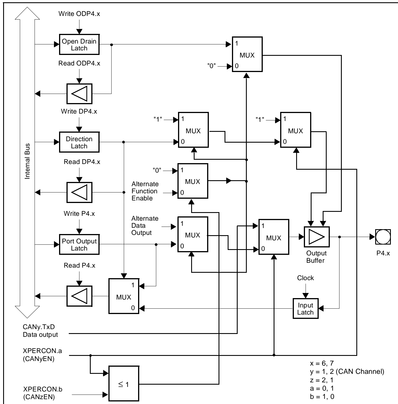
Figure 33 : Block Diagram of P4.6 and P4.7 Pins
