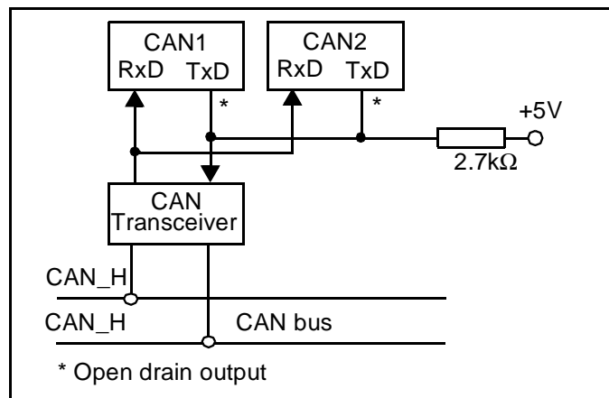
Figure 48 : Single CAN Bus, Dual Interfaces, Single Transceiver
