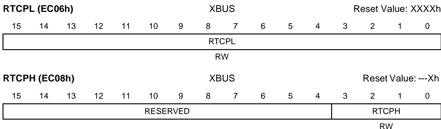
Figure 52 : PRESCALER Register
