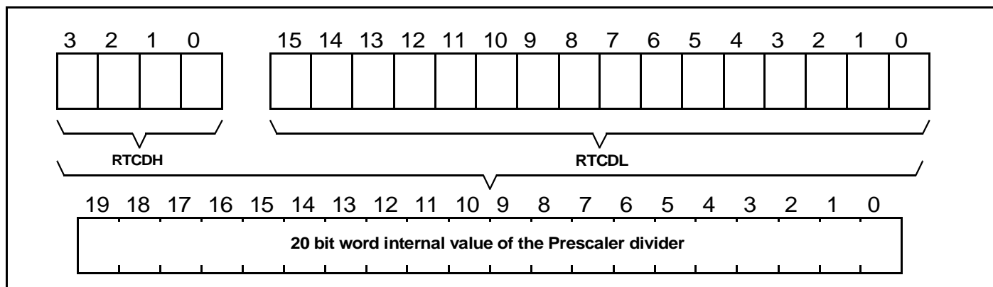
Figure 53 : DIVIDER Counters
