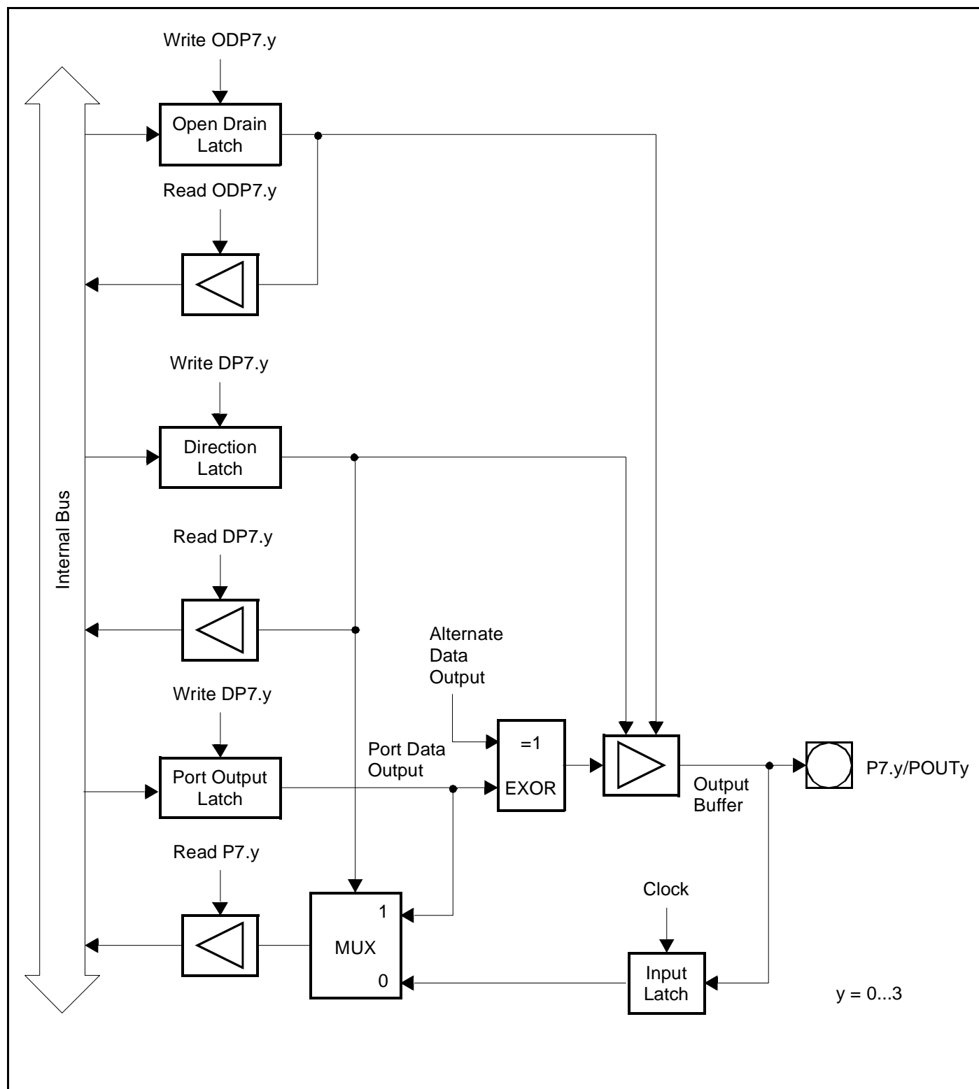
Figure 40 : Block Diagram of Port 7 Pins P7.3...P7.0
