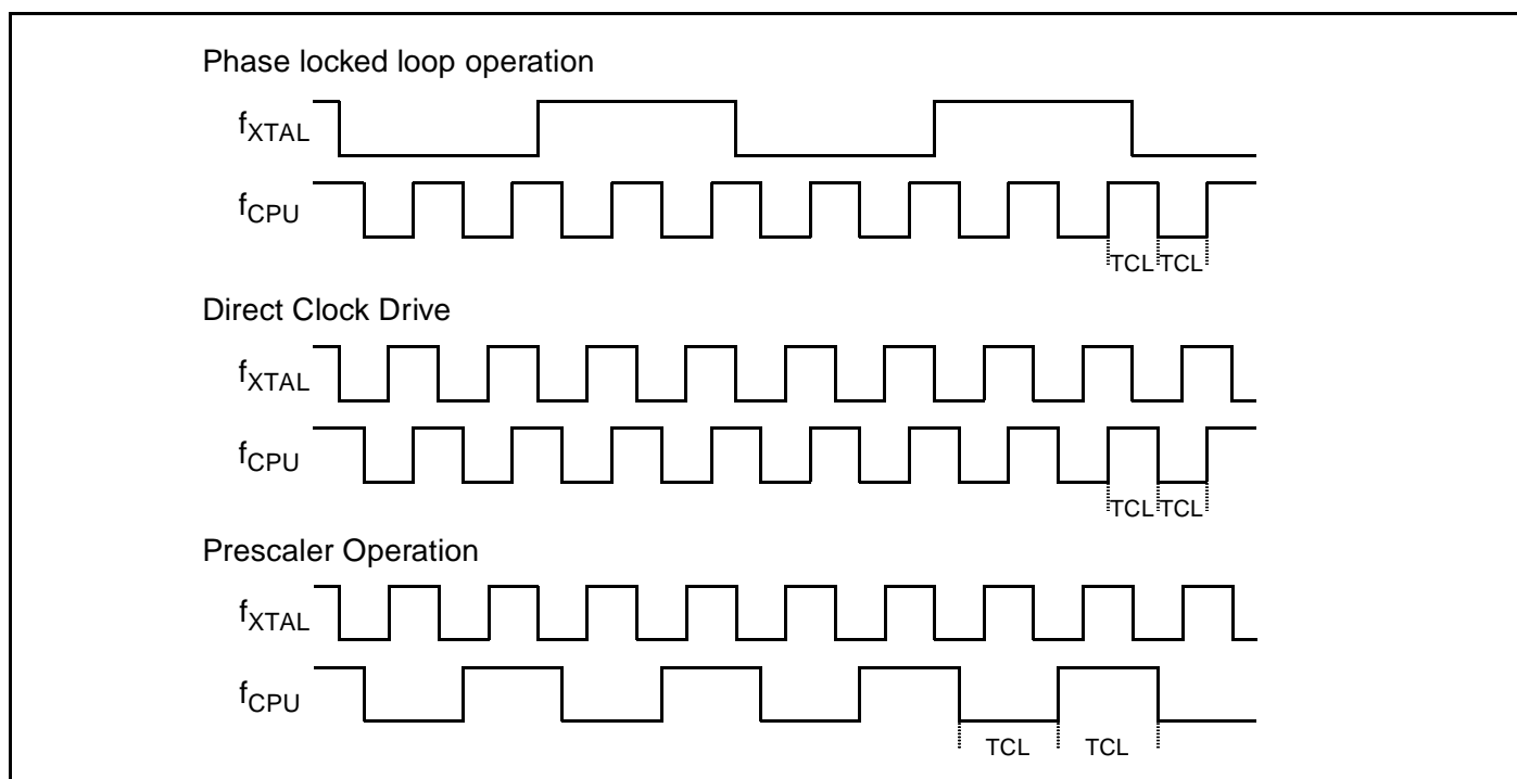
Figure 68 : Generation Mechanisms for the CPU Clock
