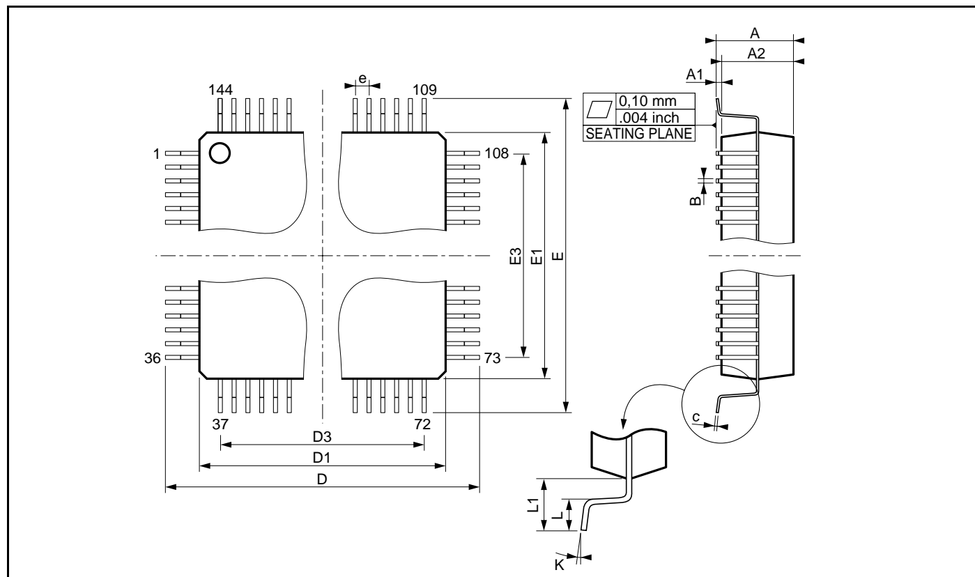
Figure 84 : Package Outline PQFP144 (28 x 28mm)
