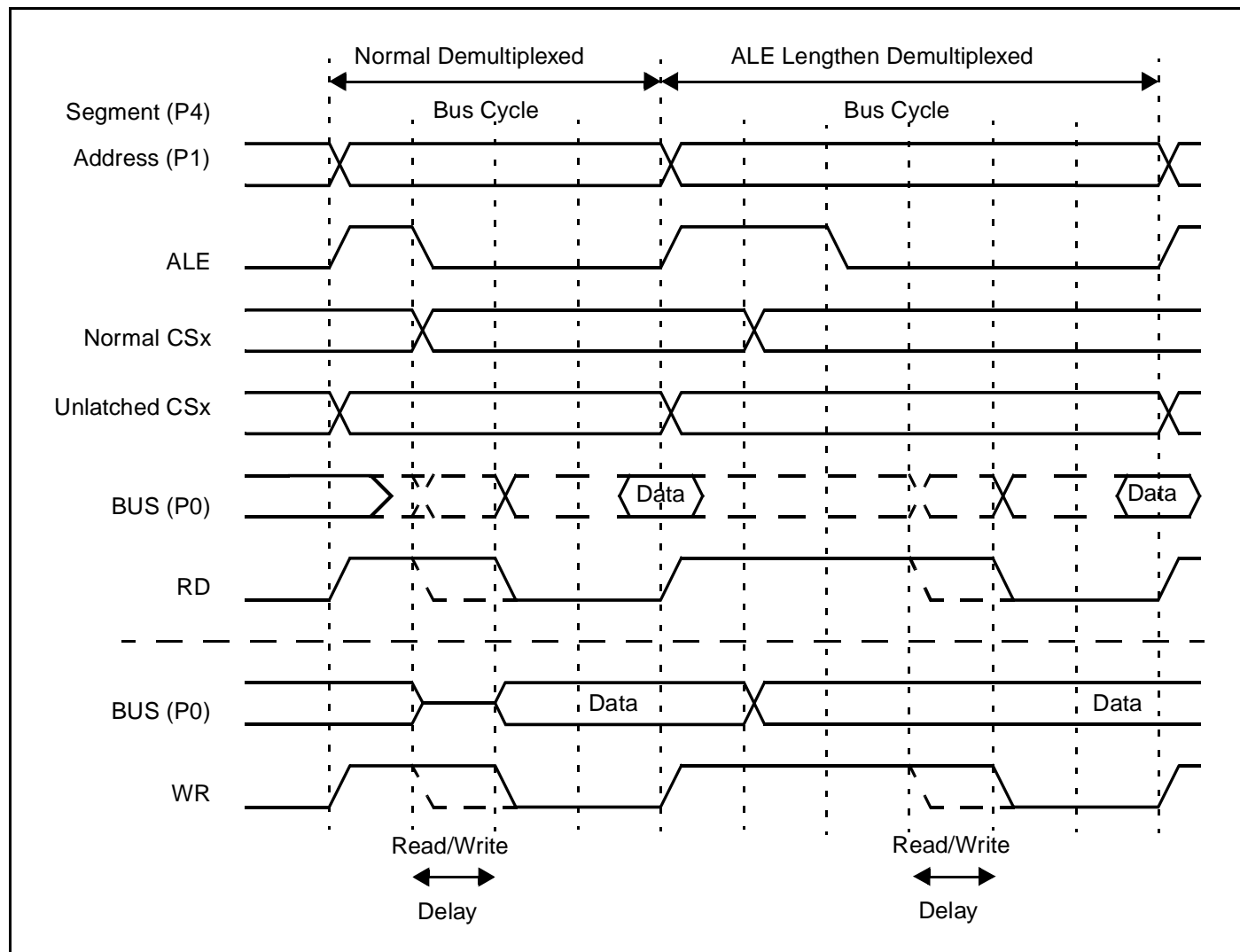
Figure 11 : Chip Select Delay
