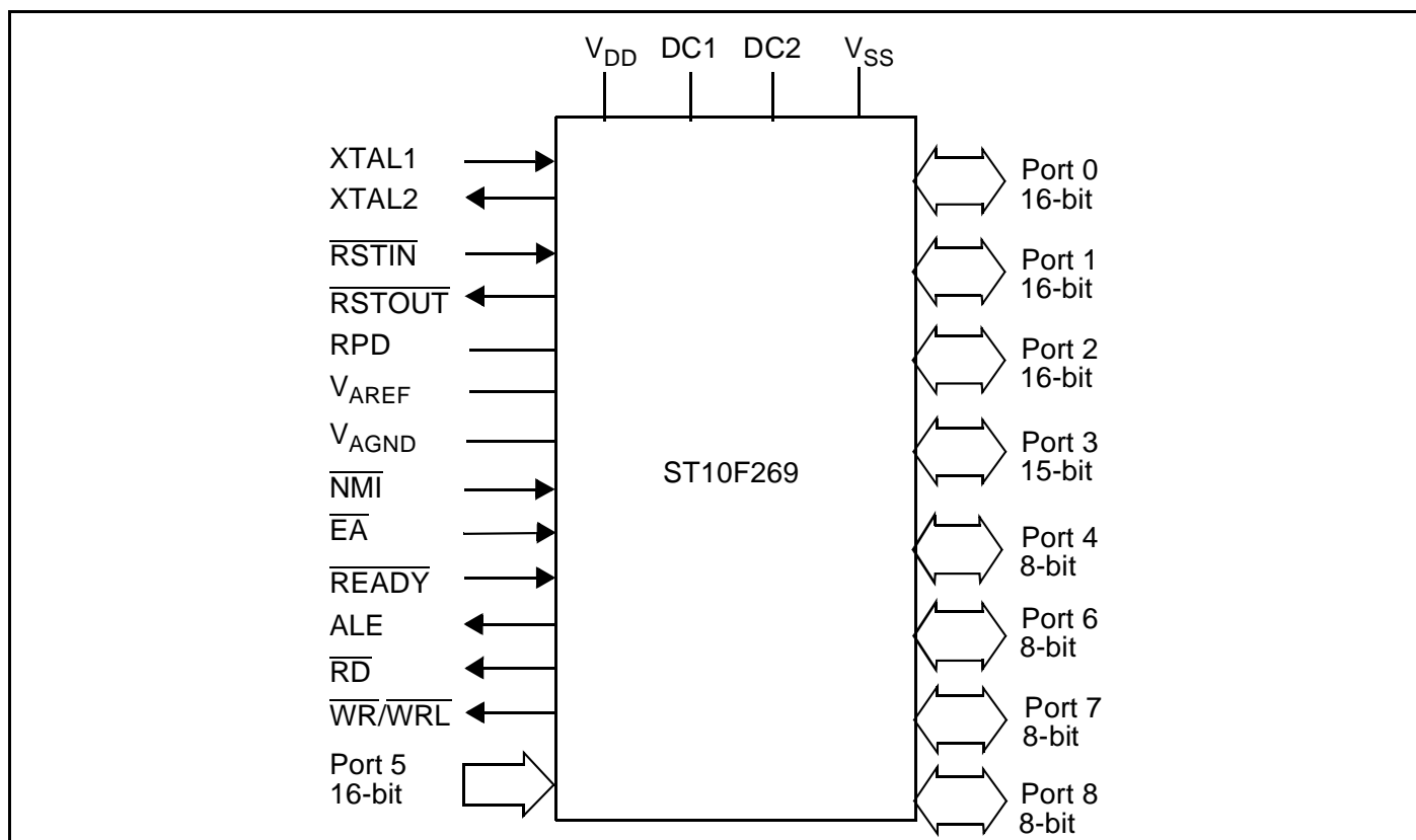
Figure 1 : Logic Symbol
