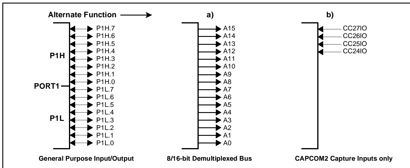
Figure 23 : PORT1 I/O and Alternate Functions
