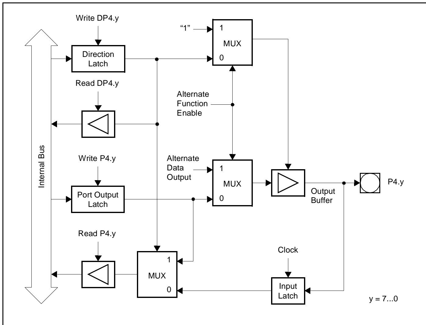
Figure 31 : Block Diagram of a Port 4 Pin
