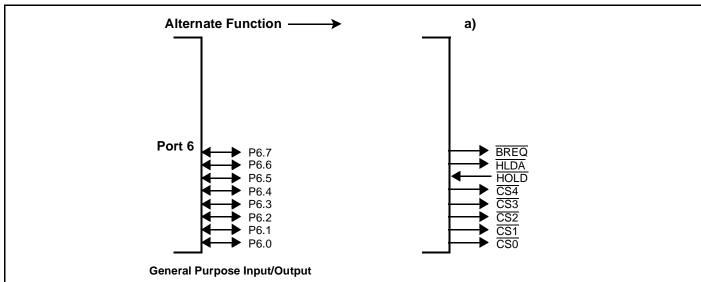
Figure 36 : Port 6 I/O and Alternate Functions
