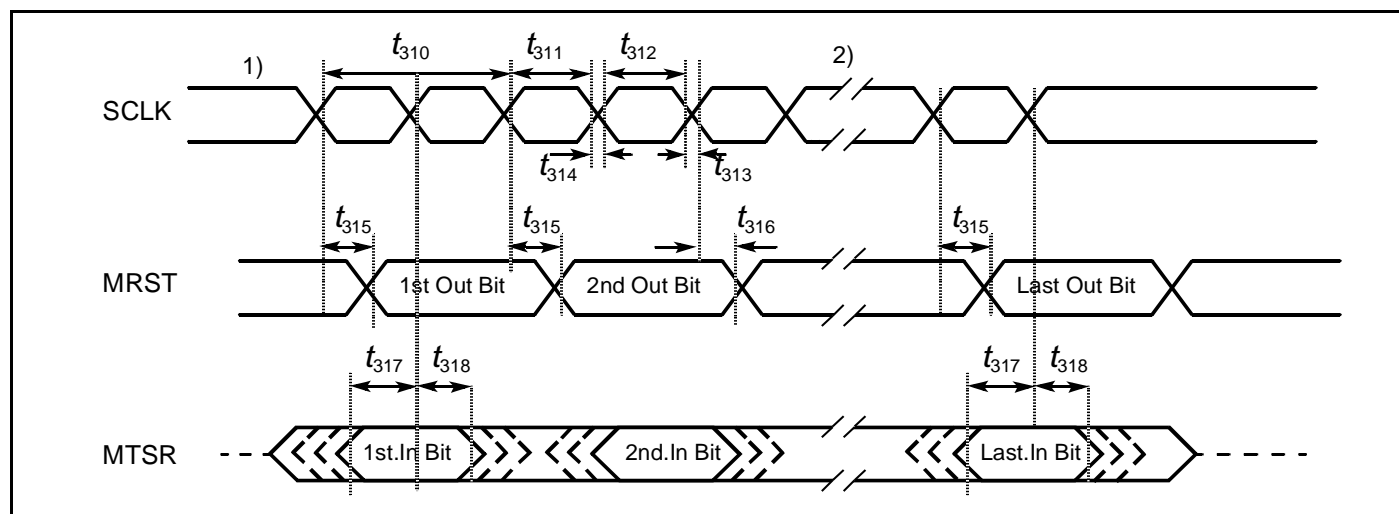
Figure 83 : SSC Slave Timing
