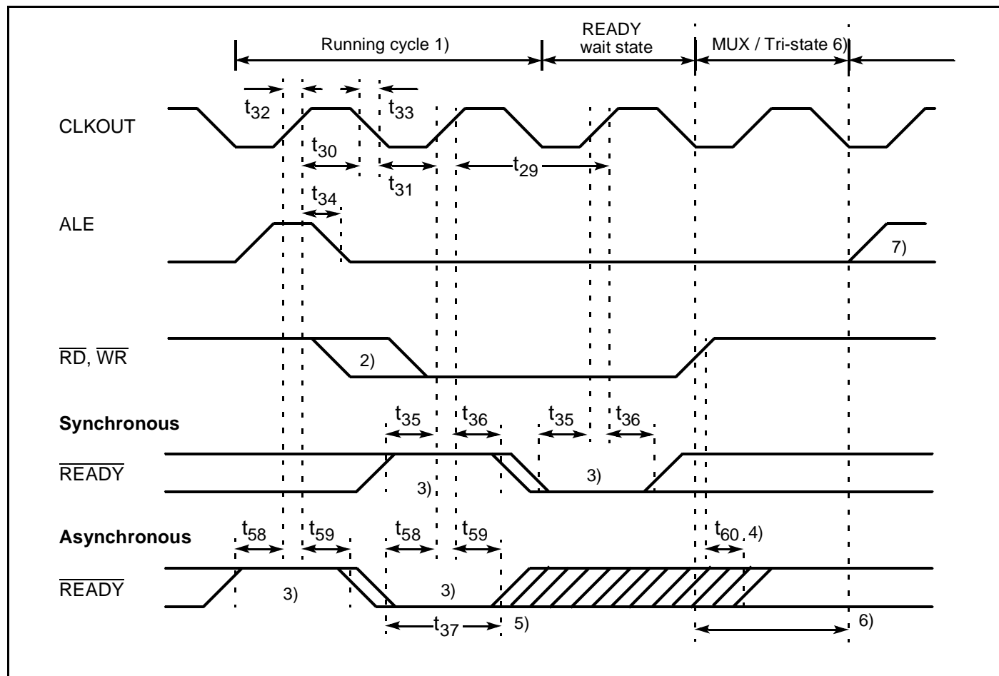
Figure 79 : CLKOUT and \overline{\text{READY}}
