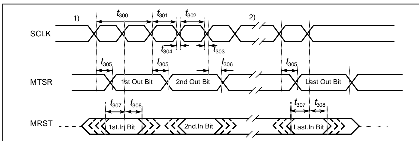
Figure 82 : SSC Master Timing
