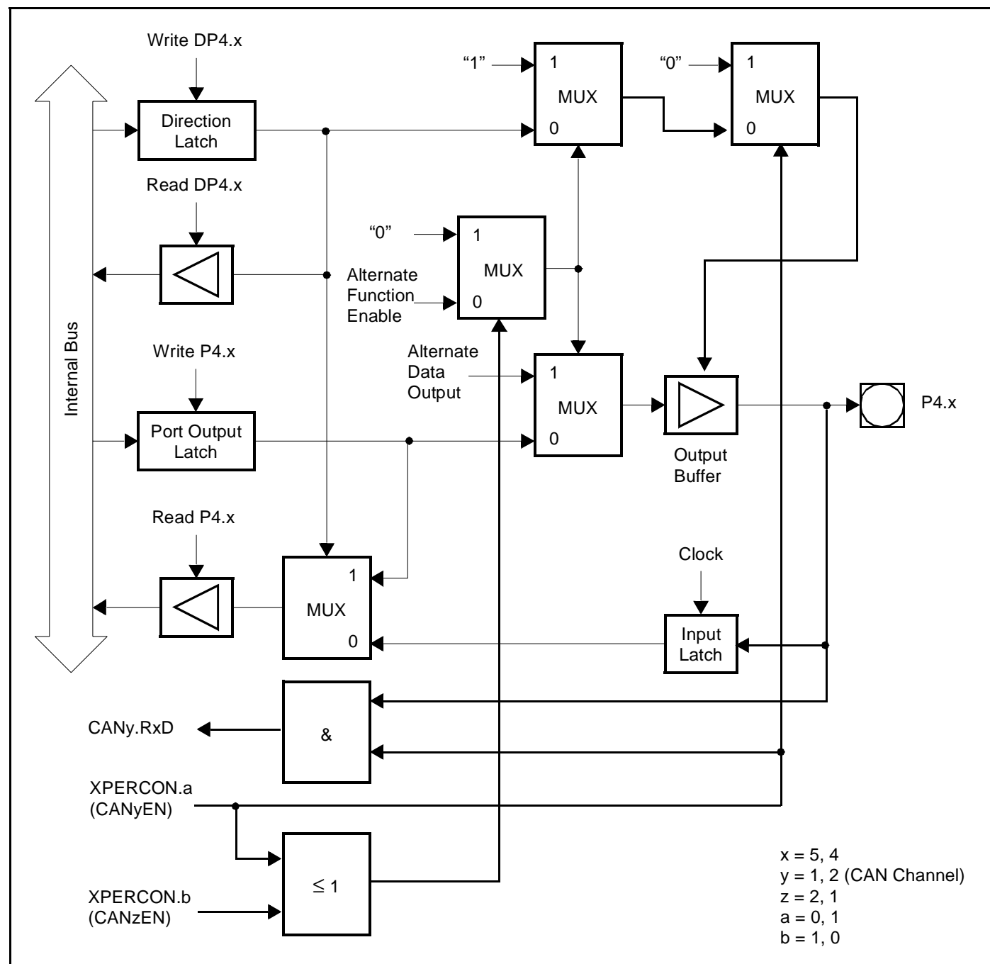
Figure 32 : Block Diagram of P4.4 and P4.5 Pins
