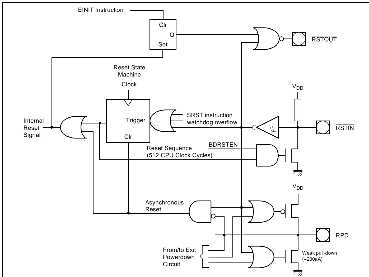
Figure 58 : Internal (simplified) Reset Circuitry.
