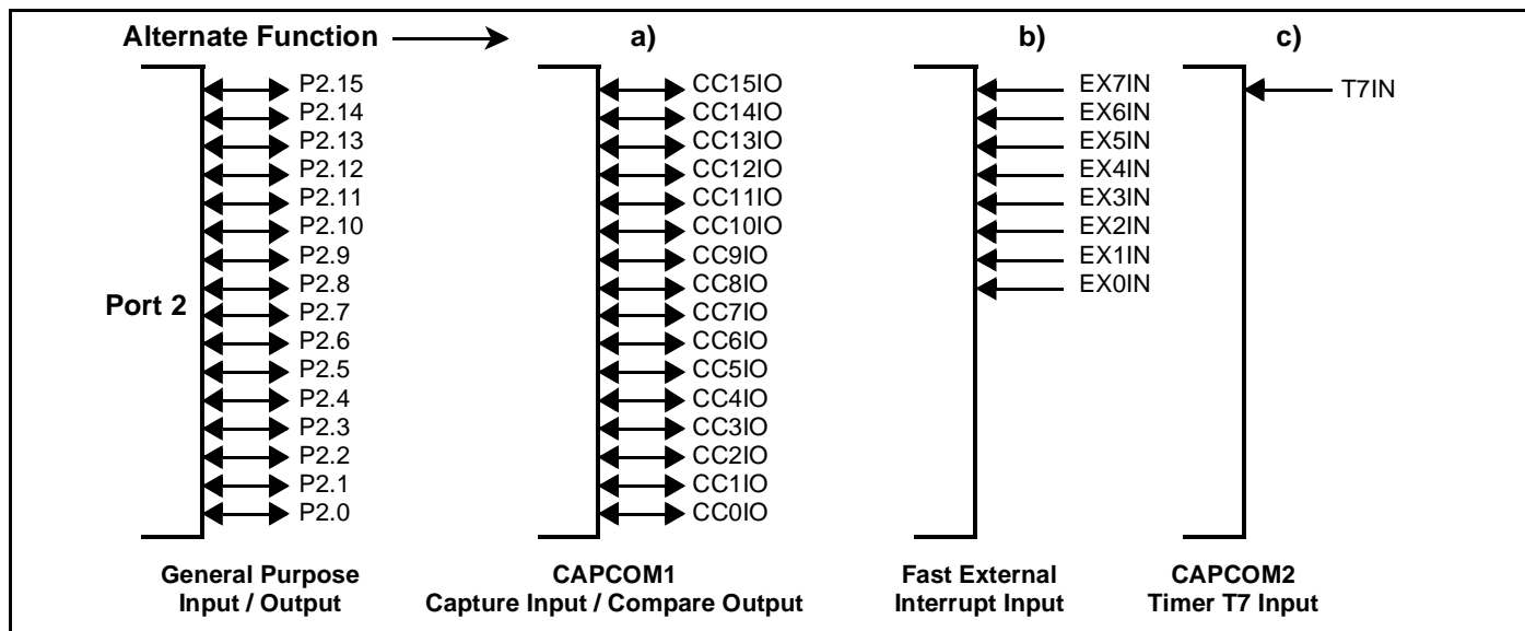
Figure 25 : Port 2 I/O and Alternate Functions
