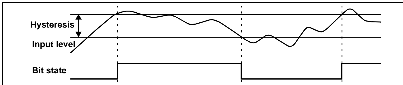
Figure 20 : Hysteresis for Special Input Thresholds
