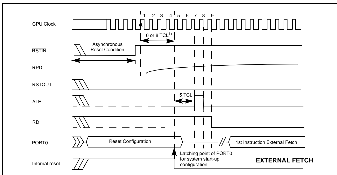
Figure 54 : Asynchronous Reset Sequence External Fetch
