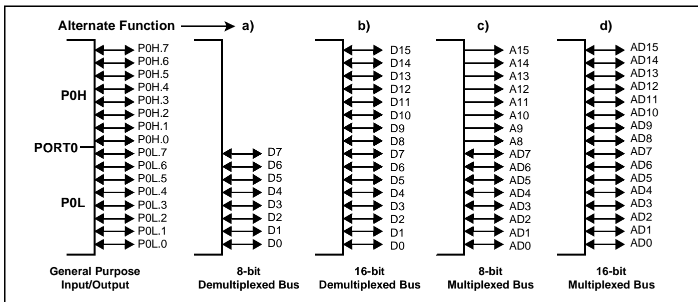
Figure 21 : PORT0 I/O and Alternate Functions
