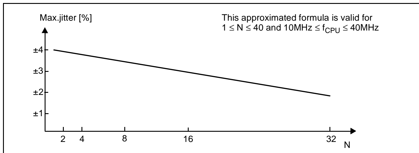
Figure 69 : Approximated Maximum PLL Jitter
