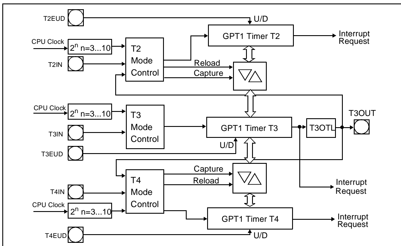
Figure 15 : Block Diagram of GPT1
