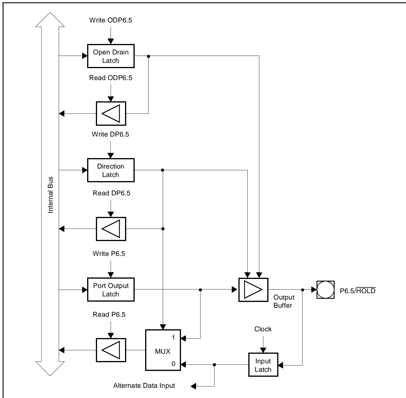
Figure 38 : Block Diagram of Pin P6.5 ( \overline{\text{HOLD}} )
