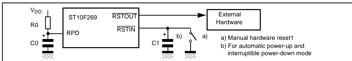
Figure 60 : External Reset Hardware Circuitry
