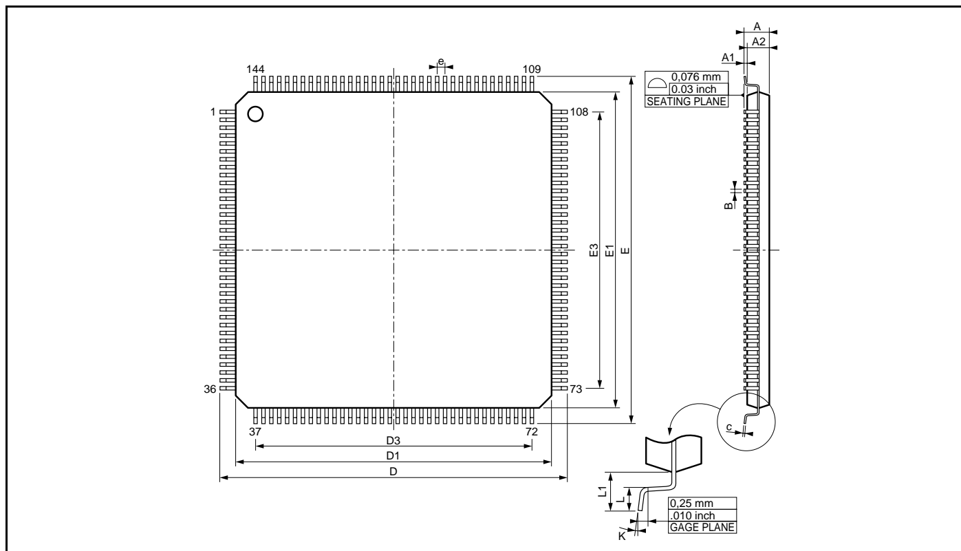
Figure 85 : Package Outline TQFP144 (20 x 20 x 1.40 mm)
