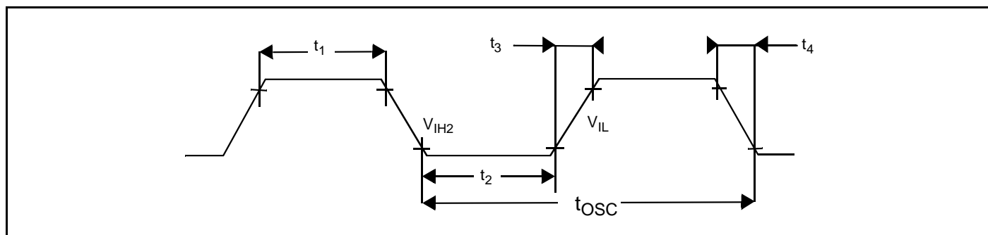
Figure 70 : External Clock Drive XTAL1
