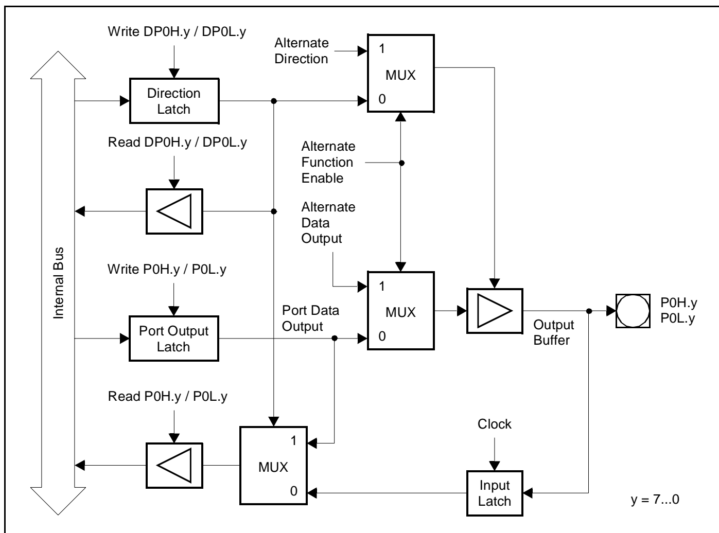
Figure 22 : Block Diagram of a PORT0 Pin
