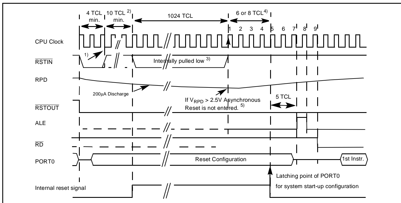
Figure 57 : Synchronous Warm Reset Sequence External Fetch ( 4 \text{ TCL} < \overline{RSTIN} pulse < 1038 \text{ TCL} )
