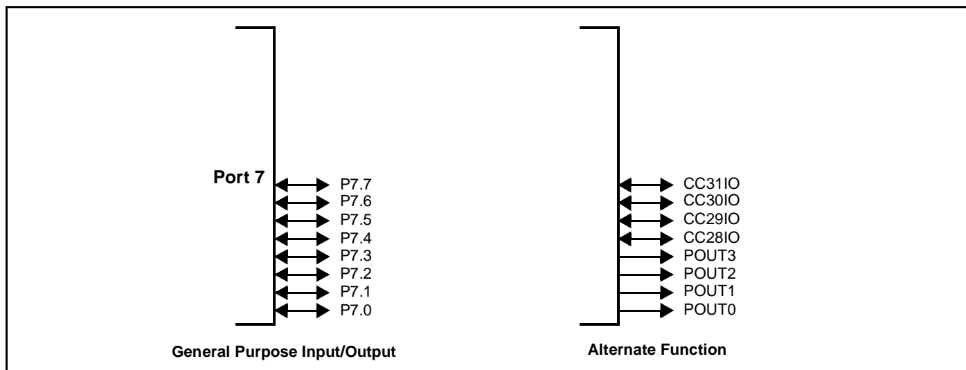
Figure 39 : Port 7 I/O and Alternate Functions
