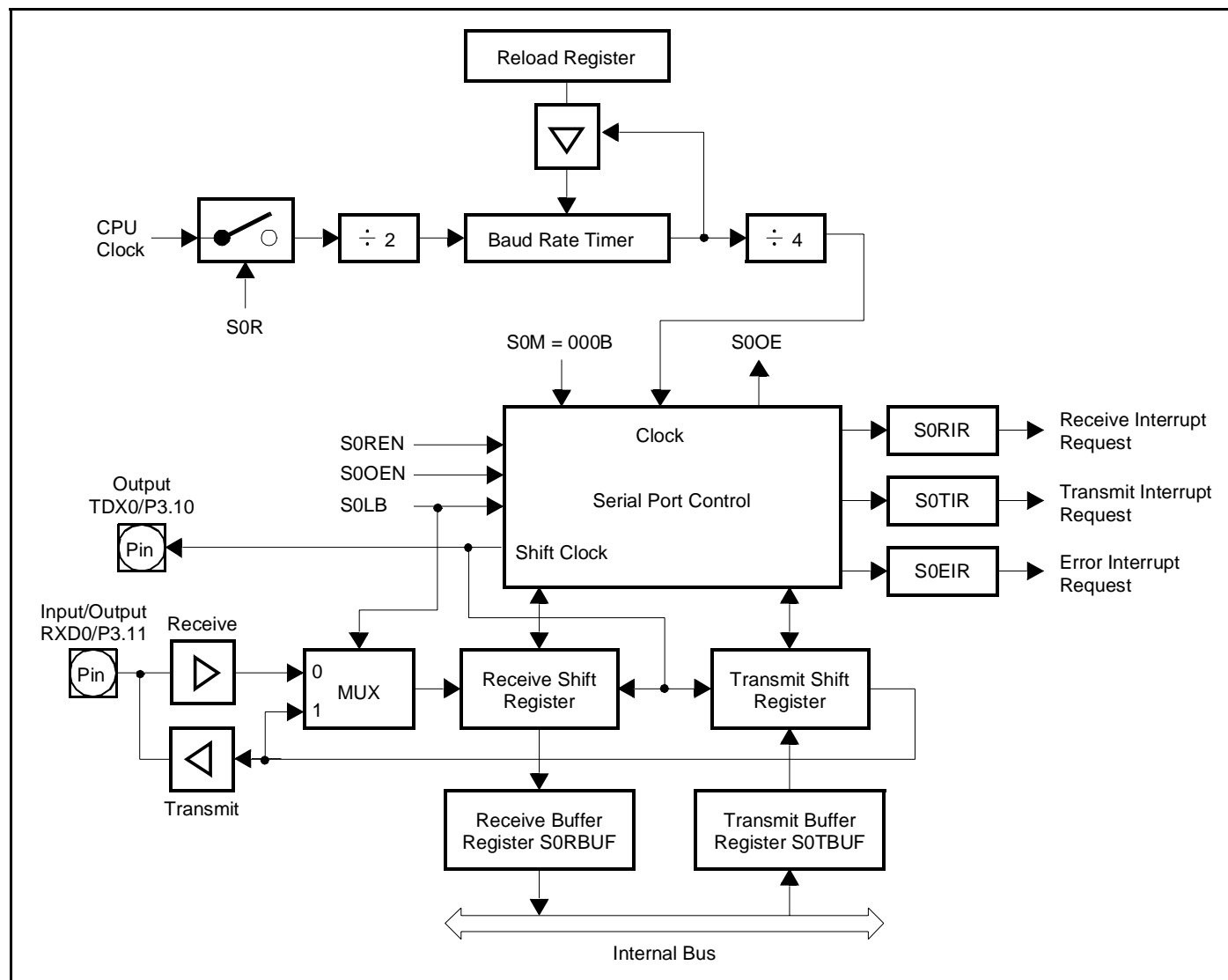
Figure 45 : Synchronous Mode of Serial Channel ASC0
