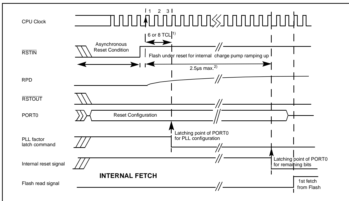
Figure 55 : Asynchronous Reset Sequence Internal Fetch
