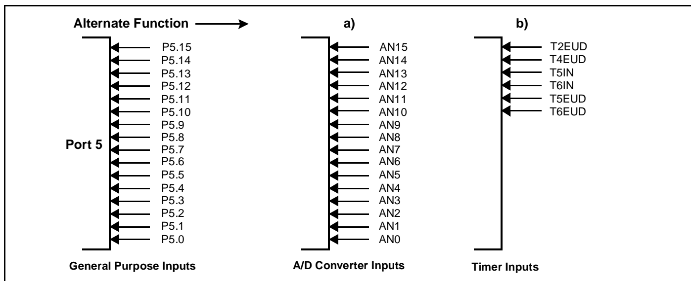
Figure 34 : Port 5 I/O and Alternate Functions
