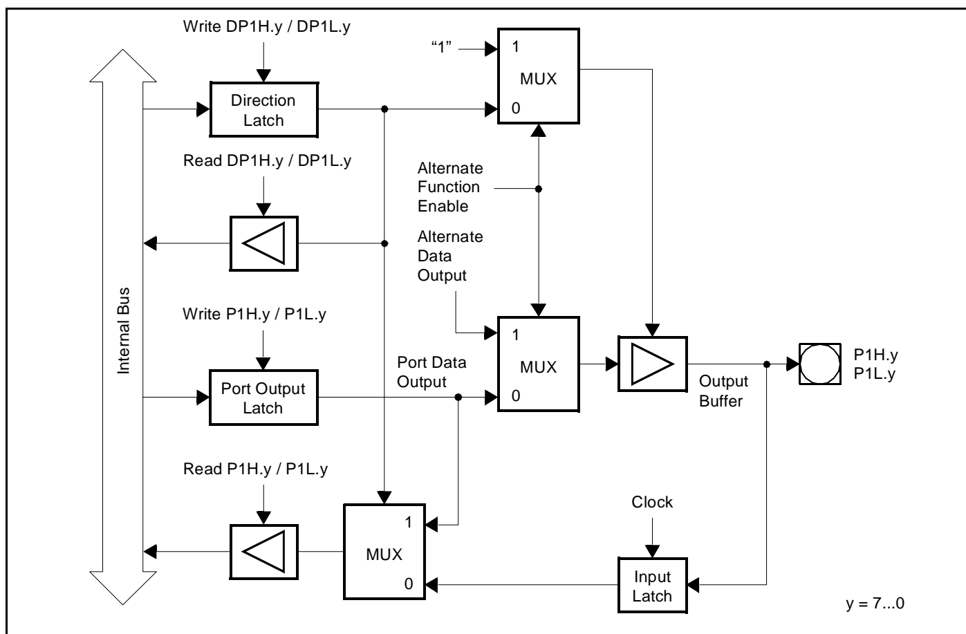
Figure 24 : Block Diagram of a PORT1 Pin
