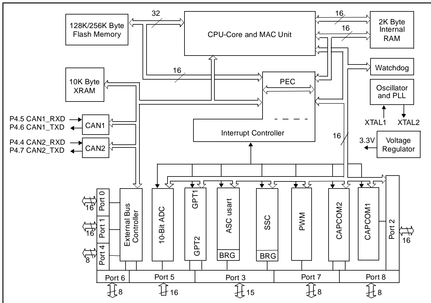
Figure 3 : Block Diagram
