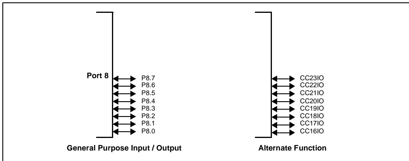
Figure 42 : Port 8 I/O and Alternate Functions
