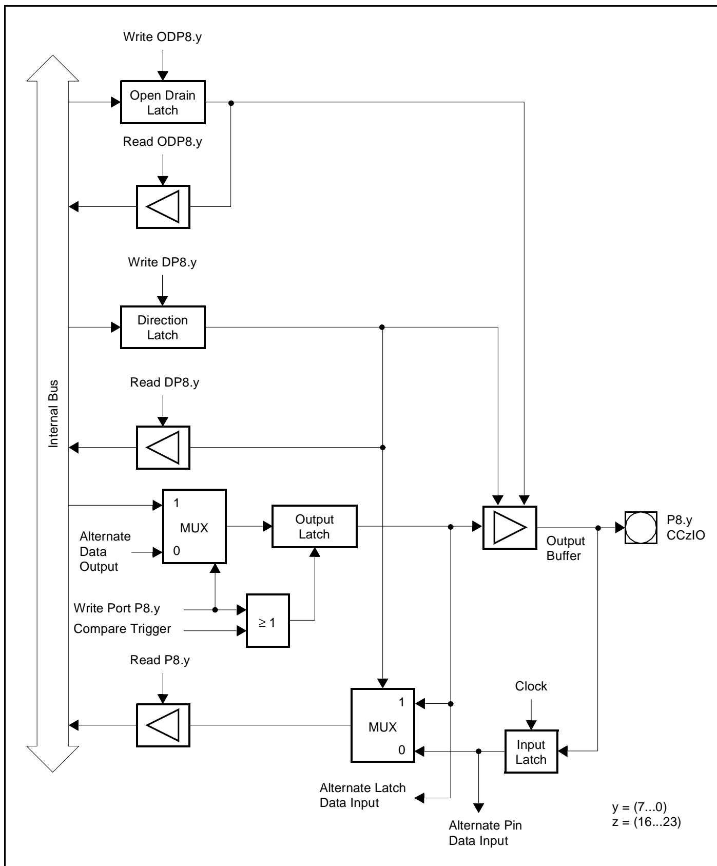
Figure 43 : Block Diagram of Port 8 Pins P8.7...P8.0
