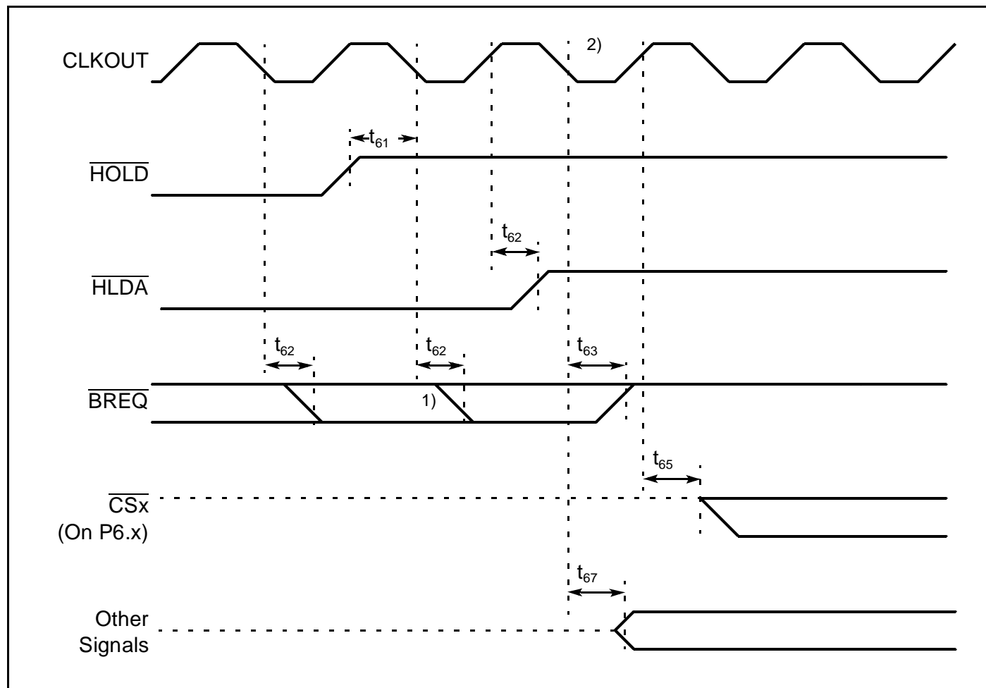
Figure 81 : External Bus Arbitration (Regaining the Bus)
