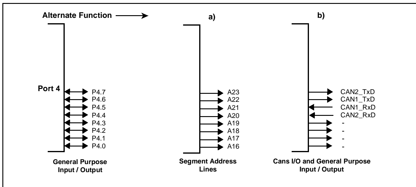
Figure 30 : Port 4 I/O and Alternate Functions
