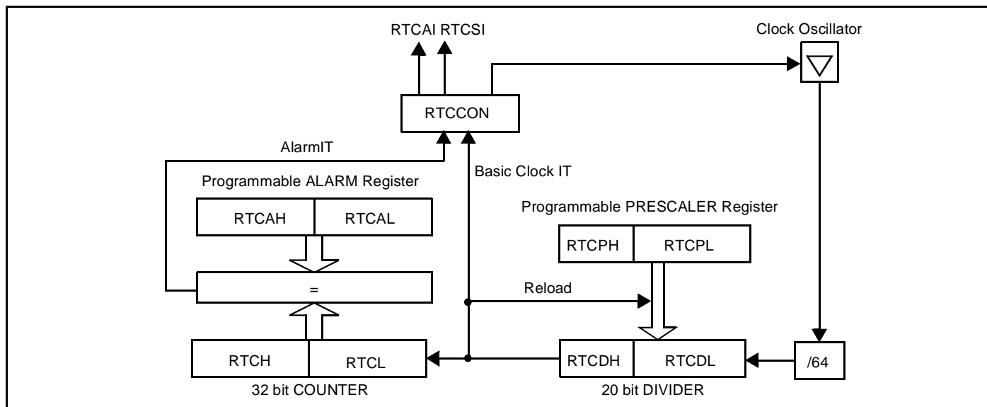
Figure 51 : RTC Block Diagram
