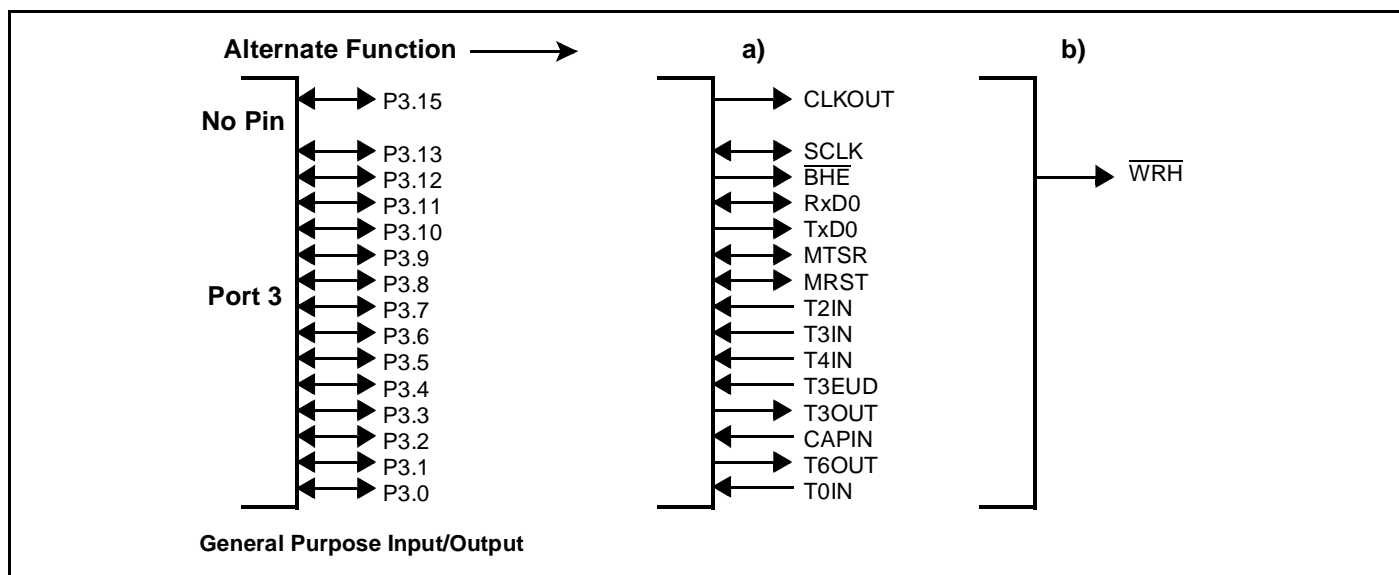
Figure 27 : Port 3 I/O and Alternate Functions
