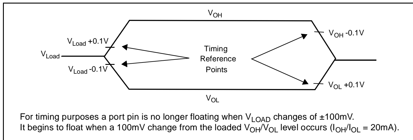
Figure 67 : Float Waveforms
