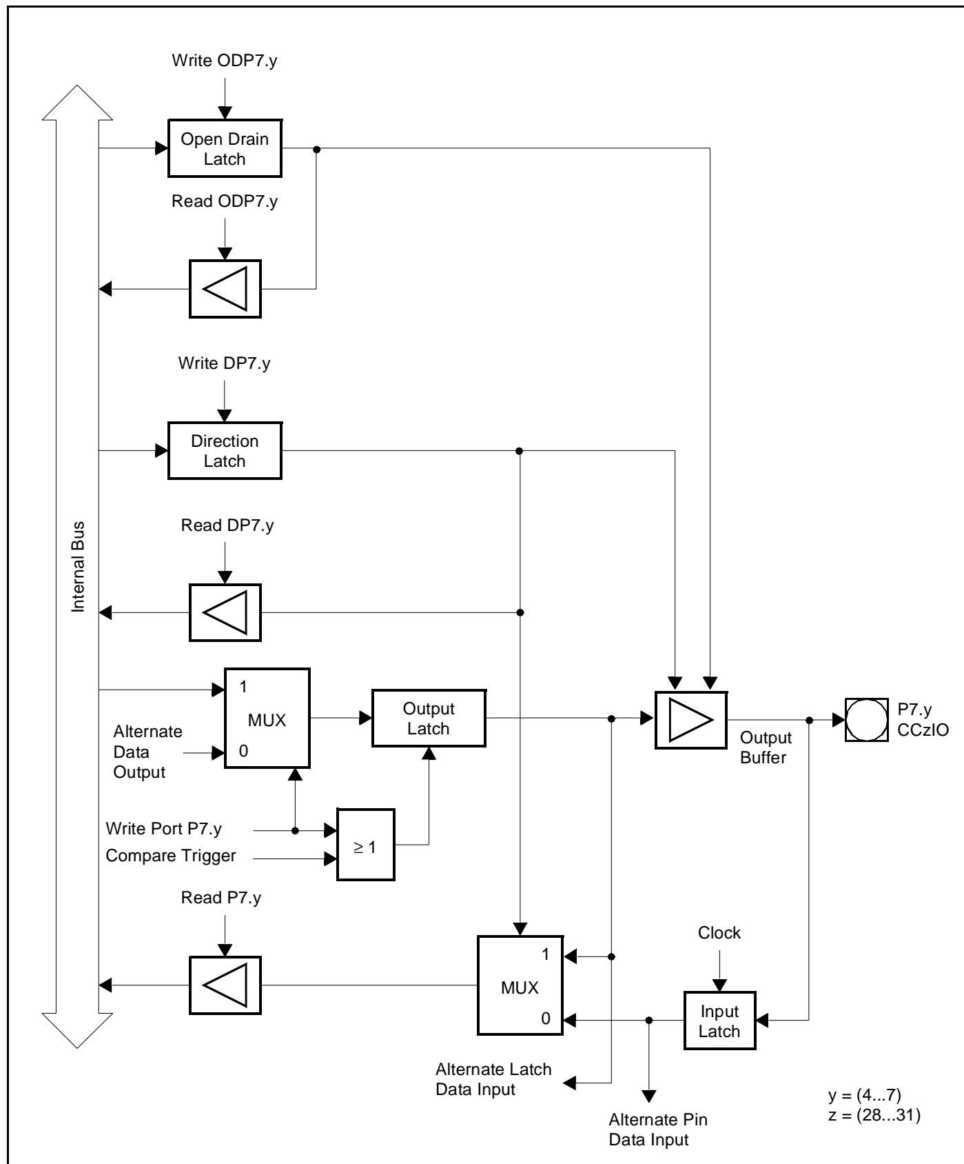
Figure 41 : Block Diagram of Port 7 Pins P7.7...P7.4
