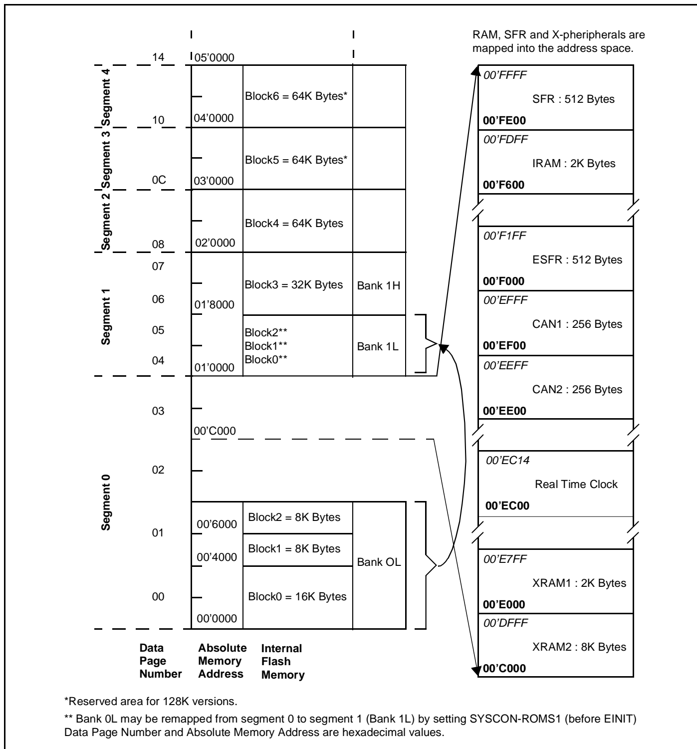
Figure 4 : ST10F269 On-chip Memory Mapping
