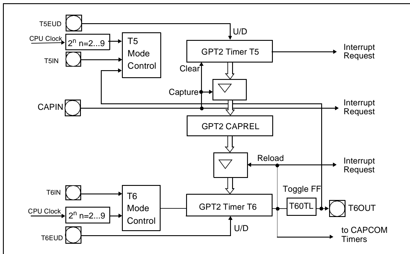
Figure 16 : Block Diagram of GPT2
