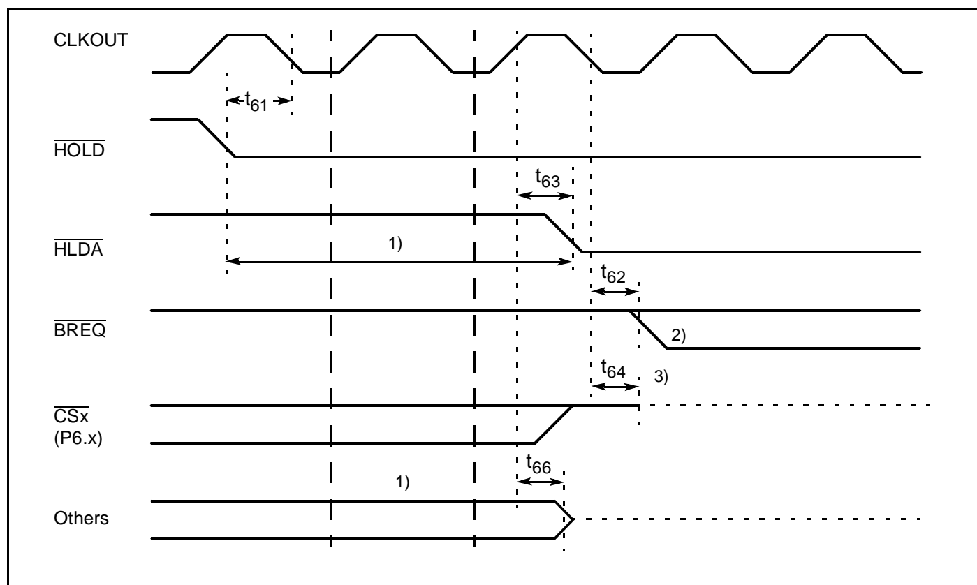
Figure 80 : External Bus Arbitration (Releasing the Bus)
