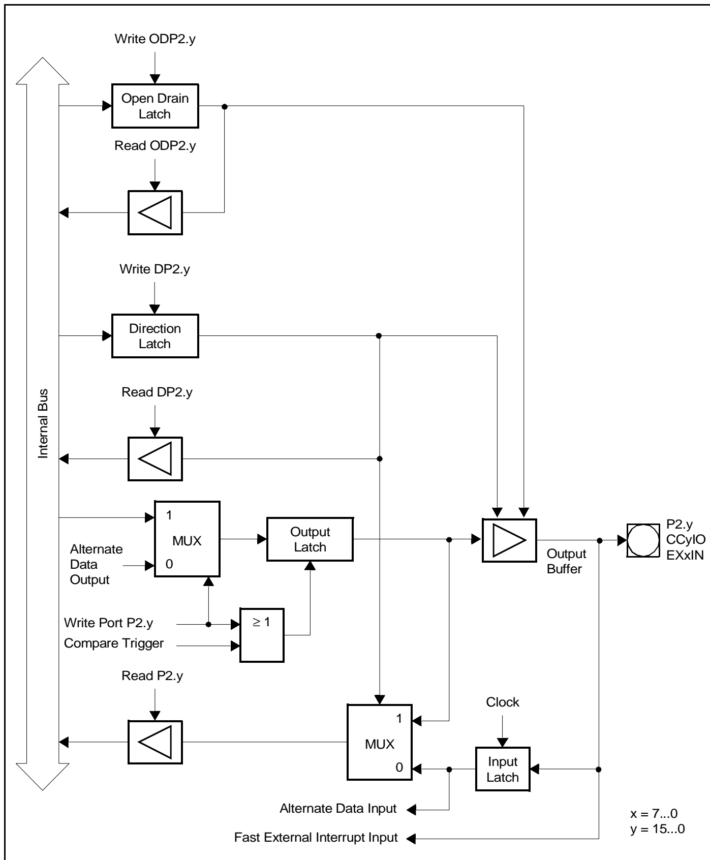
Figure 26 : Block Diagram of a Port 2 Pin
