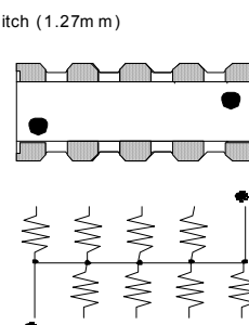
745X102 8 Resistors 10 Terminations
