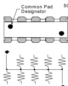
745X101 8 Resistors 10 Terminations
