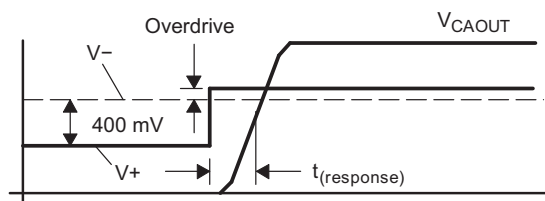
Figure 9. Overdrive Definition
