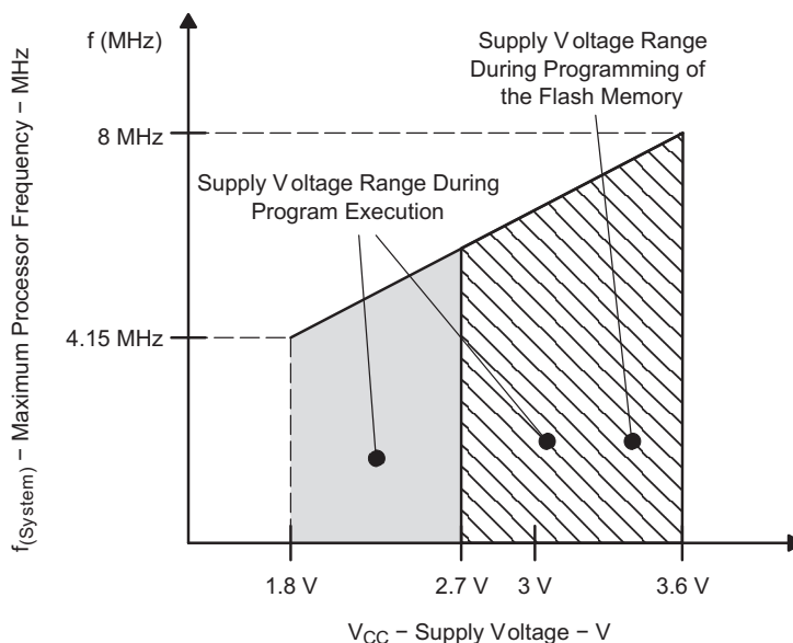
Figure 1. Maximum Frequency vs Supply Voltage
