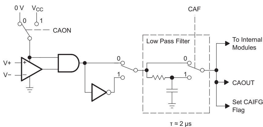
Figure 8. Block Diagram of Comparator_A Module
