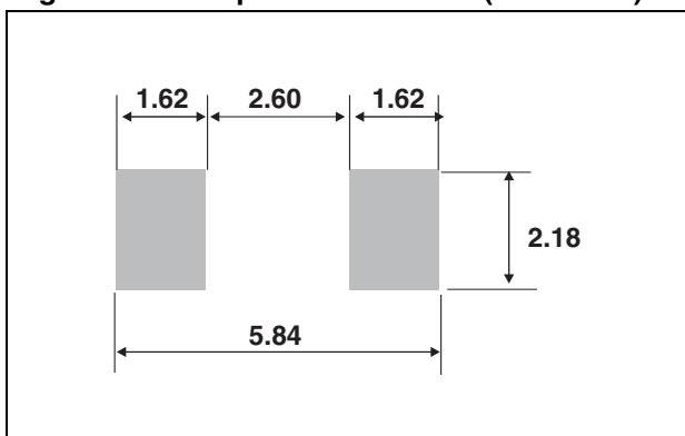
Figure 10. Footprint dimensions (millimeter)
