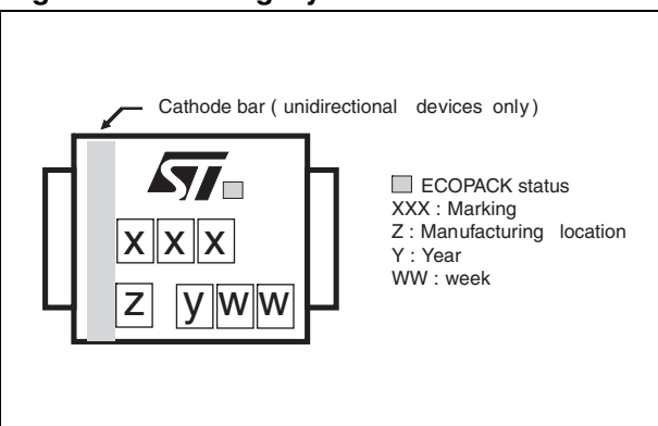
Figure 11. Marking layout
