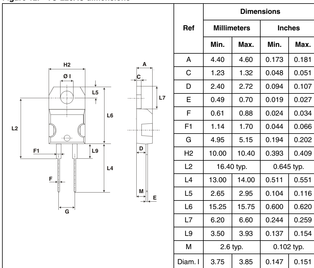
Figure 12. TO-220AC dimensions
