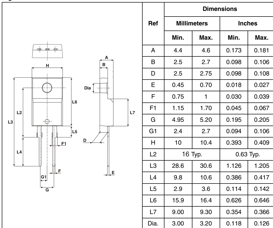
Figure 13. TO-220FPAC dimensions
