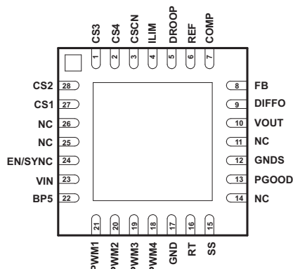
RHD PACKAGE (BOTTOM VIEW)
