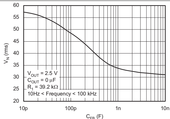
Figure 25. TPS73201 RMS Noise Voltage vs C_{FB}
