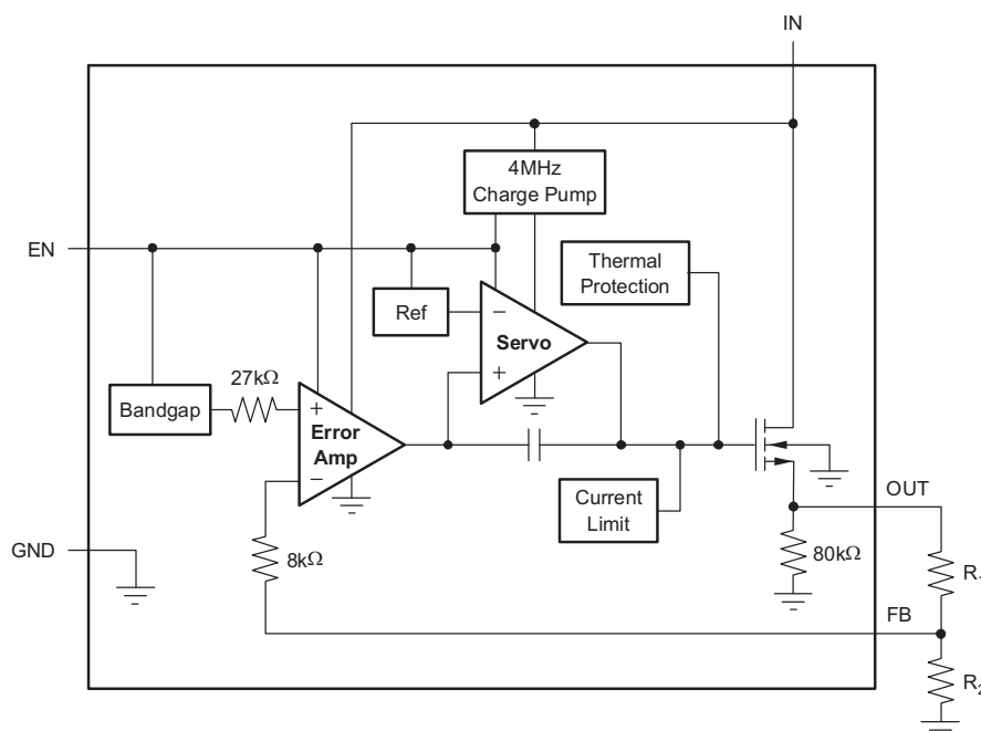
Figure 30. Adjustable-Voltage Version
