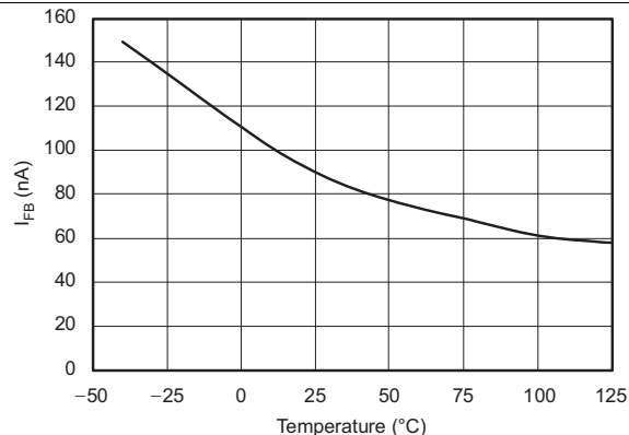
Figure 26. TPS73201 I_{FB} vs Temperature
