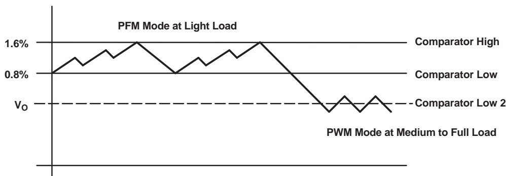
Figure 14. Power-Save Mode Thresholds and Dynamic Voltage Positioning
