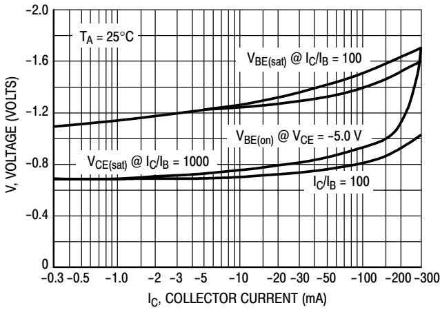
Figure 2. "On" Voltage
