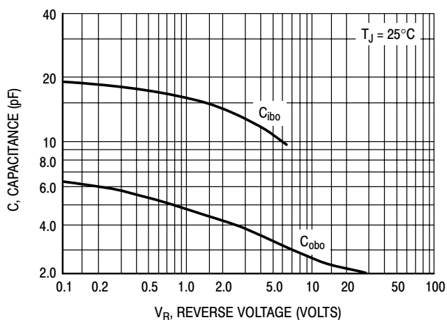
Figure 5. MPS8098/99 Capacitance
