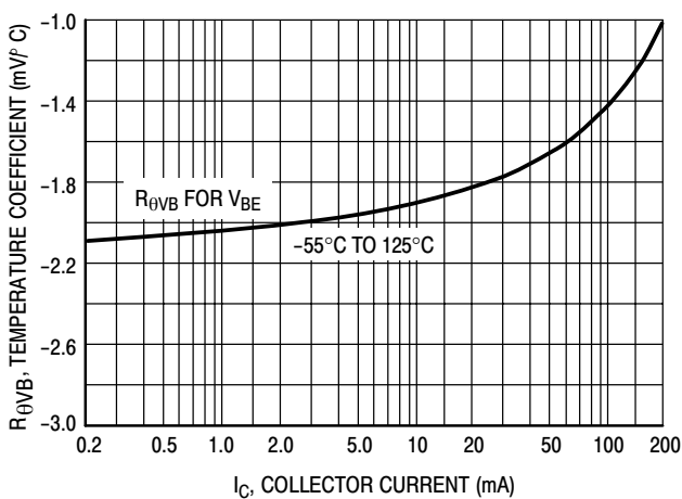
Figure 18. MPS8598/99 Base-Emitter Temperature Coefficient
