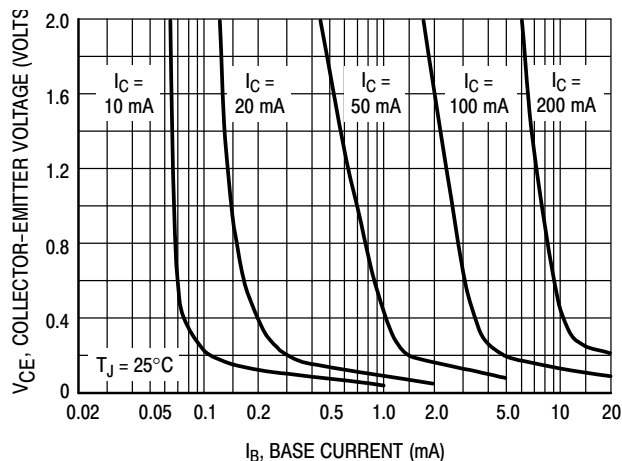
Figure 16. MPS8598/99 Collector Saturation Region
