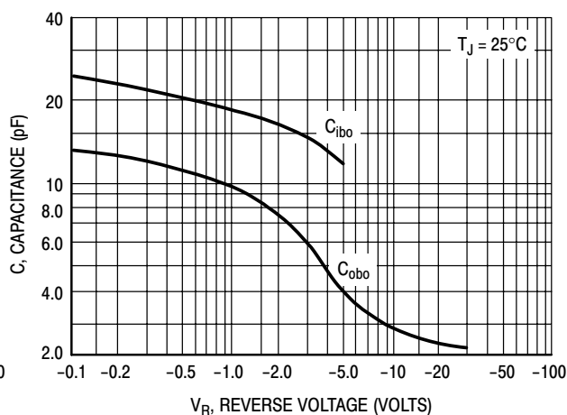
Figure 6. MPS8598/99 Capacitance
