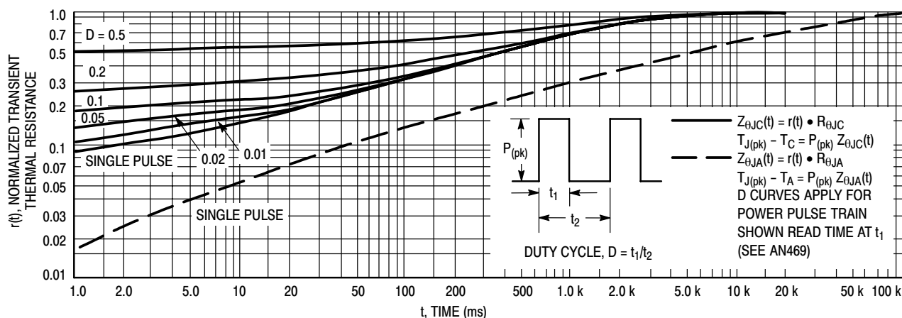
Figure 1. MPS8098, MPS8099, MPS8598 and MPS8599 Thermal Response
