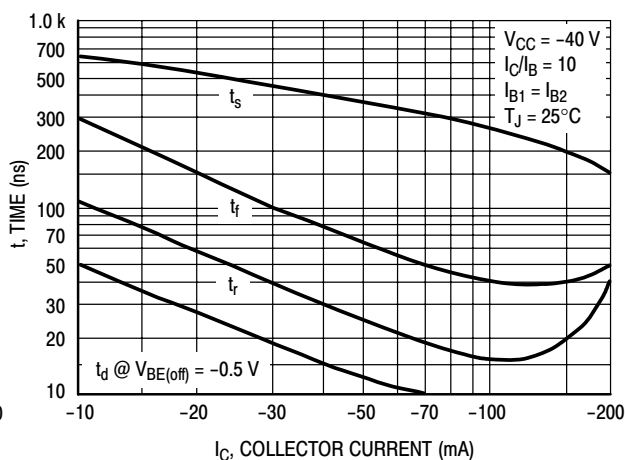
Figure 8. MPS8598/99 Switching Times
