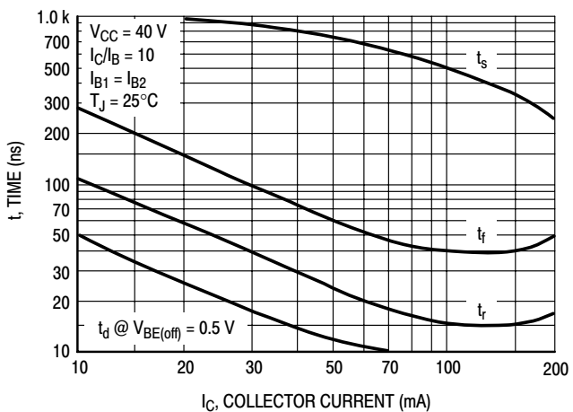
Figure 7. Switching Times
