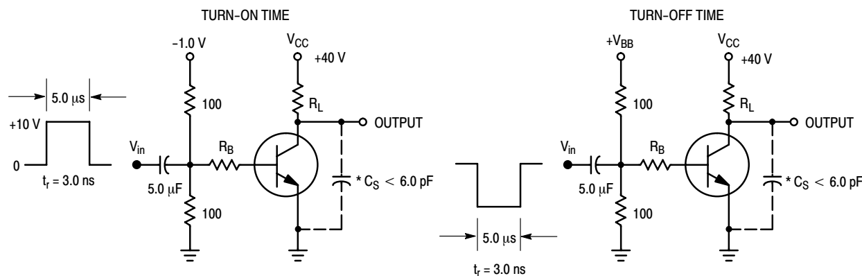
Figure 2. Switching Time Test Circuits
