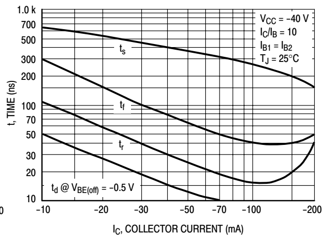
Figure 8. Switching Times
