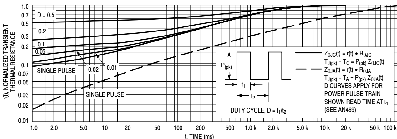
Figure 1. Thermal Response
