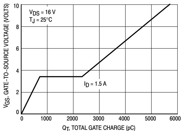
Figure 6. Gate Charge
