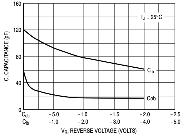
Figure 4. Capacitances
