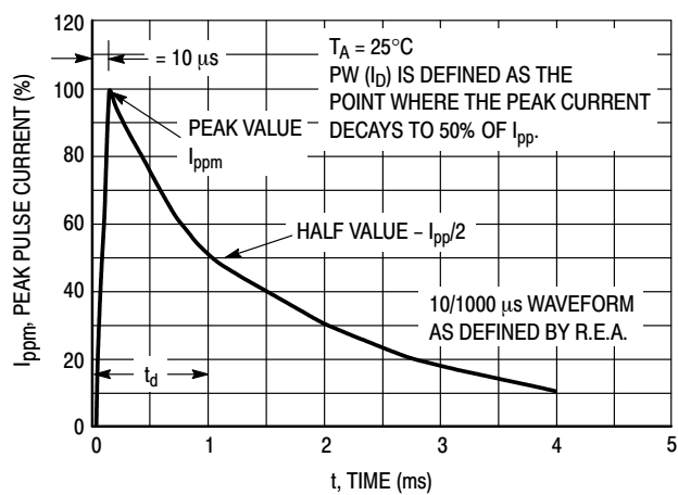
Figure 2. Pulse Waveform
