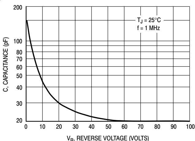
Figure 6. Typical Capacitance
