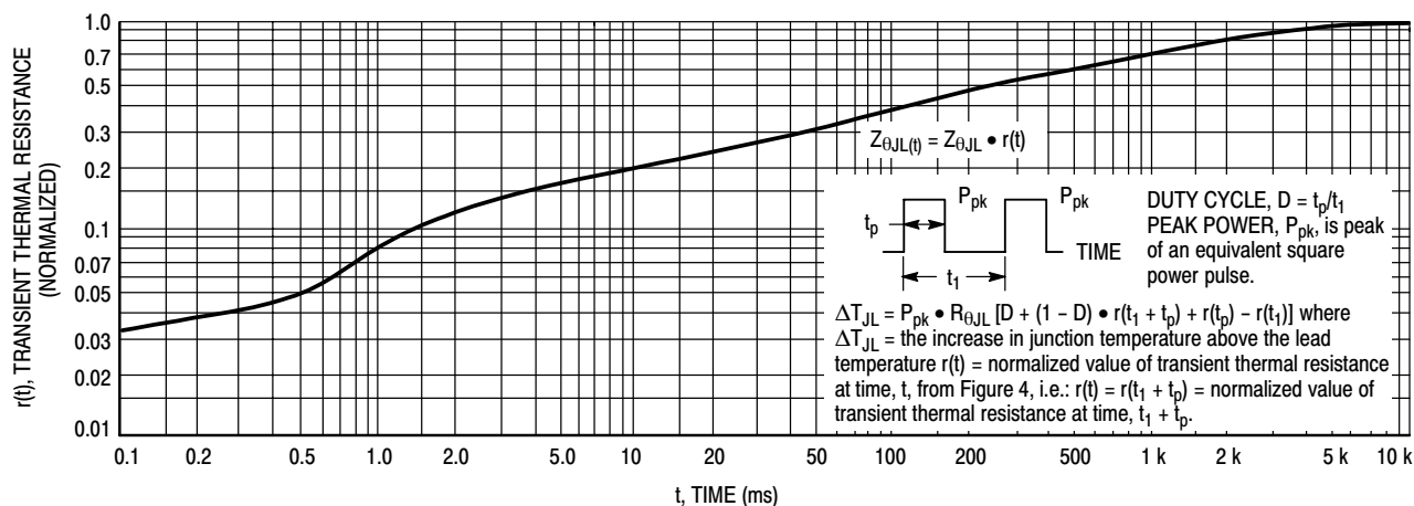
Figure 4. Thermal Response
