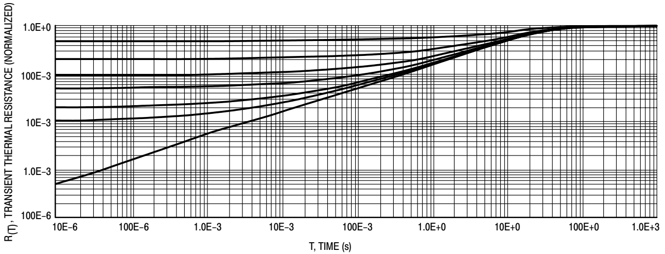
Figure 7. Thermal Response
