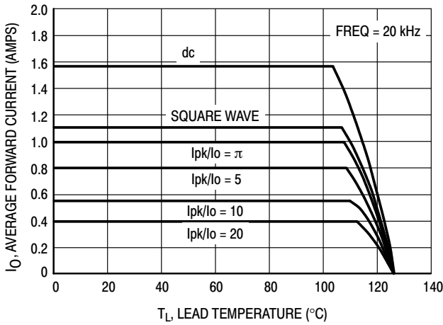
Figure 5. Current Derating
