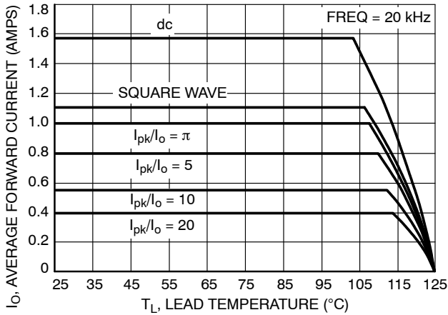
Figure 5. Current Derating
