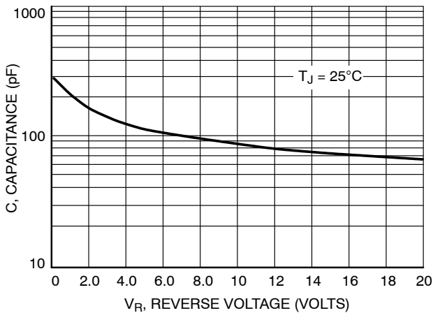
Figure 7. Capacitance
