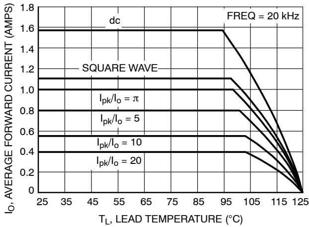
Figure 5. Current Derating
