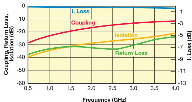
CP0603B****AS
