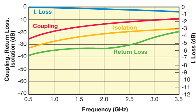
CP0603A****DS
