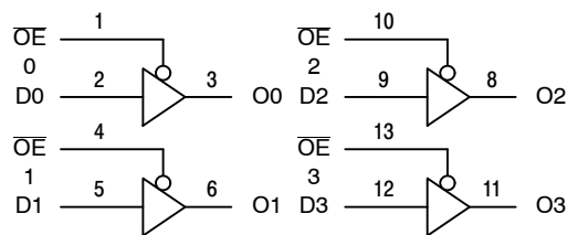
Figure 2. Logic Diagram
