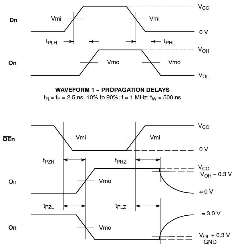
Figure 3. AC Waveforms
