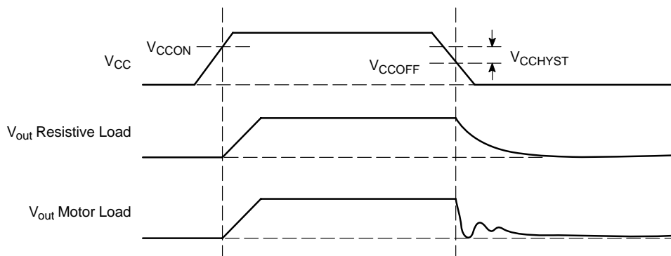
Figure 14. Timing Diagram
