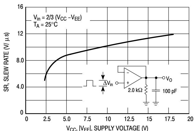
Figure 24. Slew Rate versus Supply Voltage
