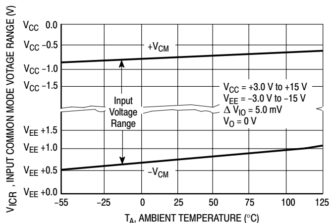
Figure 7. Input Common Mode Voltage Range versus Temperature
