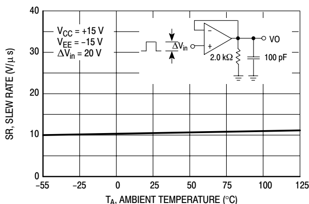
Figure 25. Slew Rate versus Temperature
