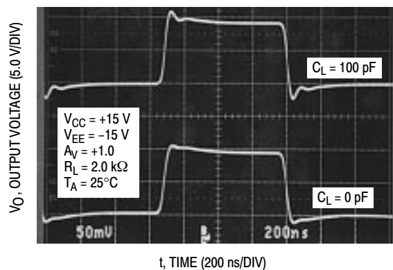
Figure 35. Non-inverting Amplifier Overshoot
