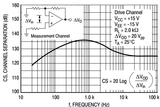
Figure 20. Channel Separation versus Frequency
