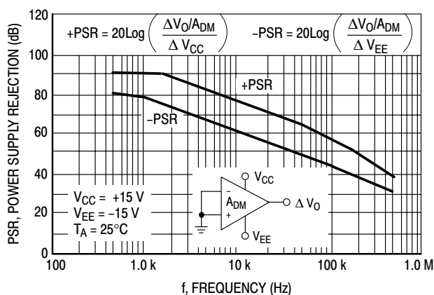
Figure 12. Power Supply Rejection versus Frequency
