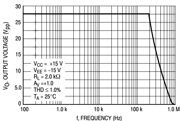
Figure 16. Output Voltage versus Frequency
