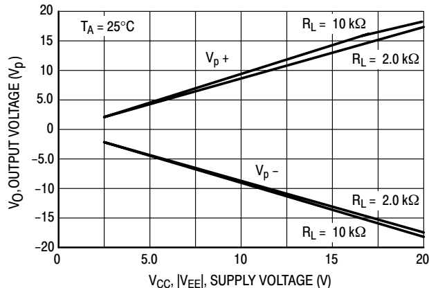
Figure 15. Maximum Output Voltage versus Supply Voltage
