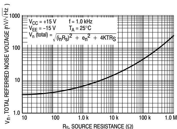
Figure 31. Total Input Referred Noise Voltage versus Source Resistance
