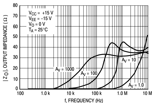
Figure 19. Output Impedance versus Frequency
