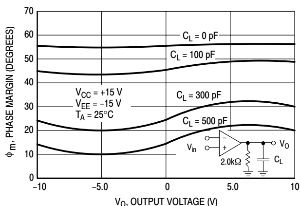
Figure 28. Phase Margin versus Output Voltage
