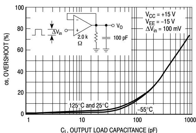
Figure 29. Overshoot versus Output Load Capacitance
