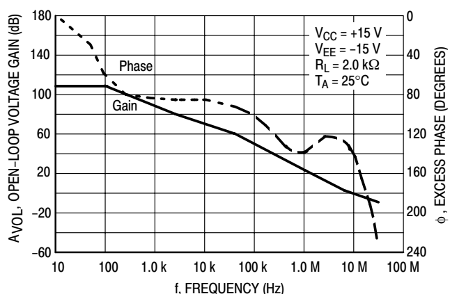
Figure 26. Voltage Gain and Phase versus Frequency
