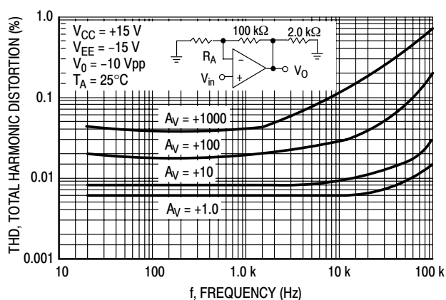
Figure 22. Total Harmonic Distortion versus Frequency
