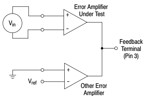
Figure 10. Error-Amplifier Characteristics
