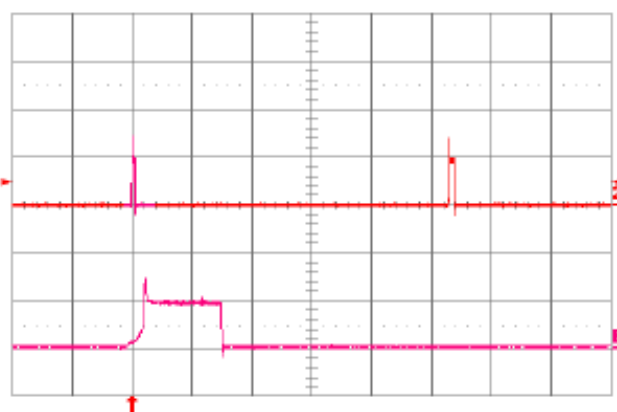
Fig. 1.8V.18: Load current (top trace, 20 A/div., 20 ms/div.) into a 10 m \Omega short circuit during restart, at V_{in} = 48 V. Bottom trace (20 A/div., 1 ms/div.) is an expansion of the on-time portion of the top trace.
