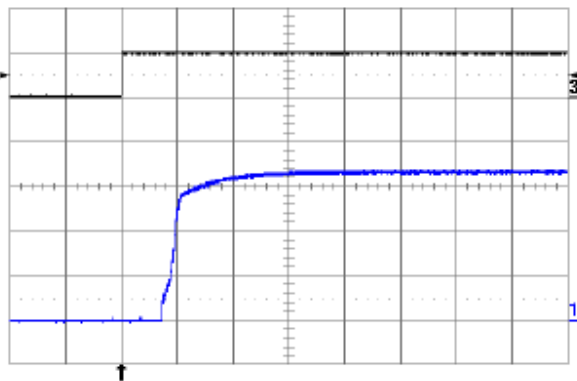
Fig. 3.3V.9: Turn-on transient at full rated load current (resistive) with no output capacitor at V_{in} = 48 V, triggered via ON/OFF pin. Top trace: ON/OFF signal (5 V/div.). Bottom trace: output voltage (1 V/div.). Time scale: 2 ms/div.
