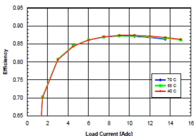
Fig. 2.0V.6: Efficiency vs. load current and ambient for SQ48T/S15020 converter mounted vertically with air flowing from pin 3 to pin 1 at a rate of 200 LFM (1.0 m/s).
