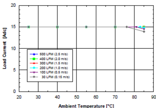
Fig. 1.5V.4: Available load current vs. ambient air temperature and airflow rates for SQ48S15015 converter mounted horizontally with V_{in} = 48 V, air flowing from pin 3 to pin 1, and maximum FET temperature \leq 120 °C.
