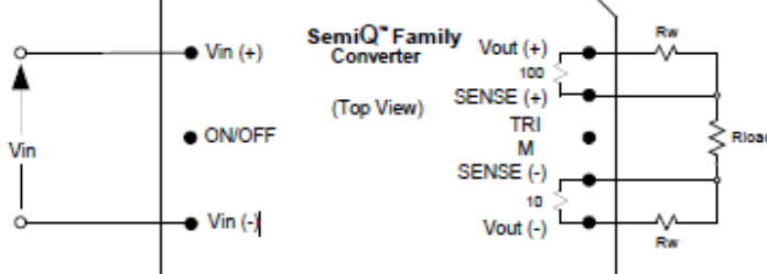
Fig. B: Remote sense circuit configuration
