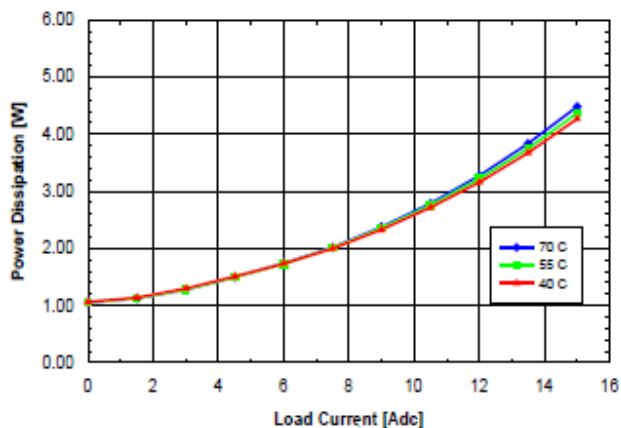
Fig. 1.5V.8: Power dissipation vs. load current and ambient temperature for SQ48T/S15015 converter mounted vertically with V_{in} = 48\text{ V} and air flowing from pin 3 to pin 1 at a rate of 200 LFM (1.0 m/s).
