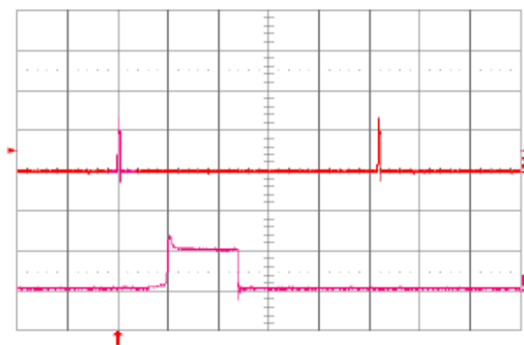
Fig. 1.2V.18: Load current (top trace, 20 A/div., 20 ms/div.) into a 10 m \Omega short circuit during restart, at V_{in} = 48 V. Bottom trace (20 A/div., 1 ms/div.) is an expansion of the on-time portion of the top trace.
