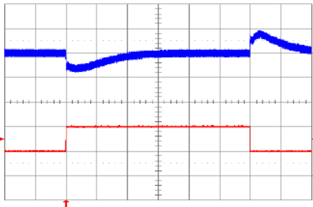
Fig. 6.0V.12: Output voltage response to load current step-change (2 A – 4 A – 2 A) at V_{in} = 48V . Top trace: output voltage (100 mV/div.). Bottom trace: load current (2 A/div.). Current slew rate: 5A/ \mu s. C_o = 450\mu F tantalum + 1\mu F ceramic. Time scale: 0.2ms/div.
