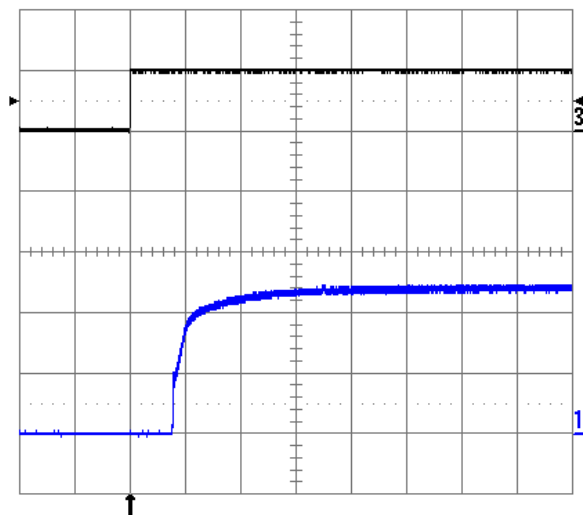
Fig. 1.2V.9: Turn-on transient at full rated load current (resistive) with no output capacitor at V_{in} = 48\text{ V} , triggered via ON/OFF pin. Top trace: ON/OFF signal (5 V/div.). Bottom trace: output voltage (0.5 V/div.). Time scale: 2 ms/div.
