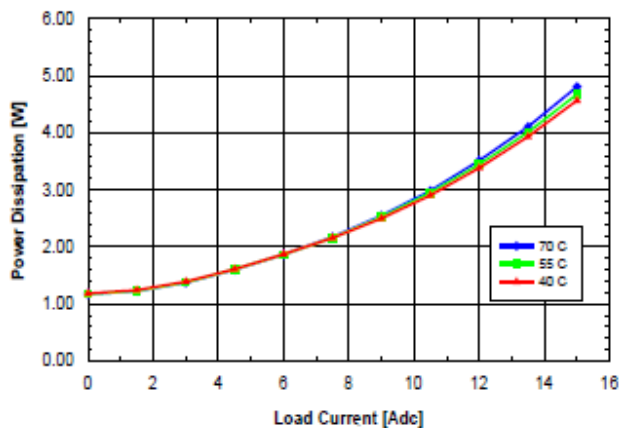
Fig. 1.8V.8: Power dissipation vs. load current and ambient temperature for SQ48T/S15018 converter mounted vertically with air flowing from pin 3 to pin 1 at a rate of 200 LFM (1.0 m/s).
