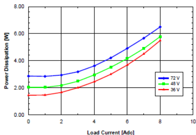
Fig. 6.0V.7: Power dissipation vs. load current and input voltage for SQ48T/S08060 converter mounted vertically with air flowing from pin 3 to pin 1 at a rate of 300 LFM (1.5 m/s) and T a = 25°C.
