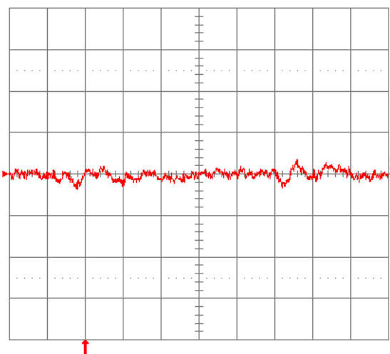
Fig. 1.2V.16: Input reflected ripple current, i_s (10 mA/div.), measured through 10 \mu H at the source at full rated load current and V_{in} = 48 V. Refer to Fig. 1.2V.14 for test setup. Time scale: 1 \mu s/div.
