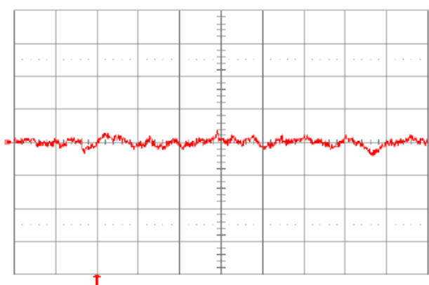
Fig. 5.0V.16: Input reflected ripple current, i_s (10 mA/div.), measured through 10 \mu\text{H} at the source at full rated load current and V_{in} = 48\text{V} . Refer to Fig. 5.0V.14 for test setup. Time scale: 1 \mu\text{s}/\text{div} .
