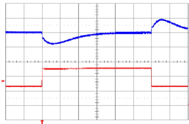
Fig. 5.0V.12: Output voltage response to load current step-change (2.5A – 5A – 2.5A) at V_{in} = 48V . Top trace: output voltage (200 mV/div.). Bottom trace: load current (2A/div.). Current slew rate: 5A/ \mu s . C_o = 450\mu F tantalum + 1 \mu F ceramic. Time scale: 0.2 ms/div.
