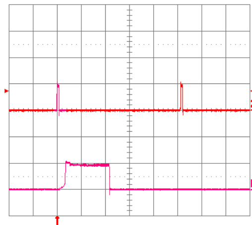
Fig. 3.3V.18: Load current (top trace, 20 A/div., 20 ms/div.) into a 10 mΩ short circuit during restart, at V_{in} = 48\text{ V} . Bottom trace (20 A/div., 1 ms/div.) is an expansion of the on-time portion of the top trace.
