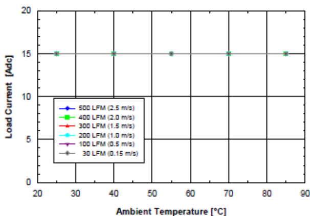
Fig. 1.0V.4: Available load current vs. ambient air temperature and airflow rates for SQ48S15010 converter mounted horizontally with V_{in} = 48 V, air flowing from pin 3 to pin 1, and maximum FET temperature \leq 120 °C.
