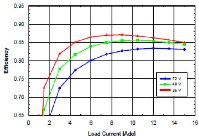
Fig. 1.5V.5: Efficiency vs. load current and input voltage for SQ48T/S15015 converter mounted vertically with air flowing from pin 3 to pin 1 at a rate of 300 LFM (1.5 m/s) and T_a = 25 °C.
