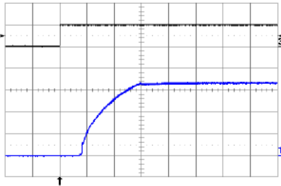
Fig. 3.3V.10: Turn-on transient at full rated load current (resistive) plus 10,000 \mu F at V_{in} = 48 V, triggered via ON/OFF pin. Top trace: ON/OFF signal (5 V/div.). Bottom trace: output voltage (1 V/div.). Time scale: 2 ms/div.
