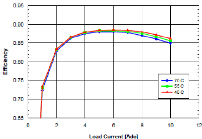
Fig. 5.0V.6: Efficiency vs. load current and ambient temperature for SQ48T/S10050 converter mounted vertically with V_{in} = 48\text{V} and air flowing from pin 3 to pin 1 at a rate of 200 LFM (1.0 m/s).
