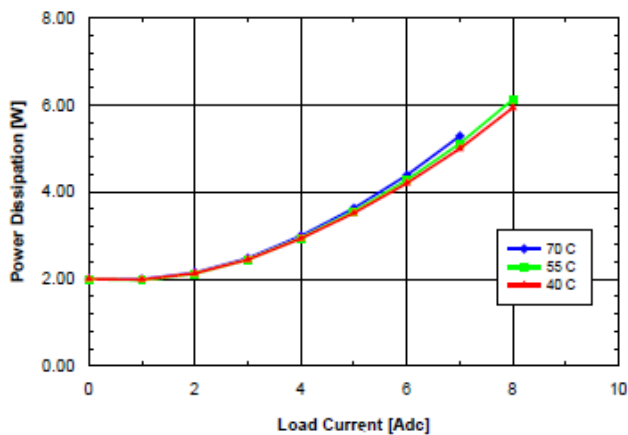
Fig. 6.0V.8: Power dissipation vs. load current and ambient temperature for SQ48T/S08060 converter mounted vertically with V in = 48V and air flowing from pin 3 to pin 1 at a rate of 200 LFM (1.0 m/s).
