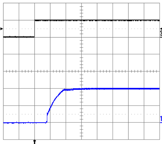
Fig. 2.0V.9: Turn-on transient at full rated load current (resistive) plus 10,000 \mu\text{F} at V_{in} = 48\text{ V} , triggered via ON/OFF pin. Top trace: ON/OFF signal (5 V/div.). Bottom trace: output voltage (1 V/div.). Time scale: 2 ms/div.
