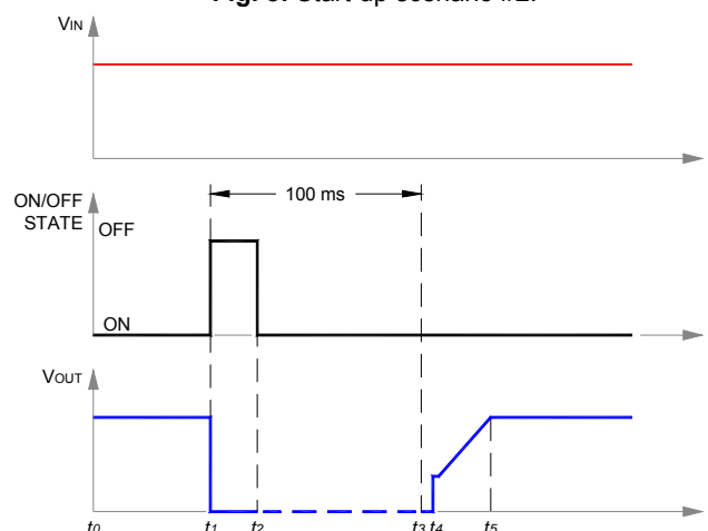
Fig. 9: Start-up scenario #3.
