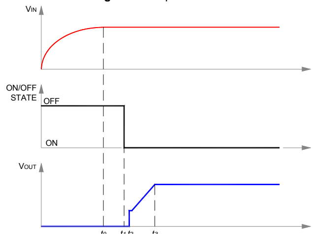
Fig. 8: Start-up scenario #2.
