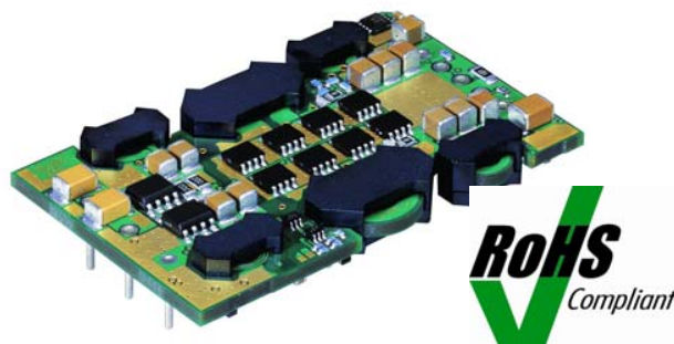
Q48T30015 Converter
