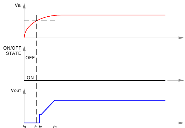
Fig. 7: Start-up scenario #1.
