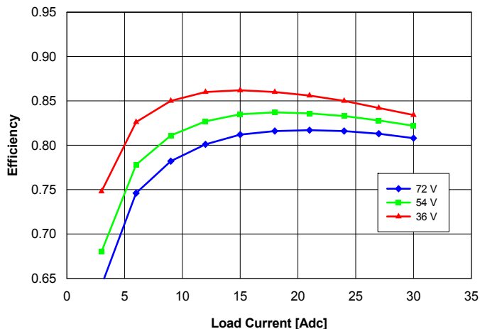
Fig. 14: Efficiency vs. load current and input voltage for converter mounted vertically with air flowing from pin 3 to pin 1 at a rate of 300 LFM (1.5 m/s) and T_a = 25^\circ\text{C} .
