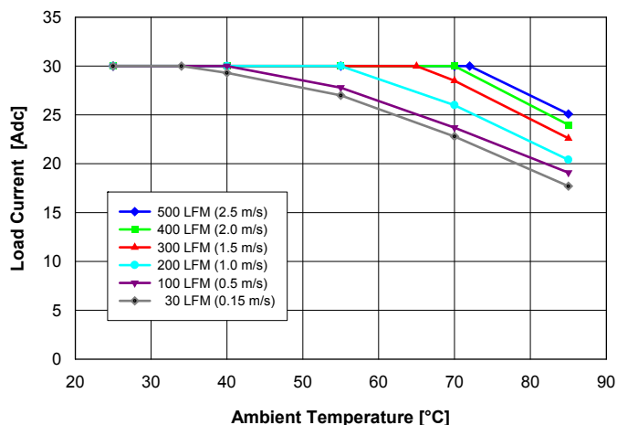
Fig. 10: Available load current vs. ambient air temperature and airflow rates for converter mounted vertically with V_{in} = 54 V, air flowing from pin 3 to pin 1 and maximum FET temperature \leq 105^{\circ}\text{C} .
