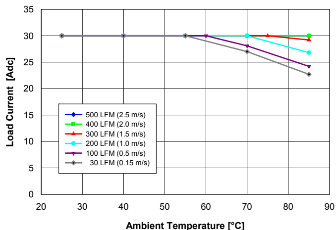
Fig. 9: Available load current vs. ambient air temperature and airflow rates for converter mounted vertically with V_{in} = 54 V, air flowing from pin 3 to pin 1 and maximum FET temperature \leq 120^{\circ}\text{C} .
