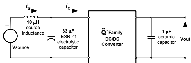
Fig. 22: Test setup for measuring input reflected ripple currents, i_c and i_s .
