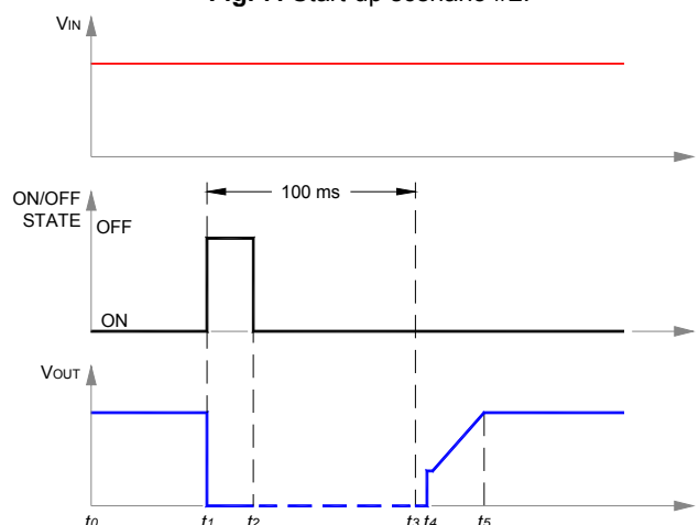
Fig. 8: Start-up scenario #3.
