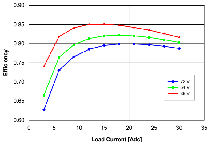
Fig. 13: Efficiency vs. load current and input voltage for converter mounted vertically with air flowing from pin 3 to pin 1 at a rate of 300 LFM (1.5 m/s) and T_a = 25^\circ\text{C} .
