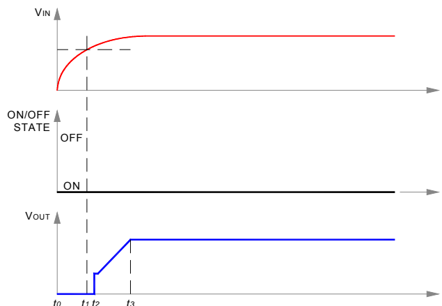
Fig. 6: Start-up scenario #1.
