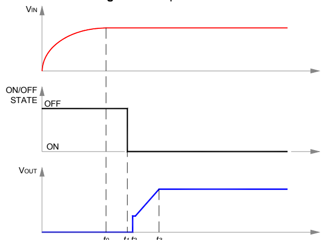
Fig. 7: Start-up scenario #2.
