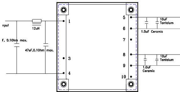
Figure 5. Typical Application of HHD Series
