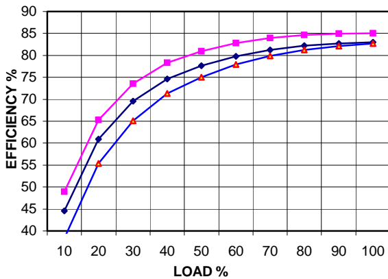
Figure 3. HHD20ZGB Efficiency vs. Output Load
