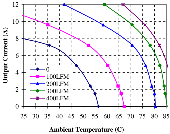
Figure 6. HHD20ZGE Derating Curves
