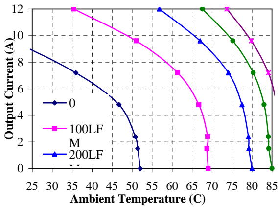
Figure 8. HD20ZGB Derating Curves
