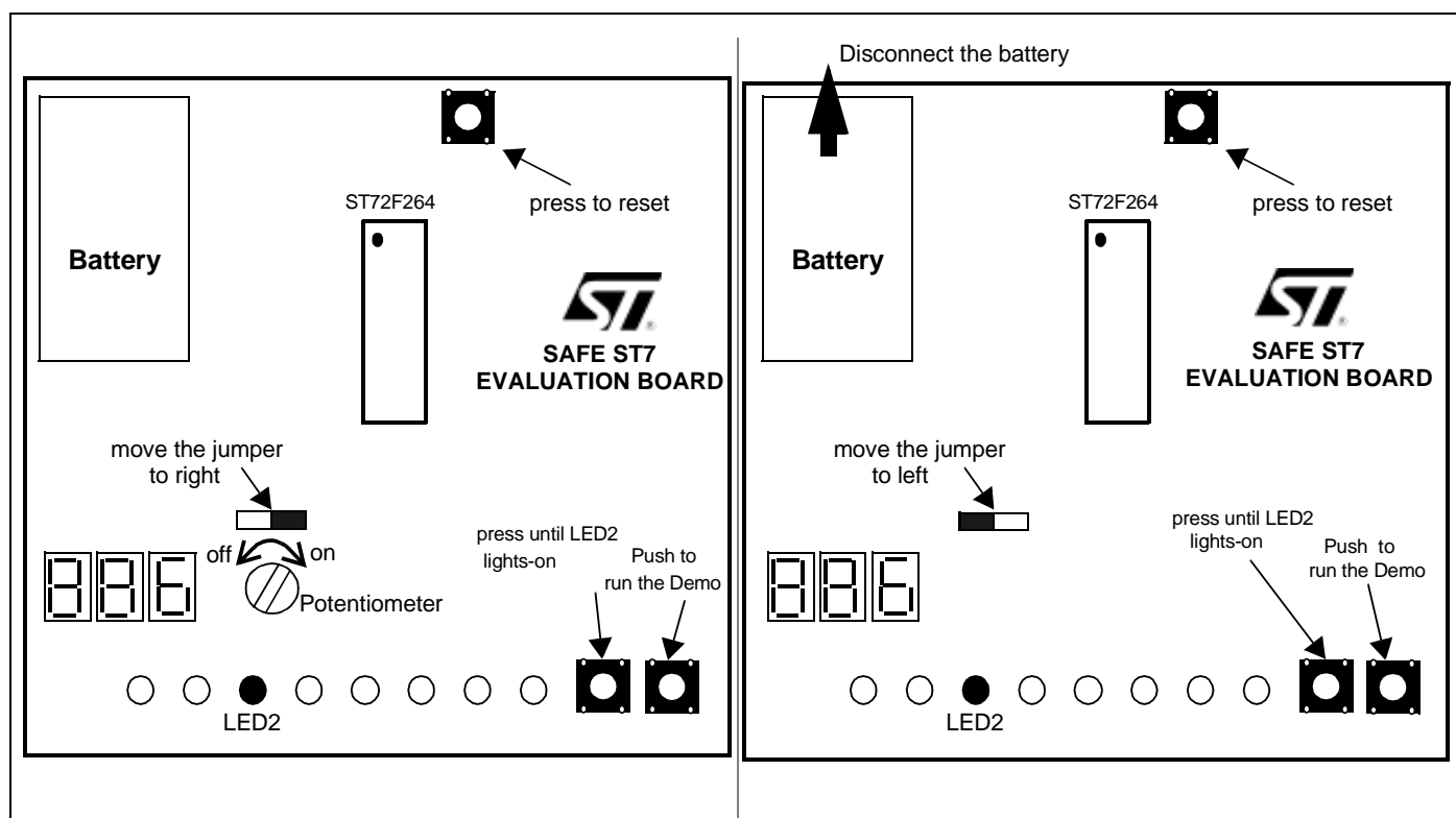
Figure 12. AVD Demo Overview
