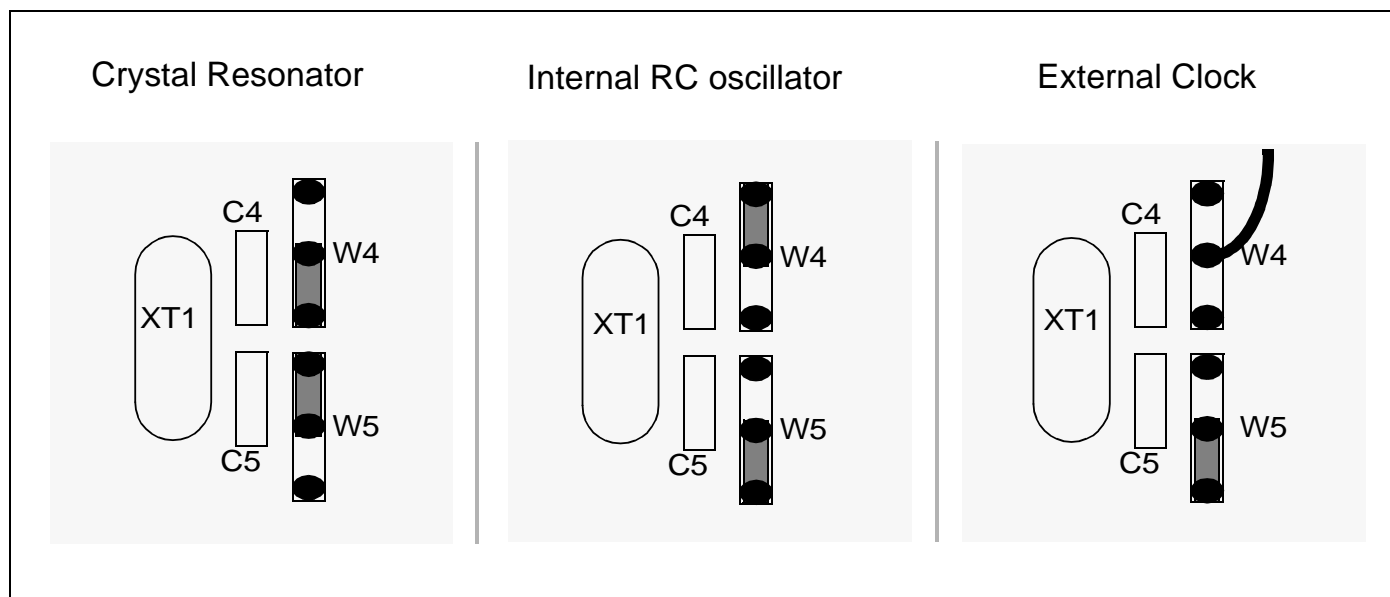
Figure 3. How to Change the Oscillator Frequency Source
