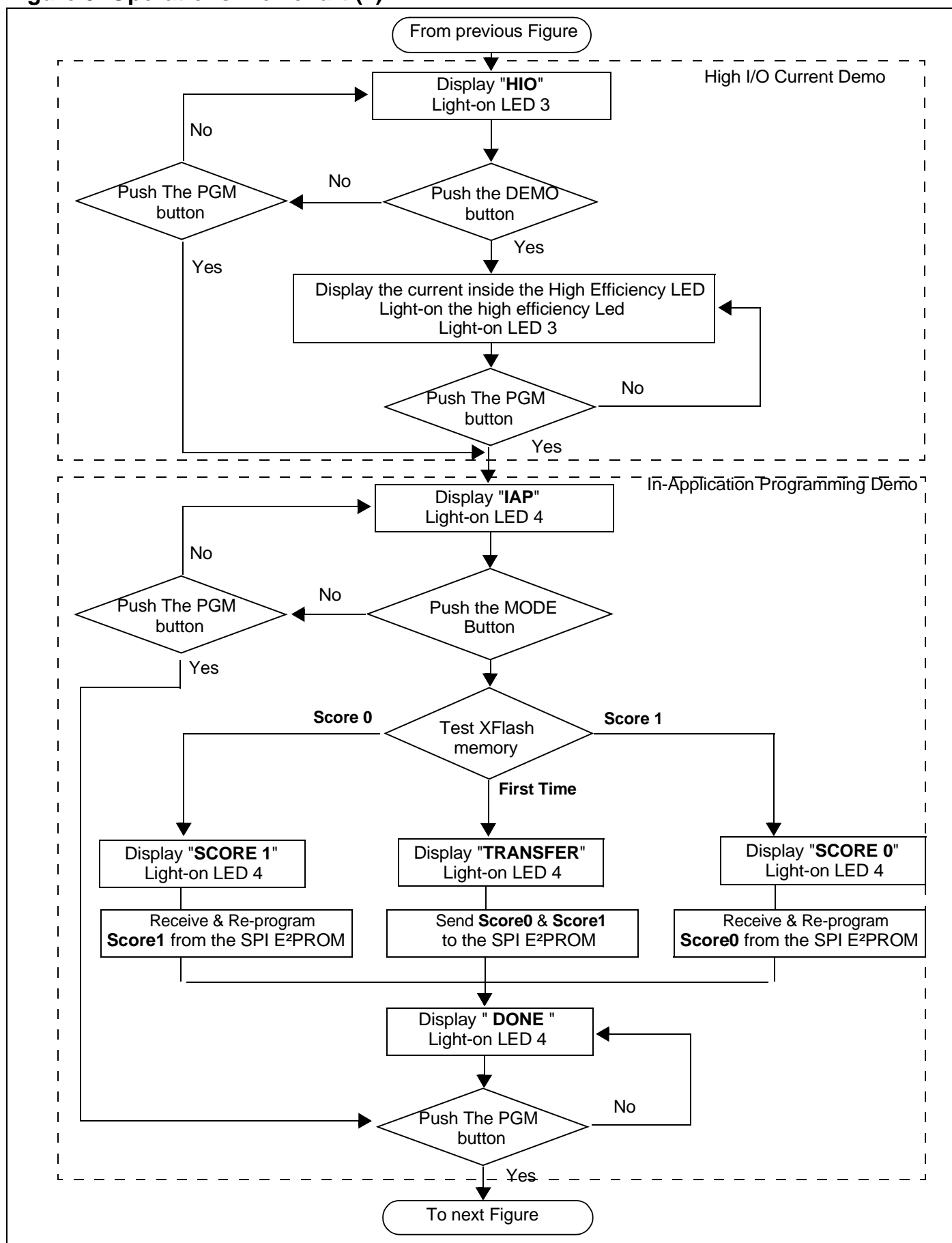
Figure 9. Operations Flowchart (2)
