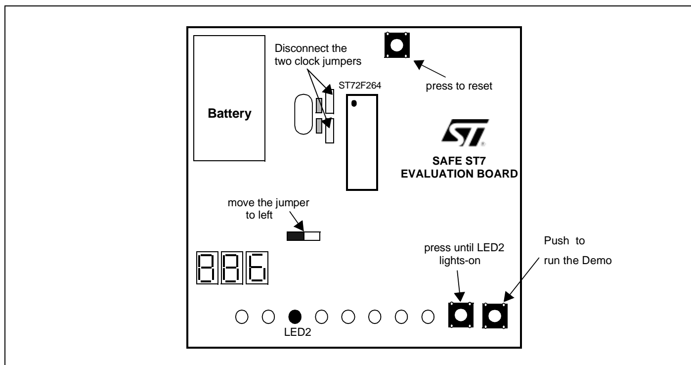
Figure 13. CSS Demo Overview
