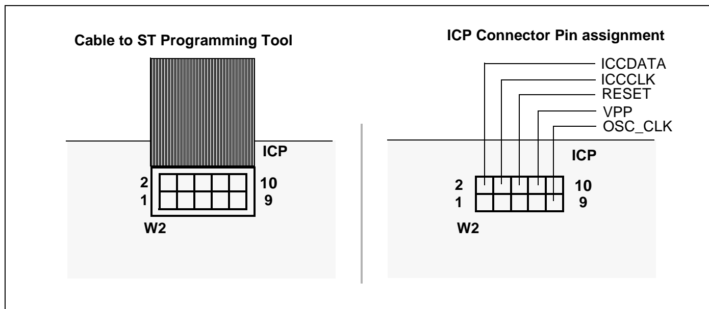
Figure 4. How to use the ICP Connector
