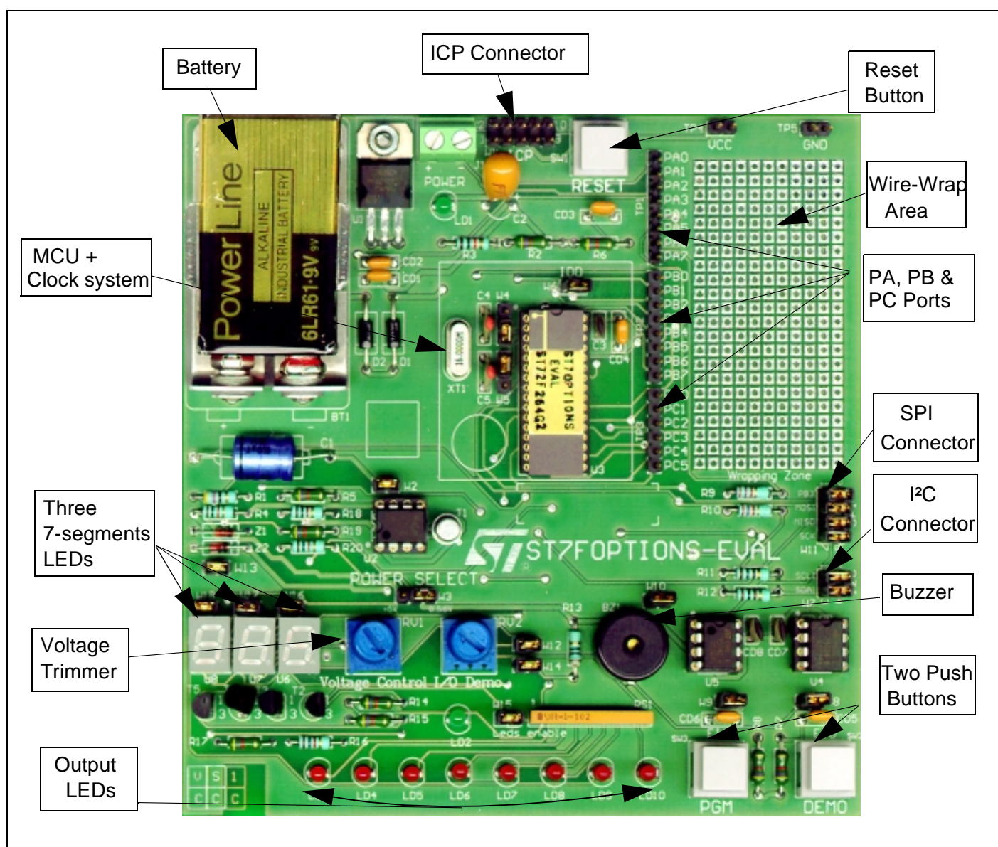
Figure 1. Safe ST7 Evaluation Board layout
