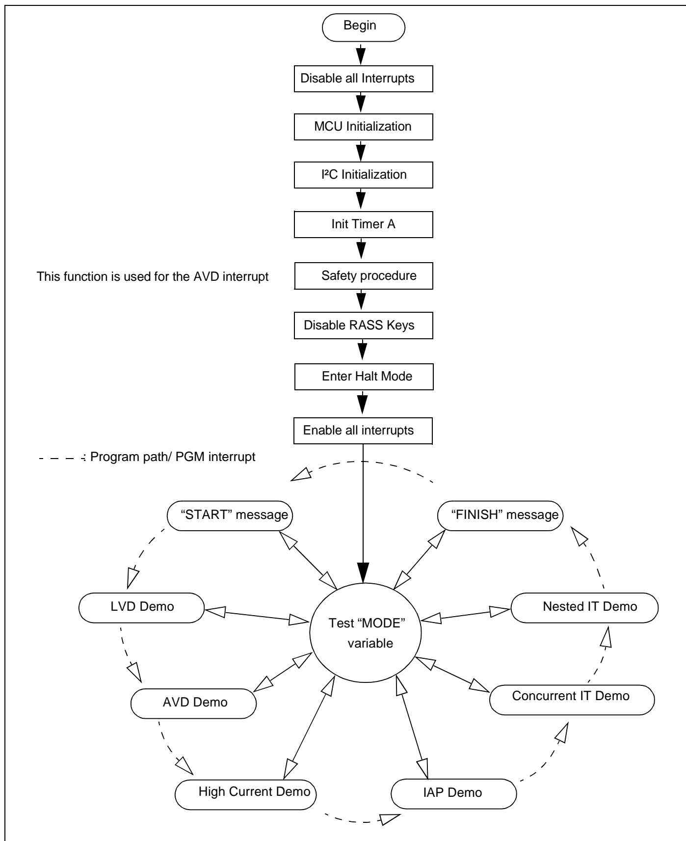
Figure 7. Main program flowchart
