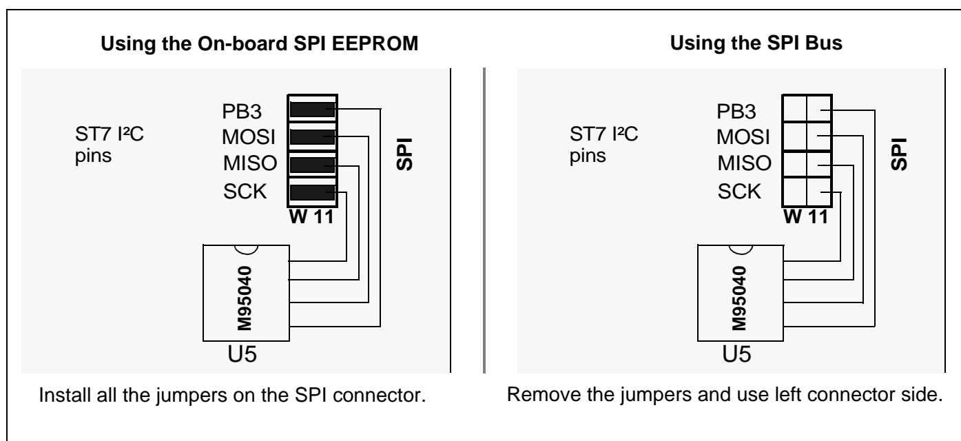
Figure 6. How to use the SPI Connection
