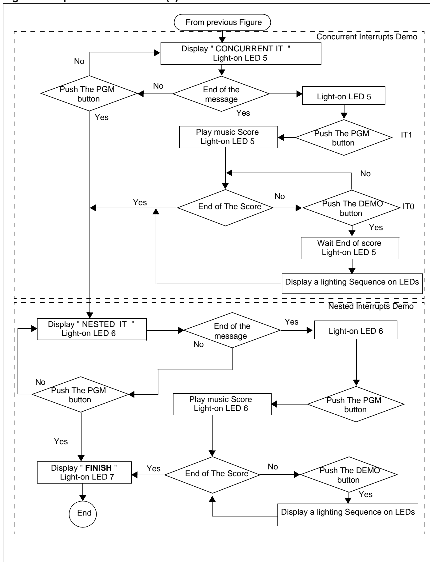
Figure 10. Operations Flowchart (3)
