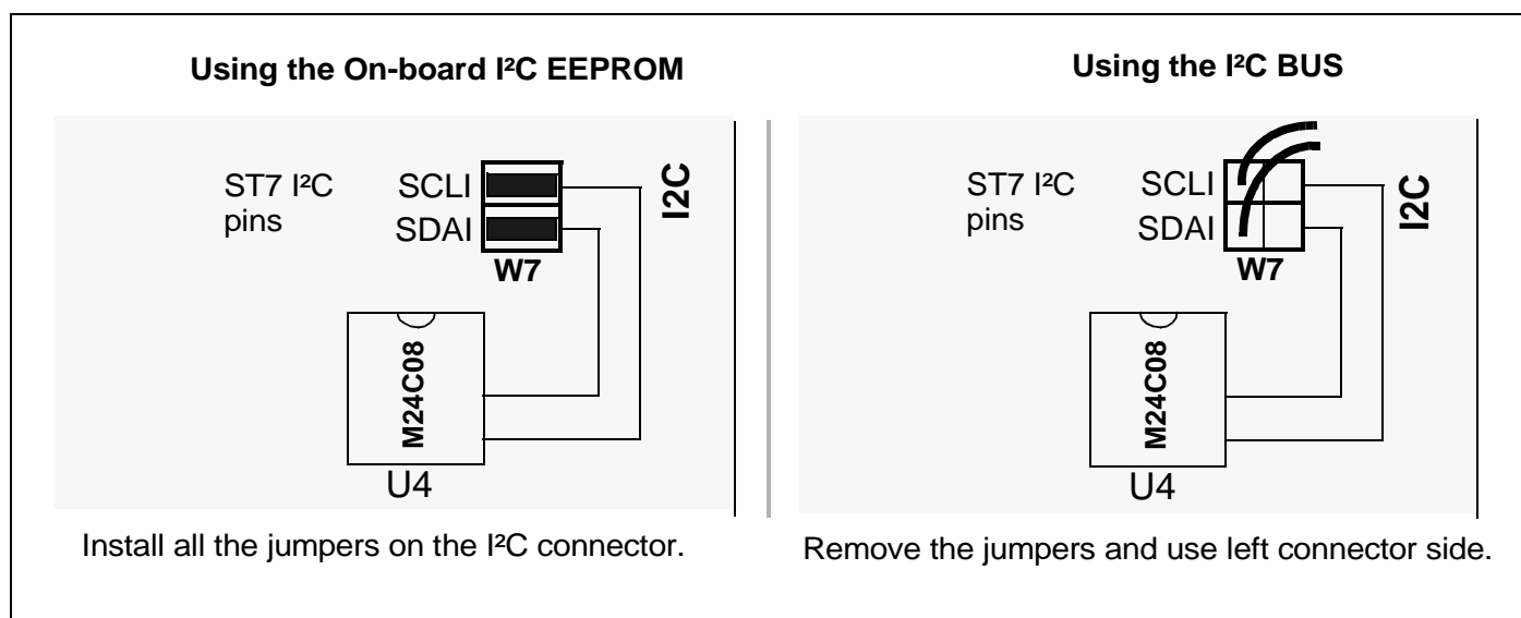
Figure 5. How to use the I 2 C Connection
