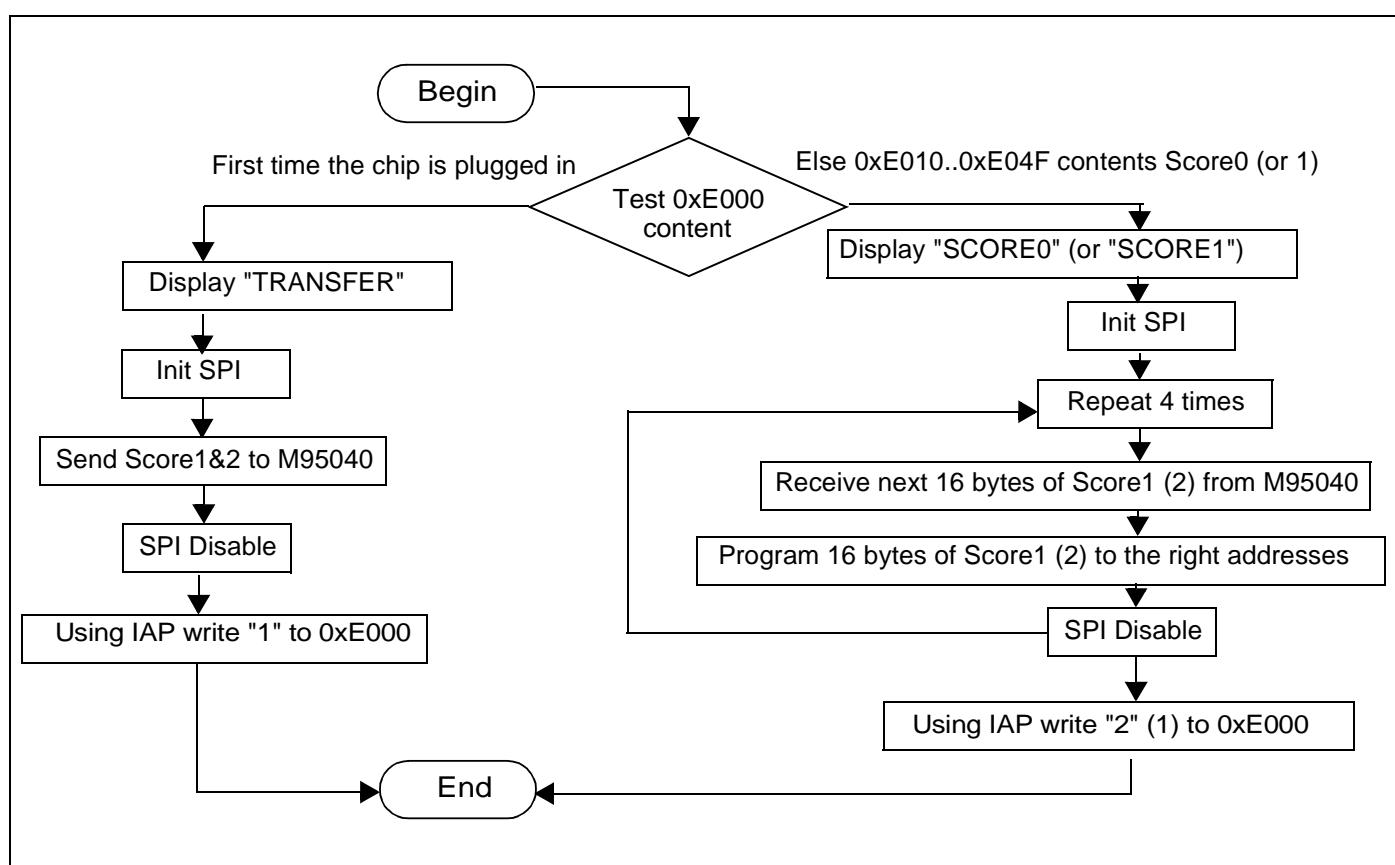
Figure 16. IAP Demo flowchart
